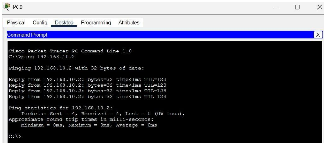
Fig. (2.3) Testing using ping command
