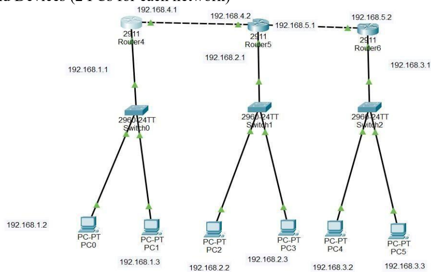
(8.1) Configuration for OSPF
