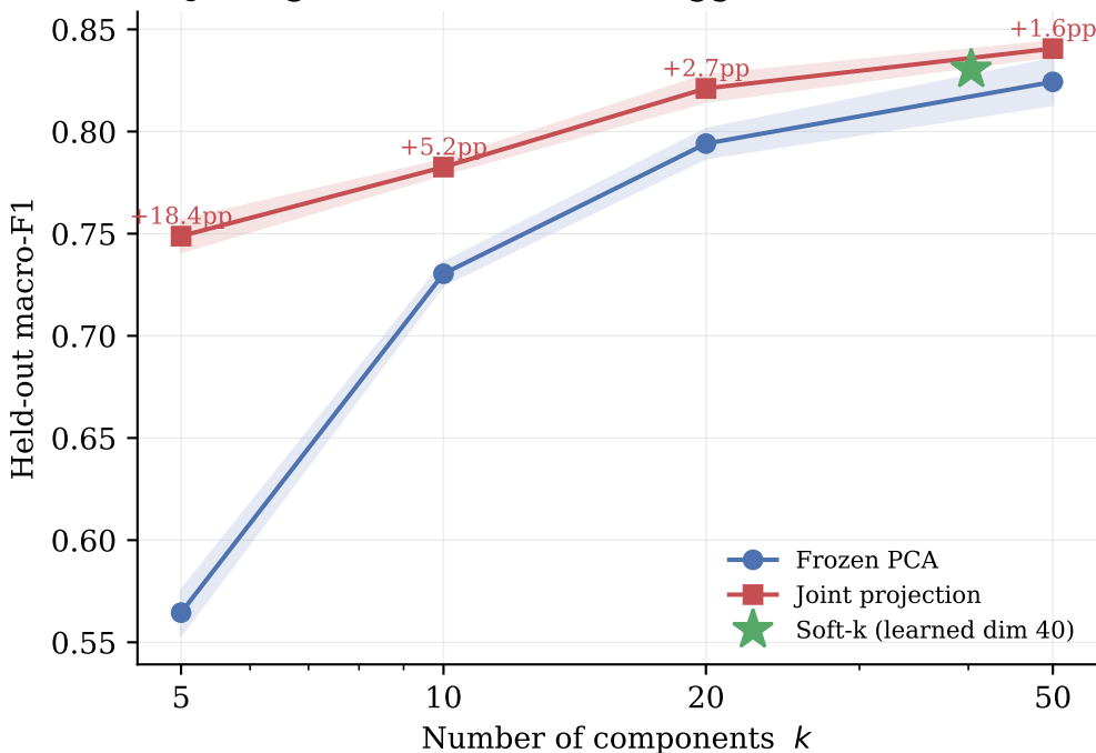
Joint gain concentrates at aggressive reduction
