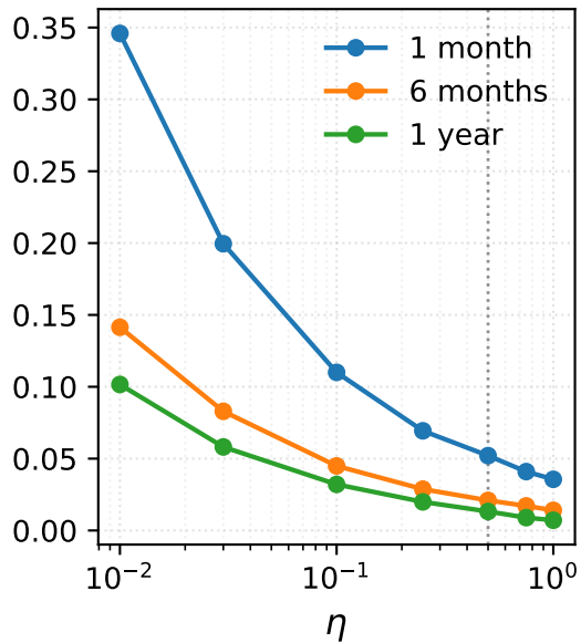
Median rel. CI width (diag. PSD)
