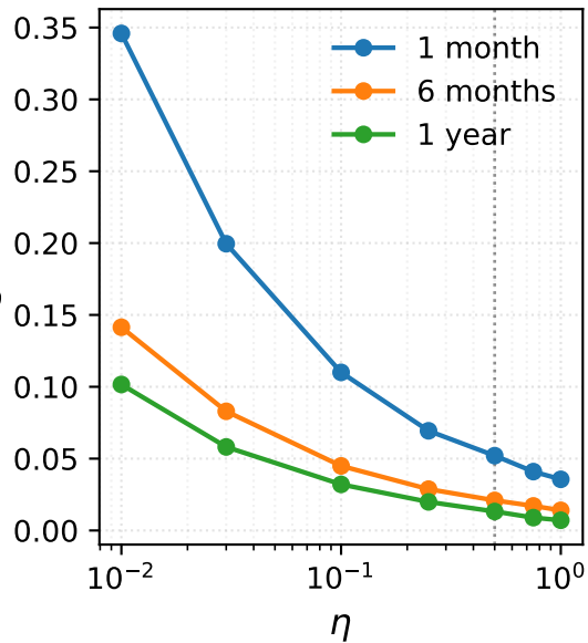
Median rel. CI width (diag. PSD)
