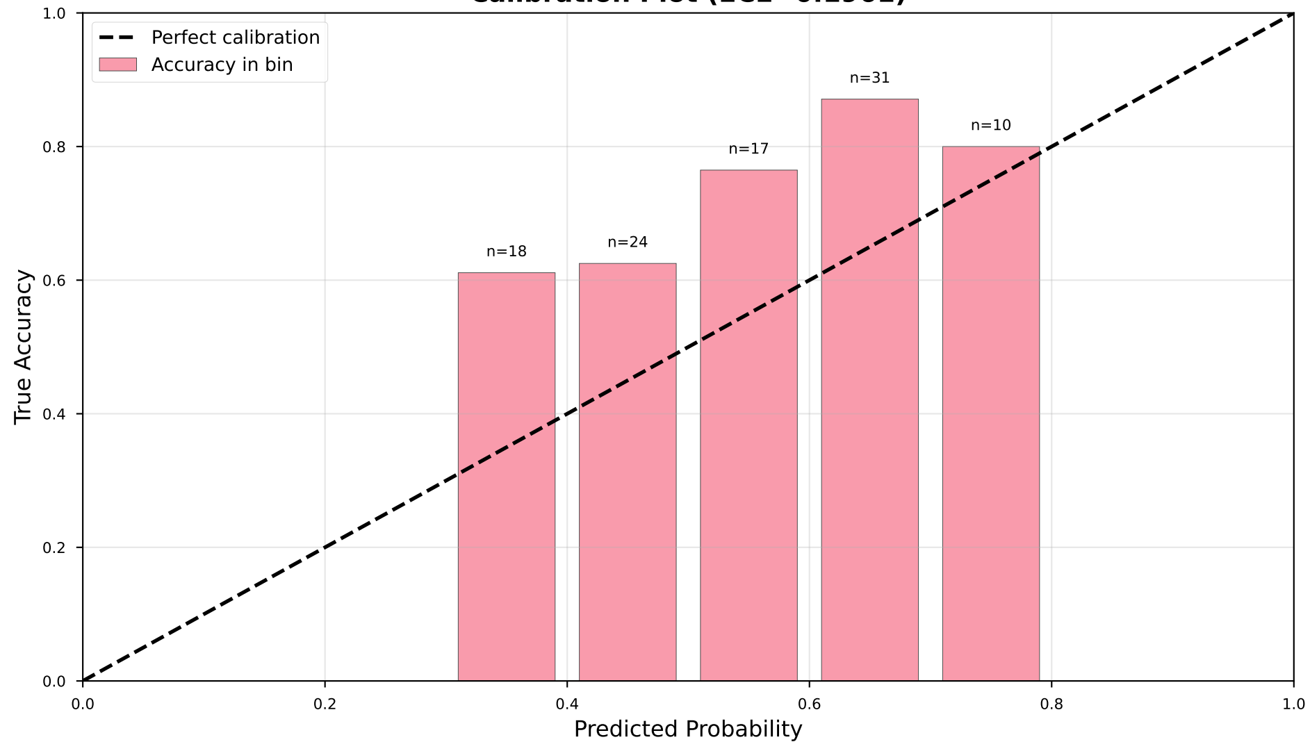
Calibration Plot (ECE=0.1961)
