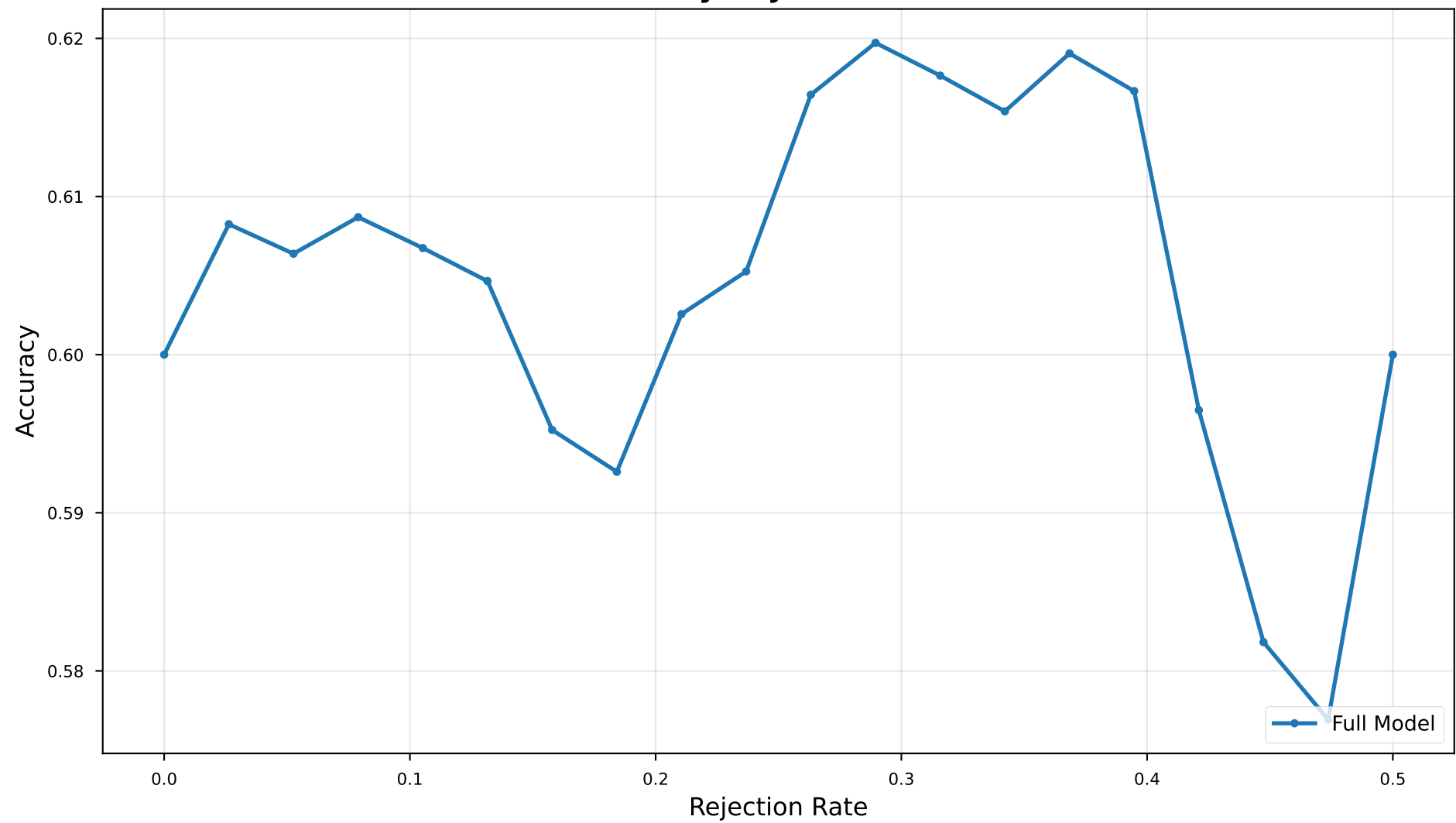
Accuracy-Rejection Curve
