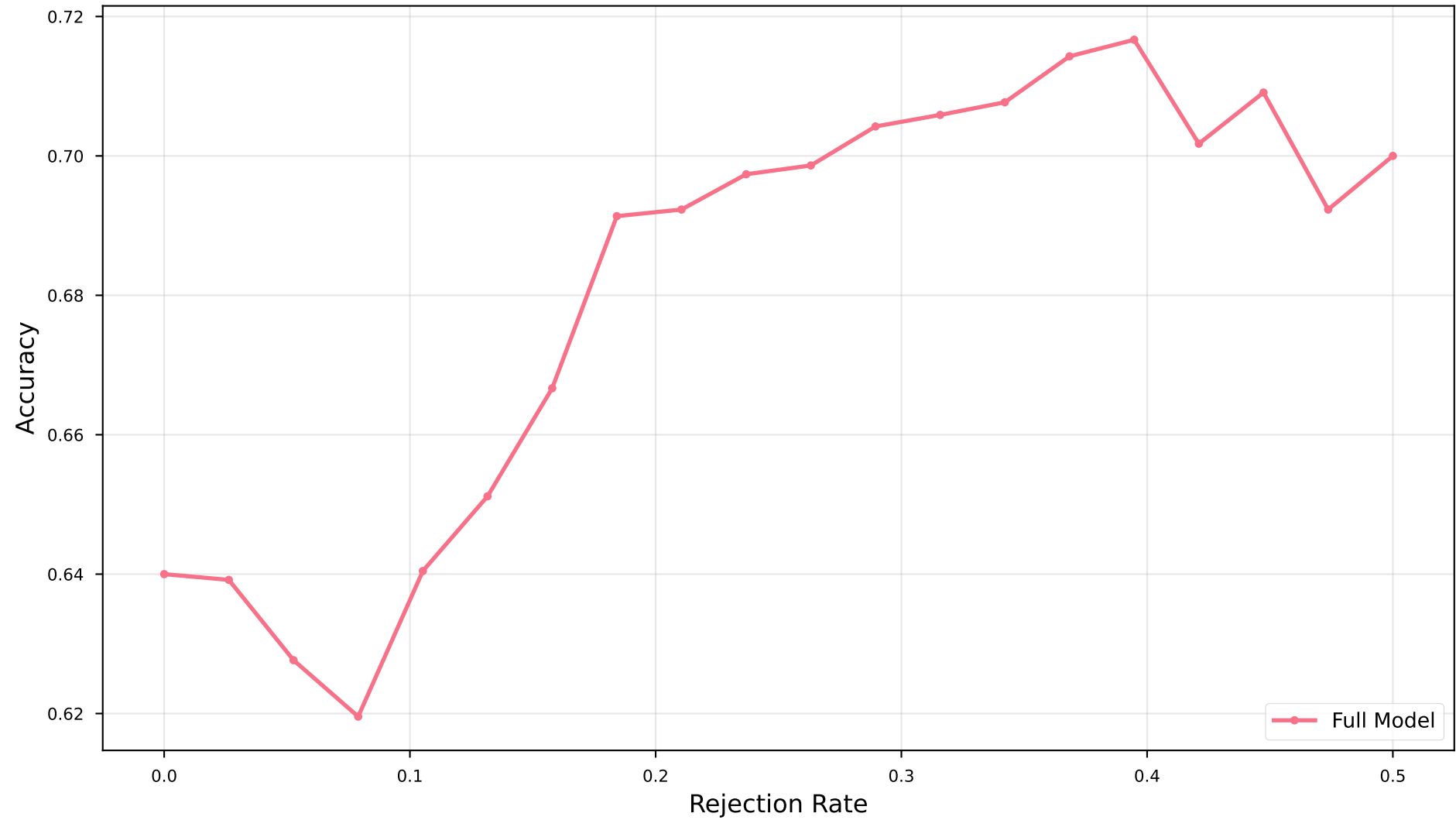
Accuracy-Rejection Curve
