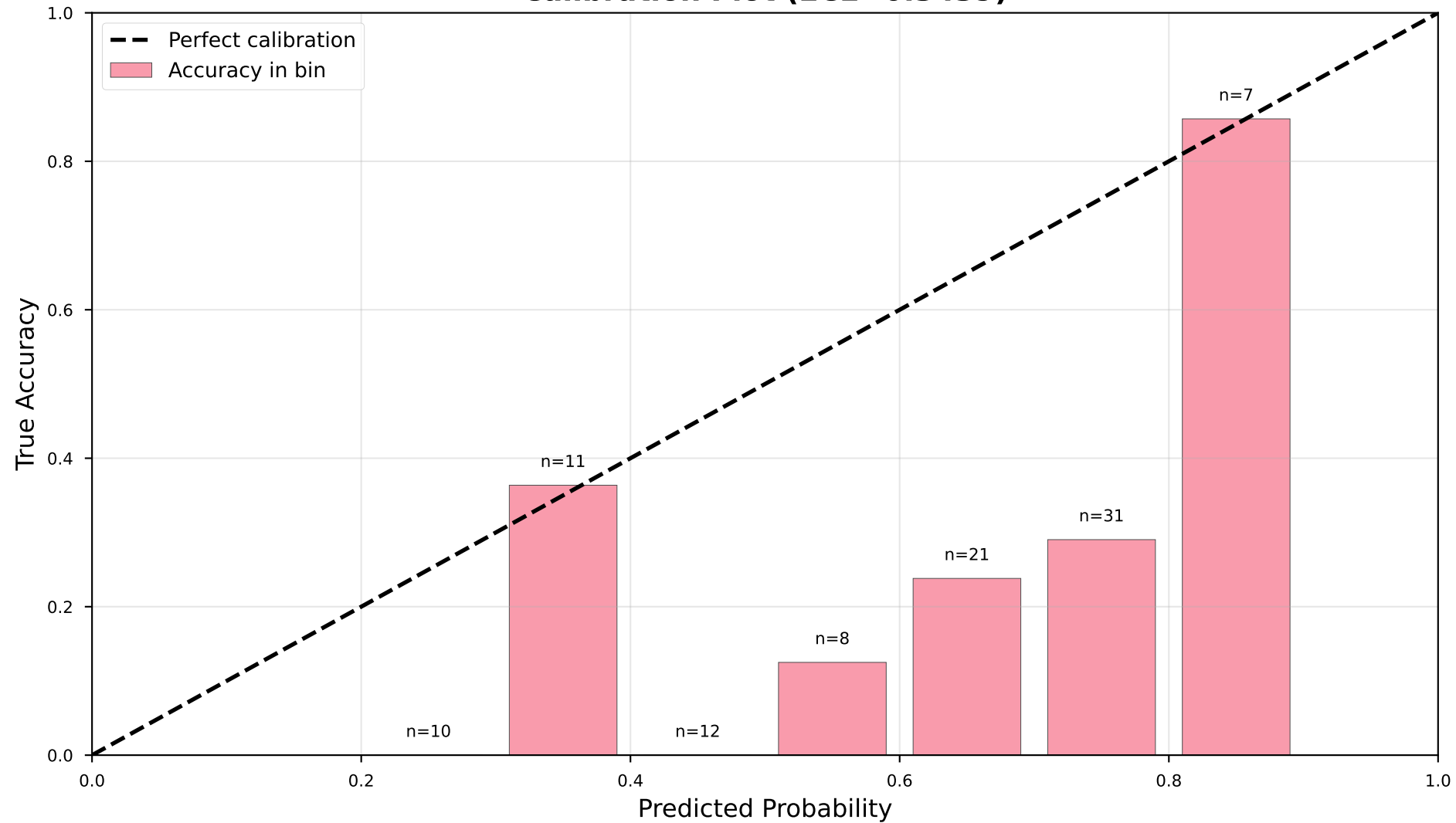
Calibration Plot (ECE=0.3439)
