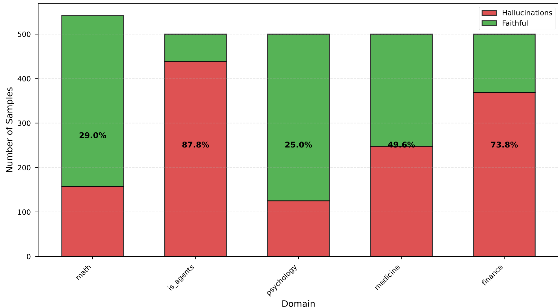
RQ3a: Hallucination Rate Distribution Across Domains
