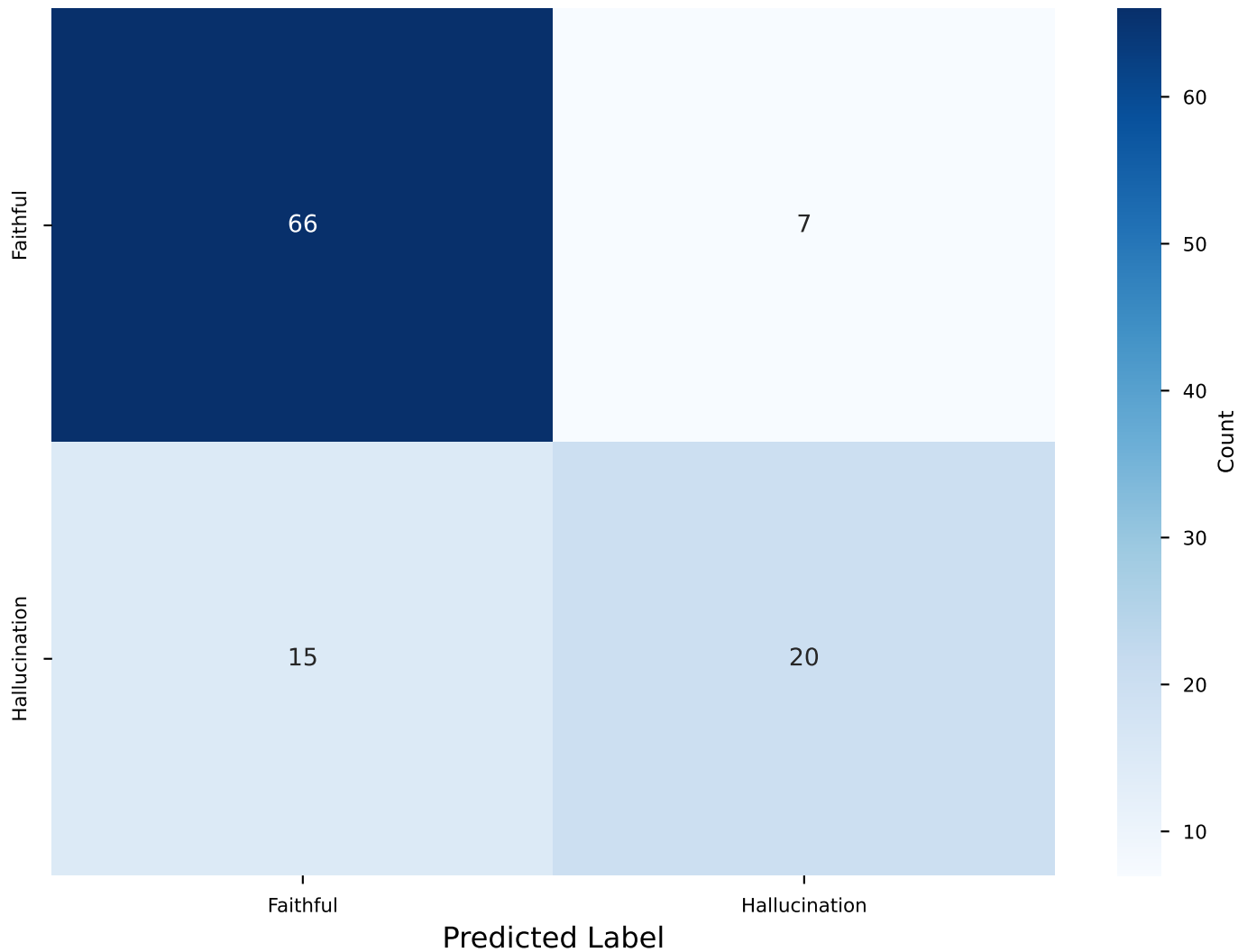
Confusion Matrix
