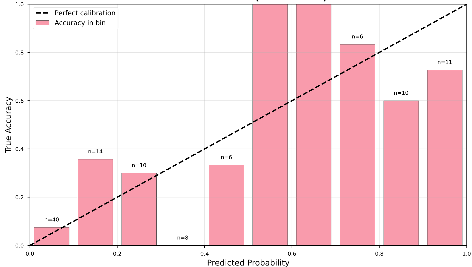
Calibration Plot (ECE=0.1404)
