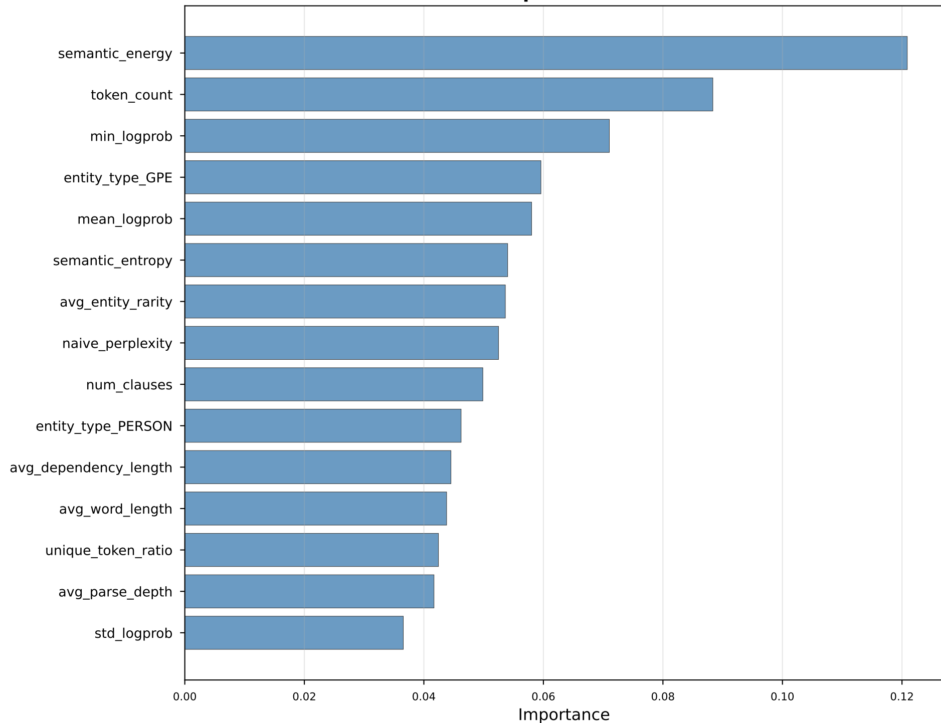
Feature Importance - Finance
