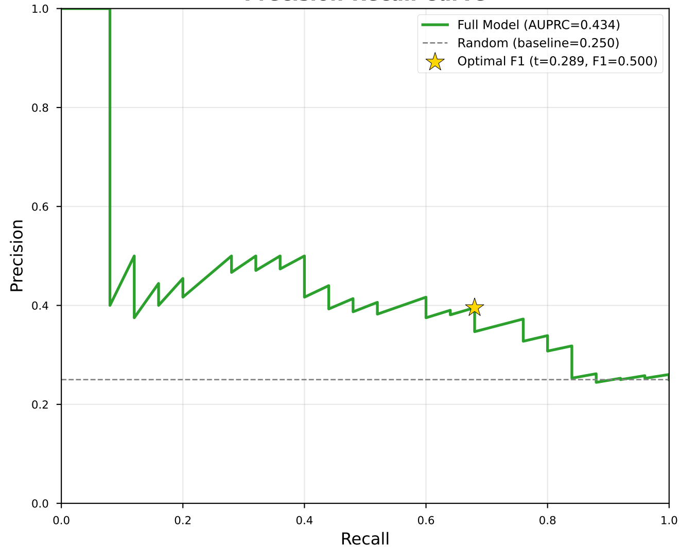
Precision-Recall Curve
