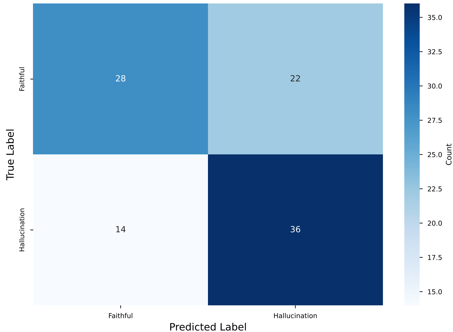
Confusion Matrix
