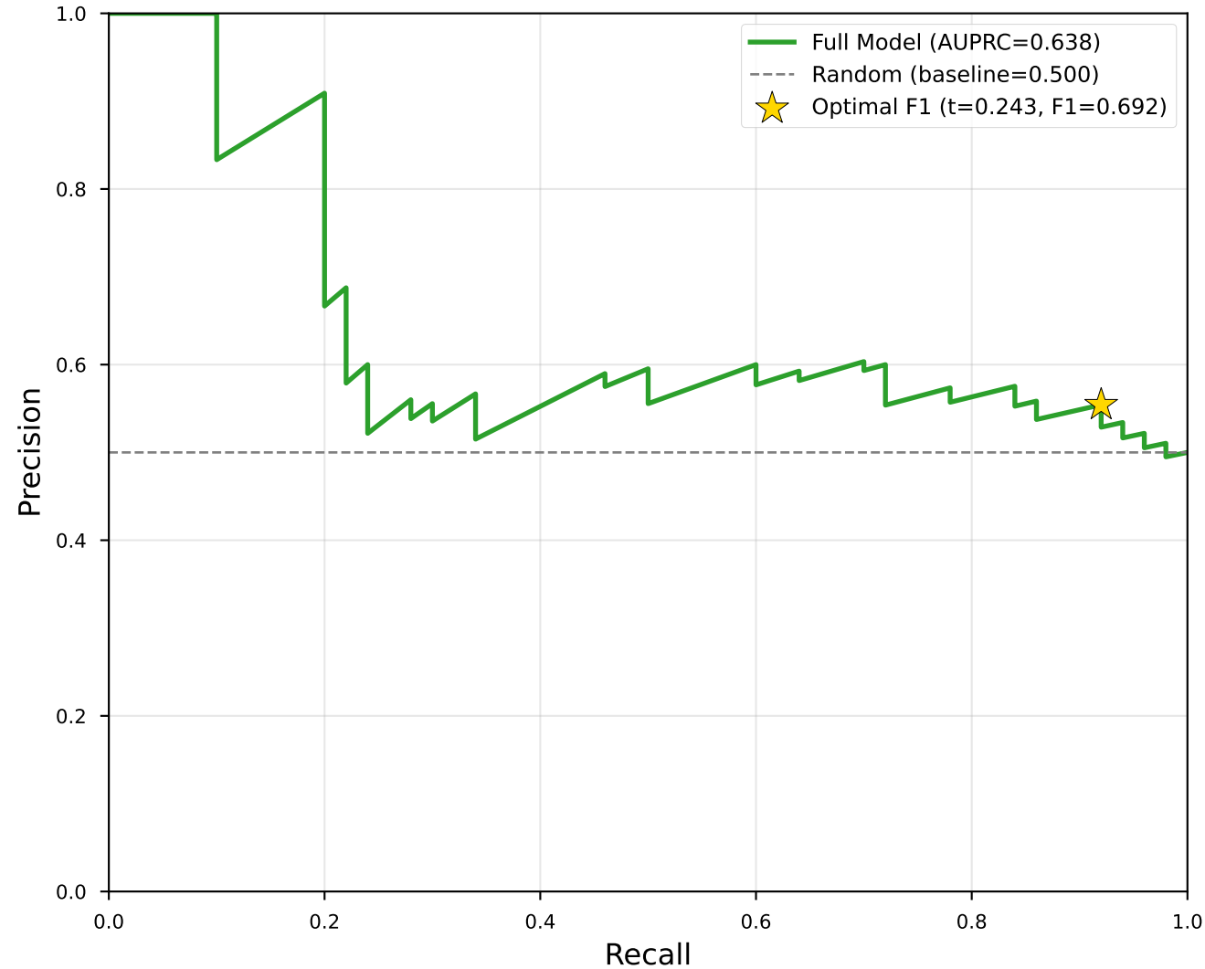
Precision-Recall Curve
