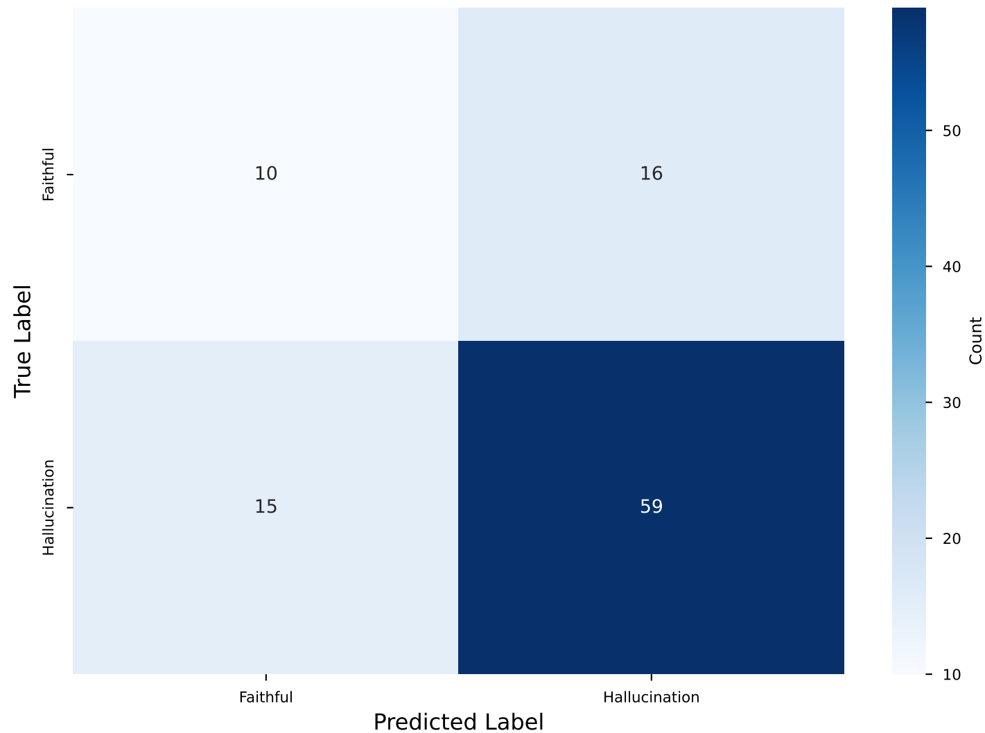
Confusion Matrix
