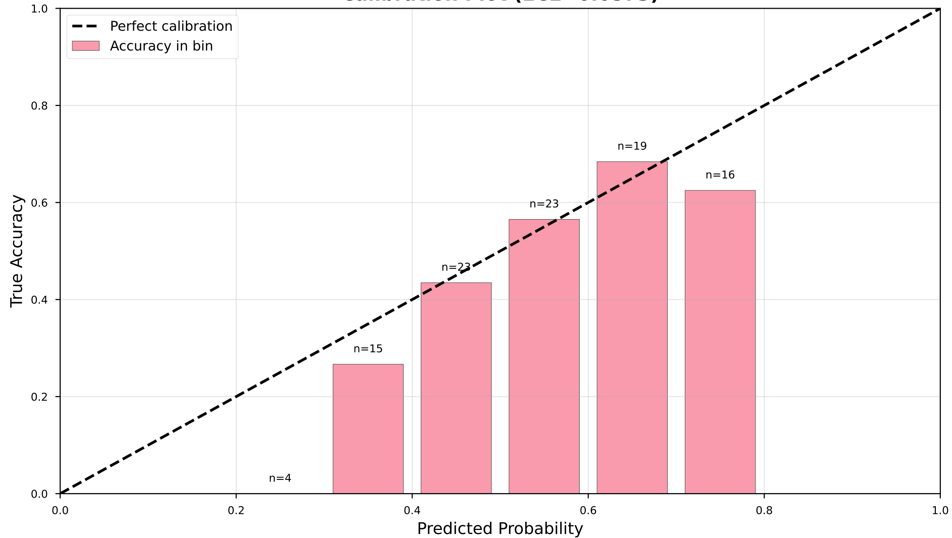
Calibration Plot (ECE=0.0573)
