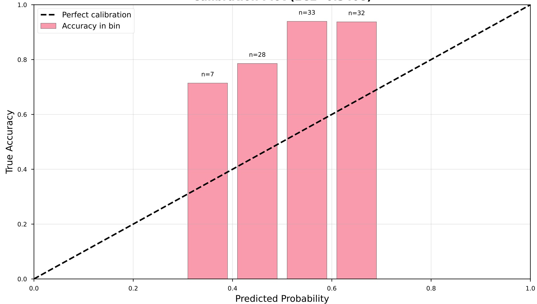
Calibration Plot (ECE=0.3408)
