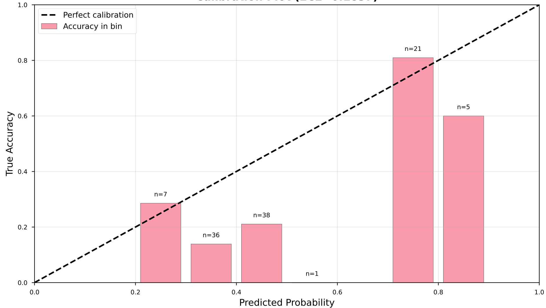
Calibration Plot (ECE=0.1837)
