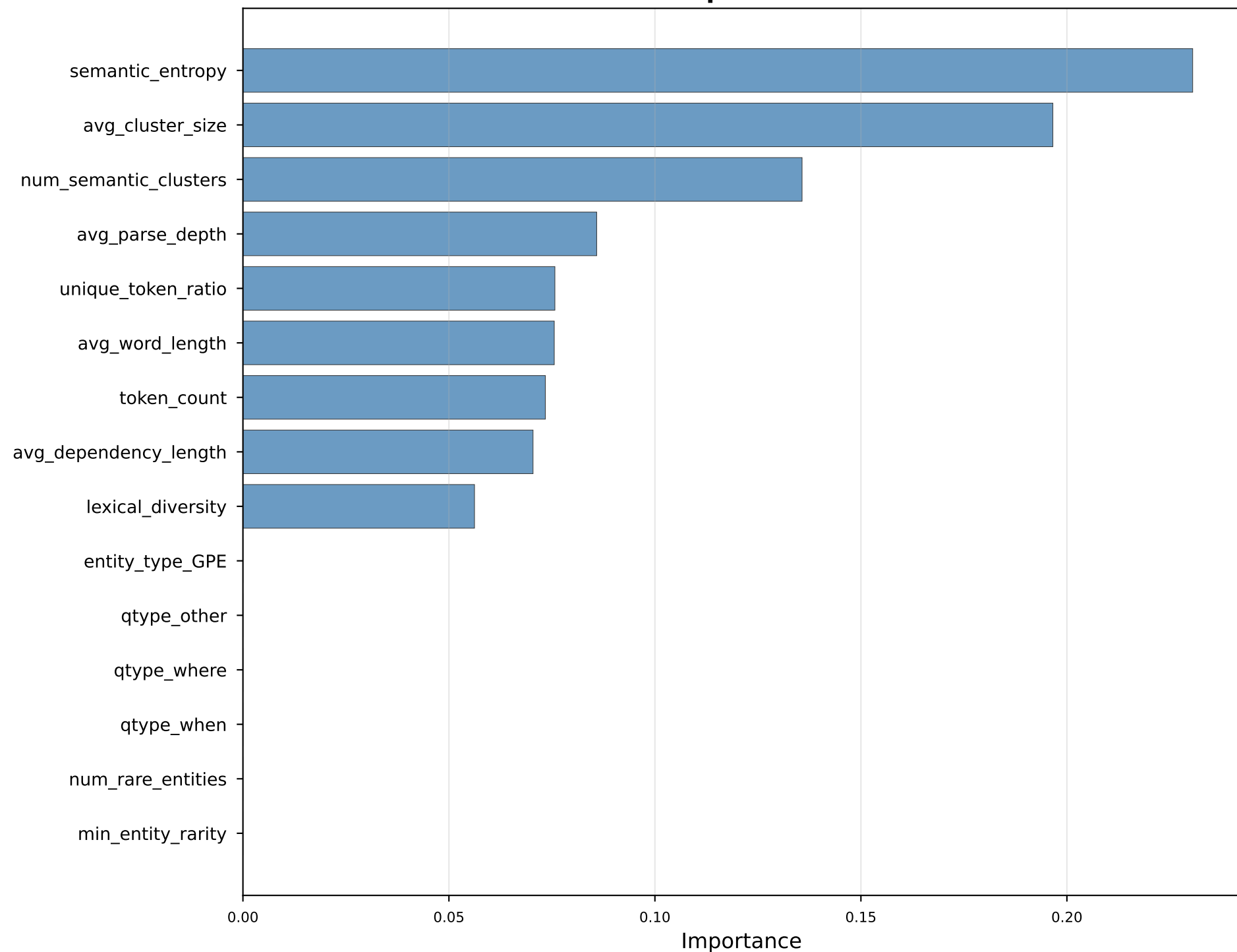
Feature Importance - Math
