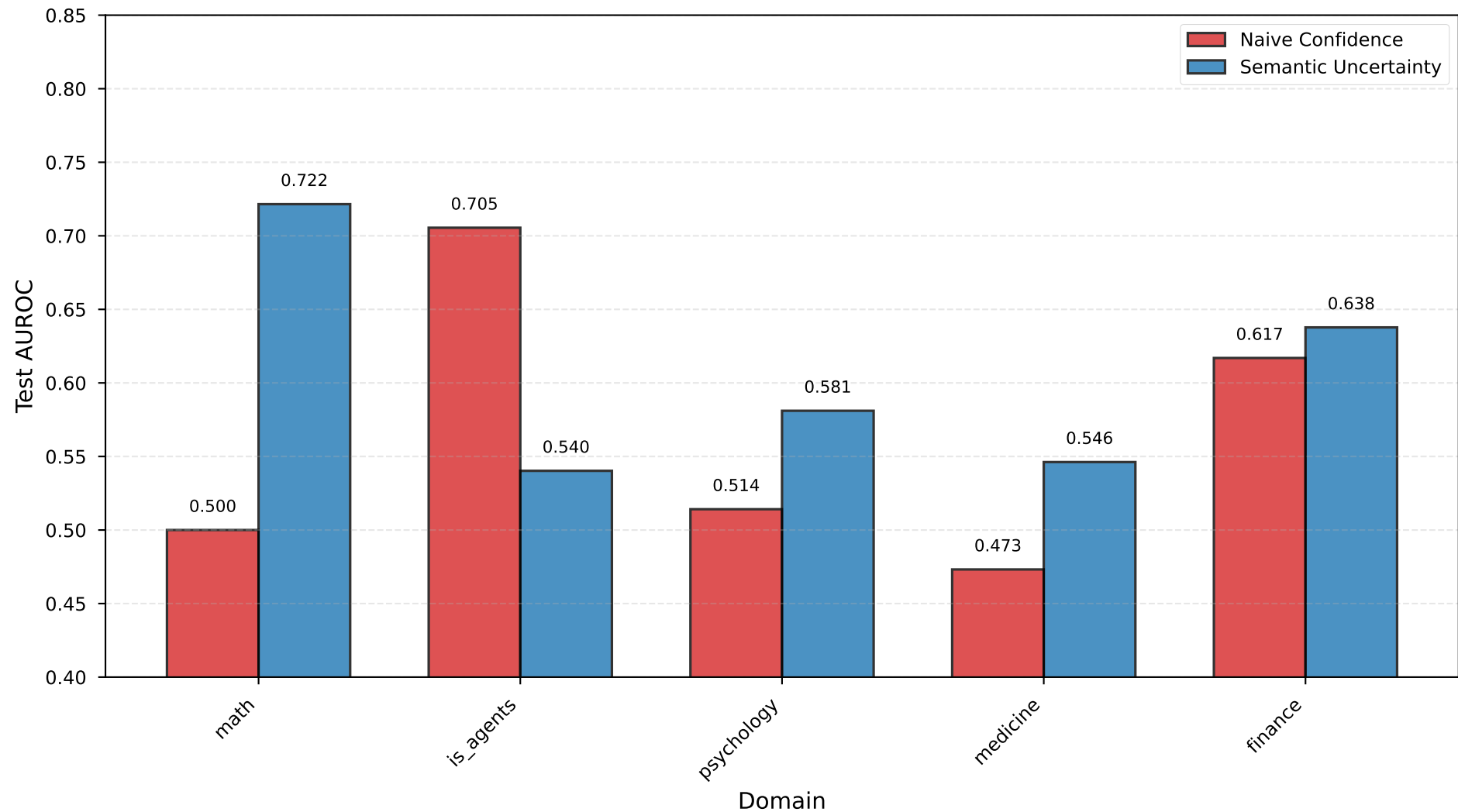
RQ2: Semantic Uncertainty vs Naive Confidence by Domain
