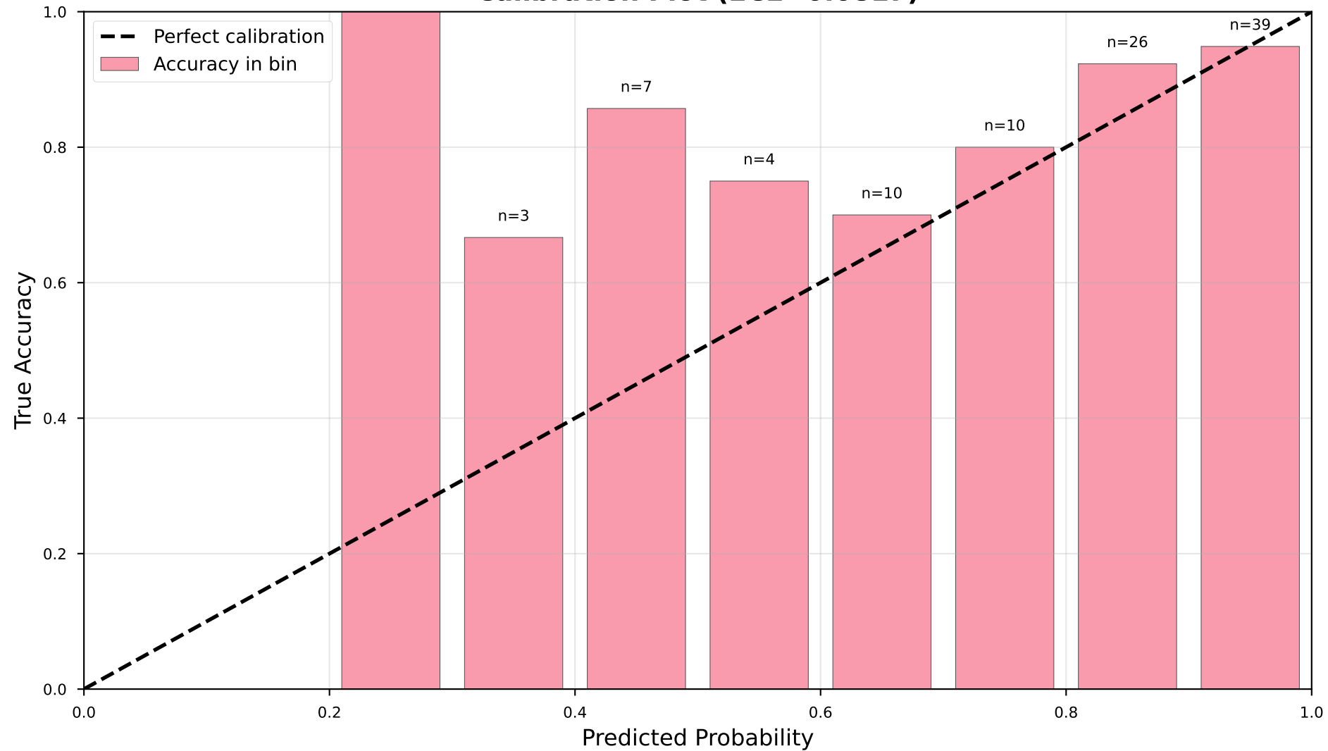
Calibration Plot (ECE=0.0817)
