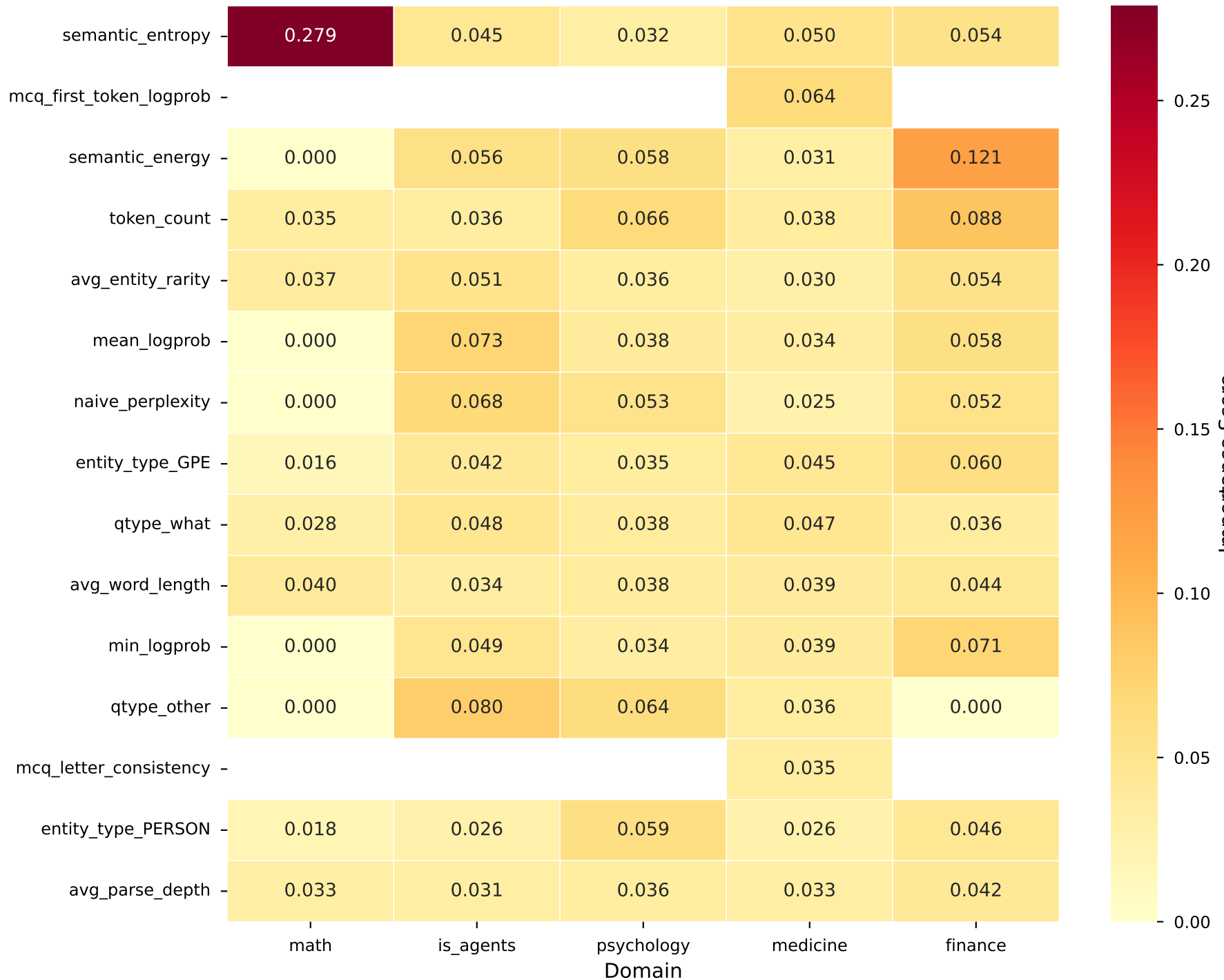
RQ3c: Top 15 Feature Importance Across Domains
