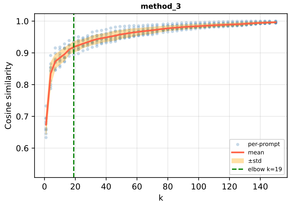
Cosine similarity vs k (spread across 10 prompts) — Layer 5, Head 1
