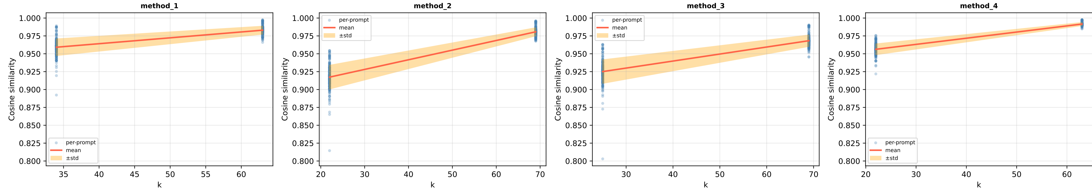
Cosine similarity vs k (spread across 90 prompts) — Layer 5, Head 1
