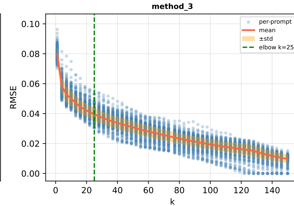
RMSE vs k (spread across 225 prompts) — Layer 5, Head 1
