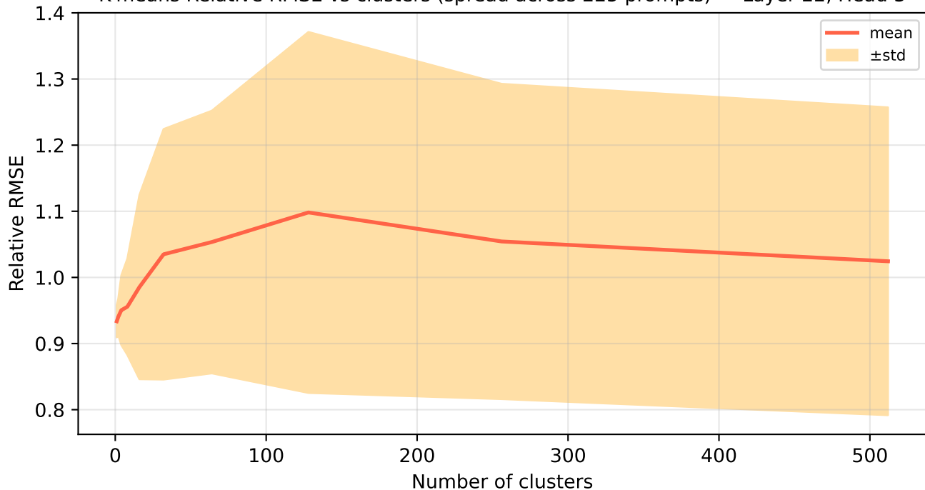
K-means Relative RMSE vs clusters (spread across 225 prompts) — Layer 22, Head 3
