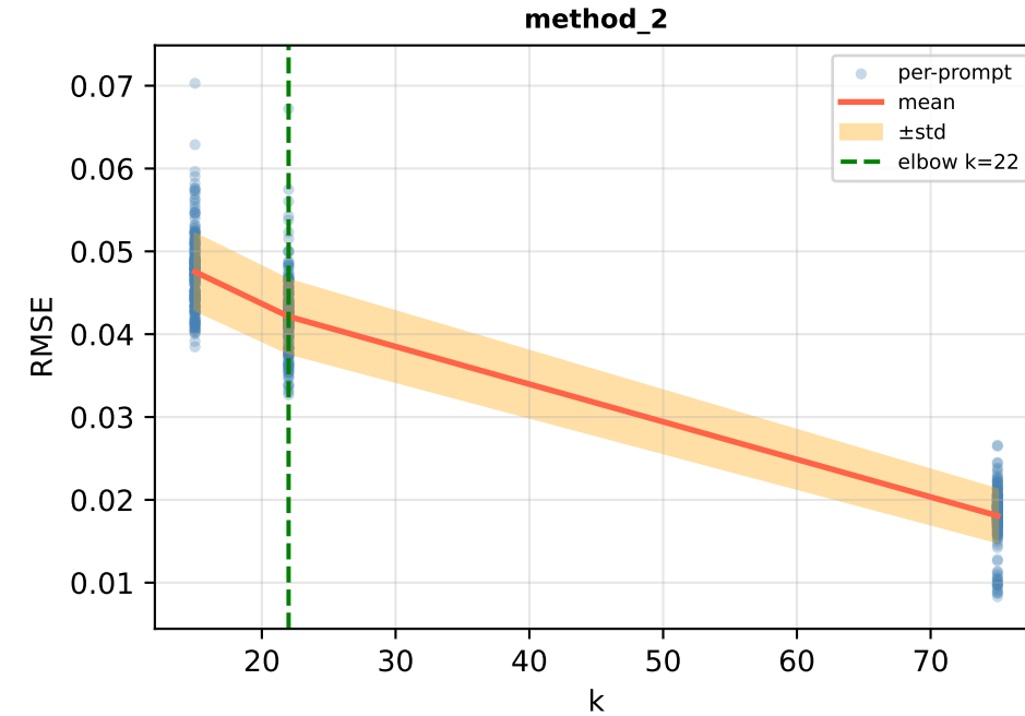
RMSE vs k (spread across 96 prompts) — Layer 5, Head 1
