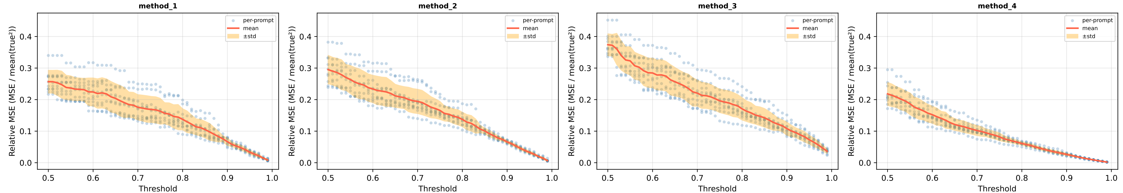
Relative MSE vs threshold (spread across 10 prompts) — Layer 5, Head 1
