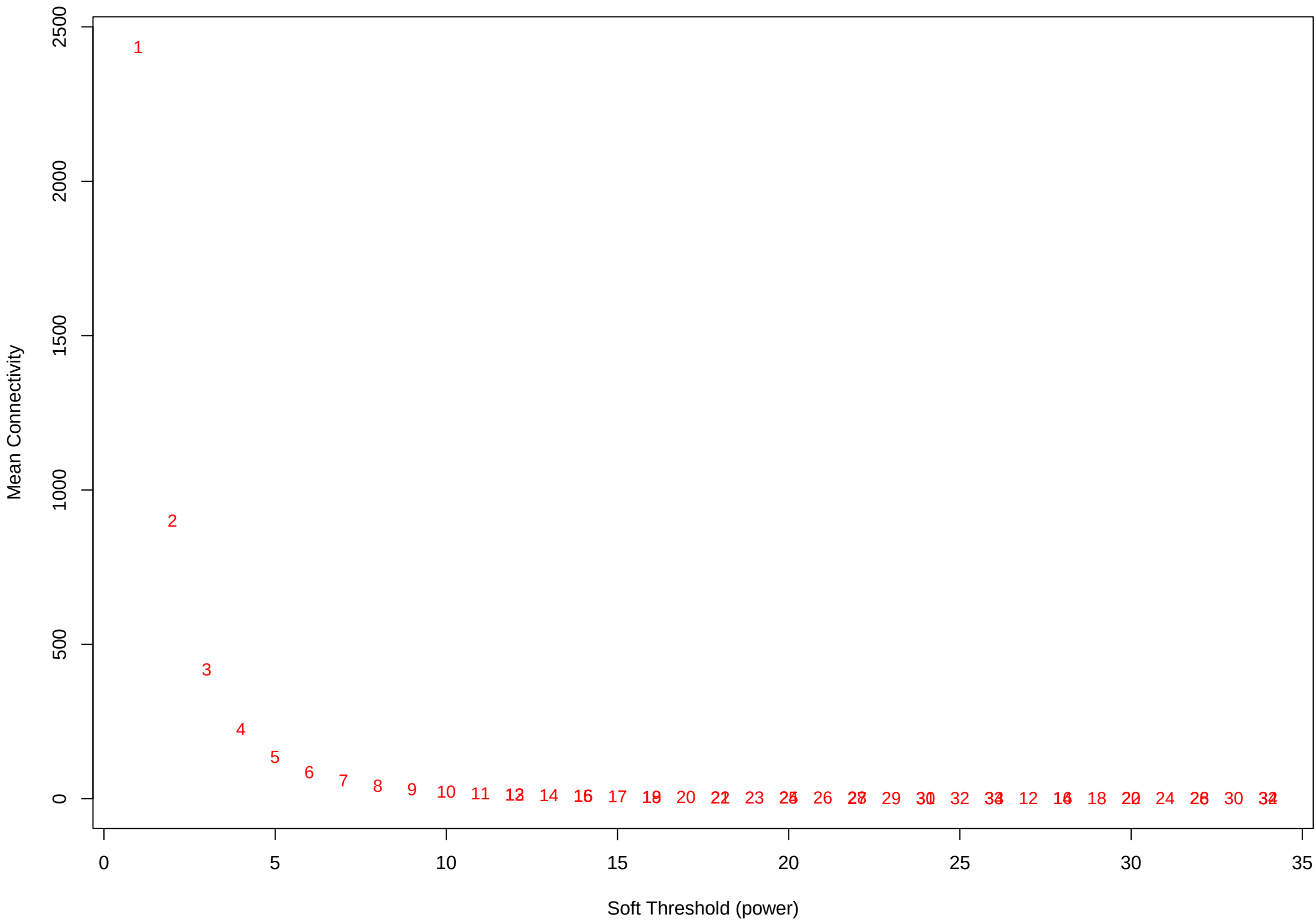
Mean connectivity
