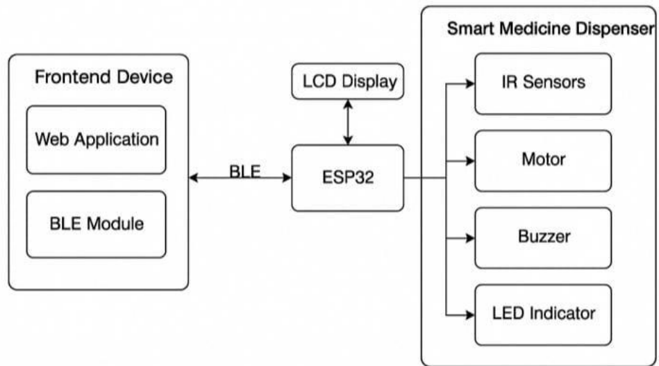
Smart Medicine Reminder and Dispensing System
