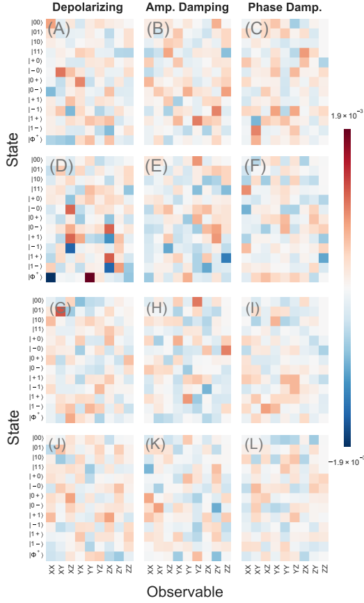
Fig. 2: IBM Boston vs Quantinuum H2 .
