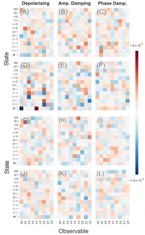
Fig. 2: IBM Boston vs Quantinuum H2 .
