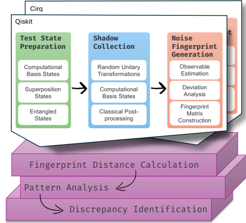
Fig. 1: SIMSHADOW Architecture
