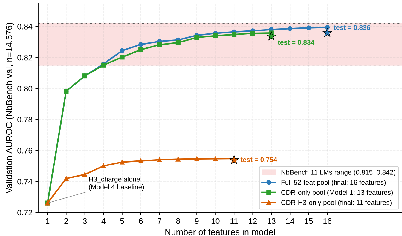
Forward-selection climb: full, CDR-only, CDR-H3-only pools
