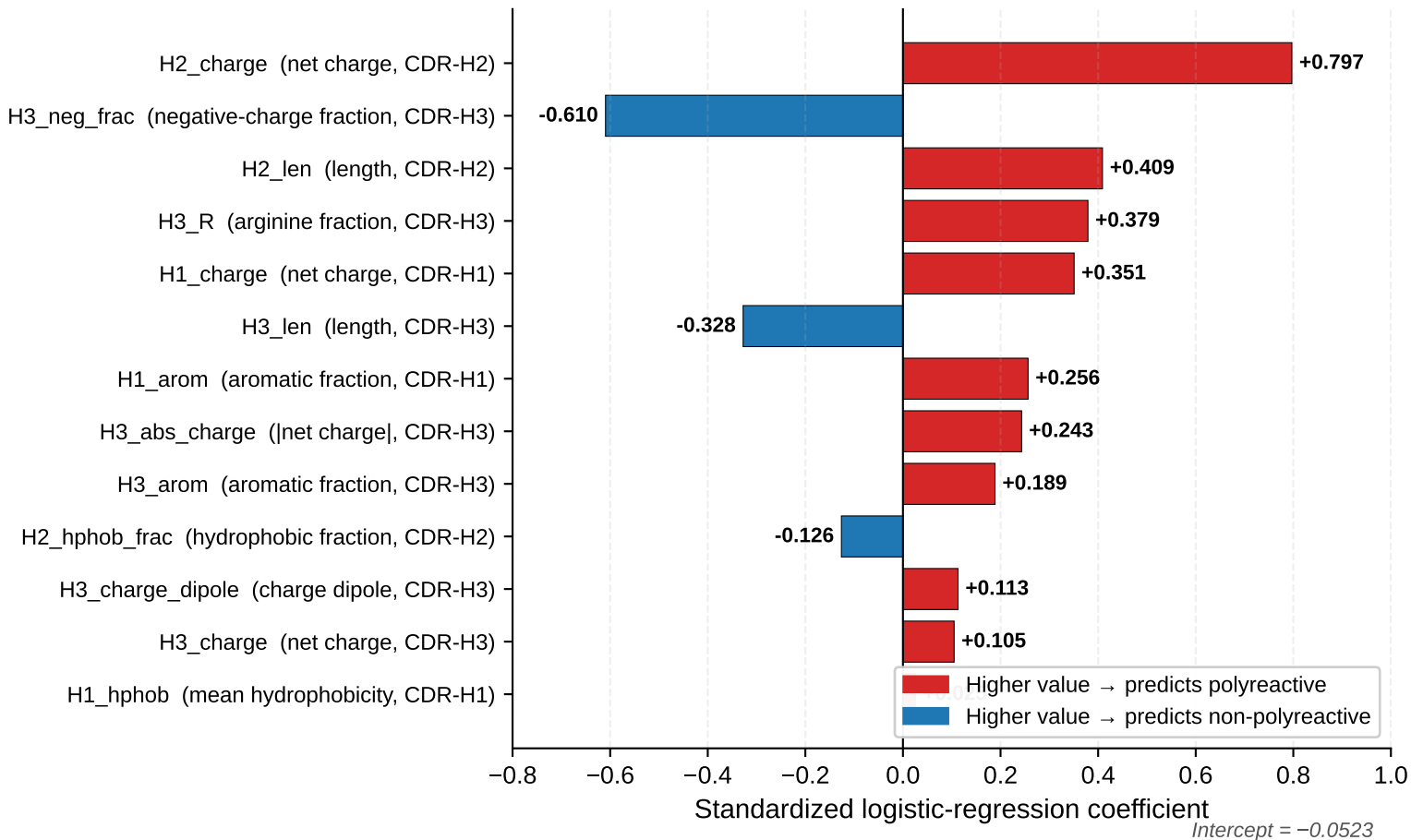
Model 1 (13-feature CDR-only) fitted coefficients
