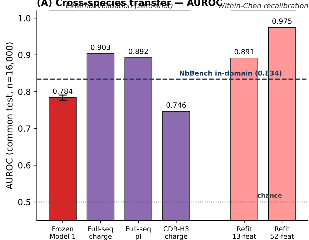
(A) Cross-species transfer — AUROC
