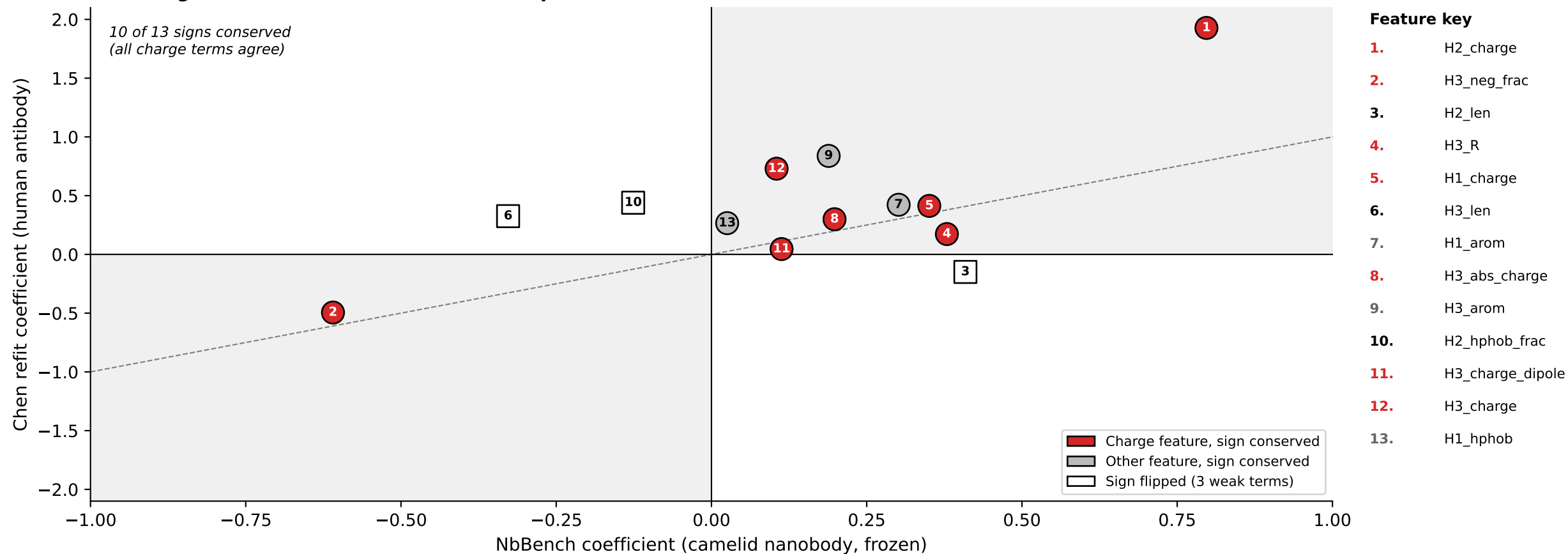
(C) Charge coefficients conserved across species
