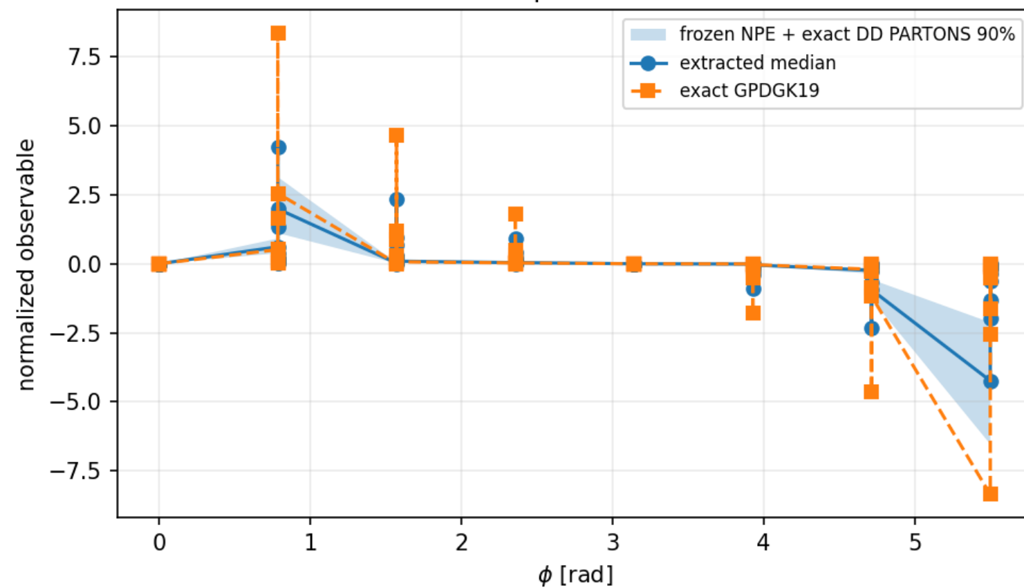
Beam-spin asymmetry
