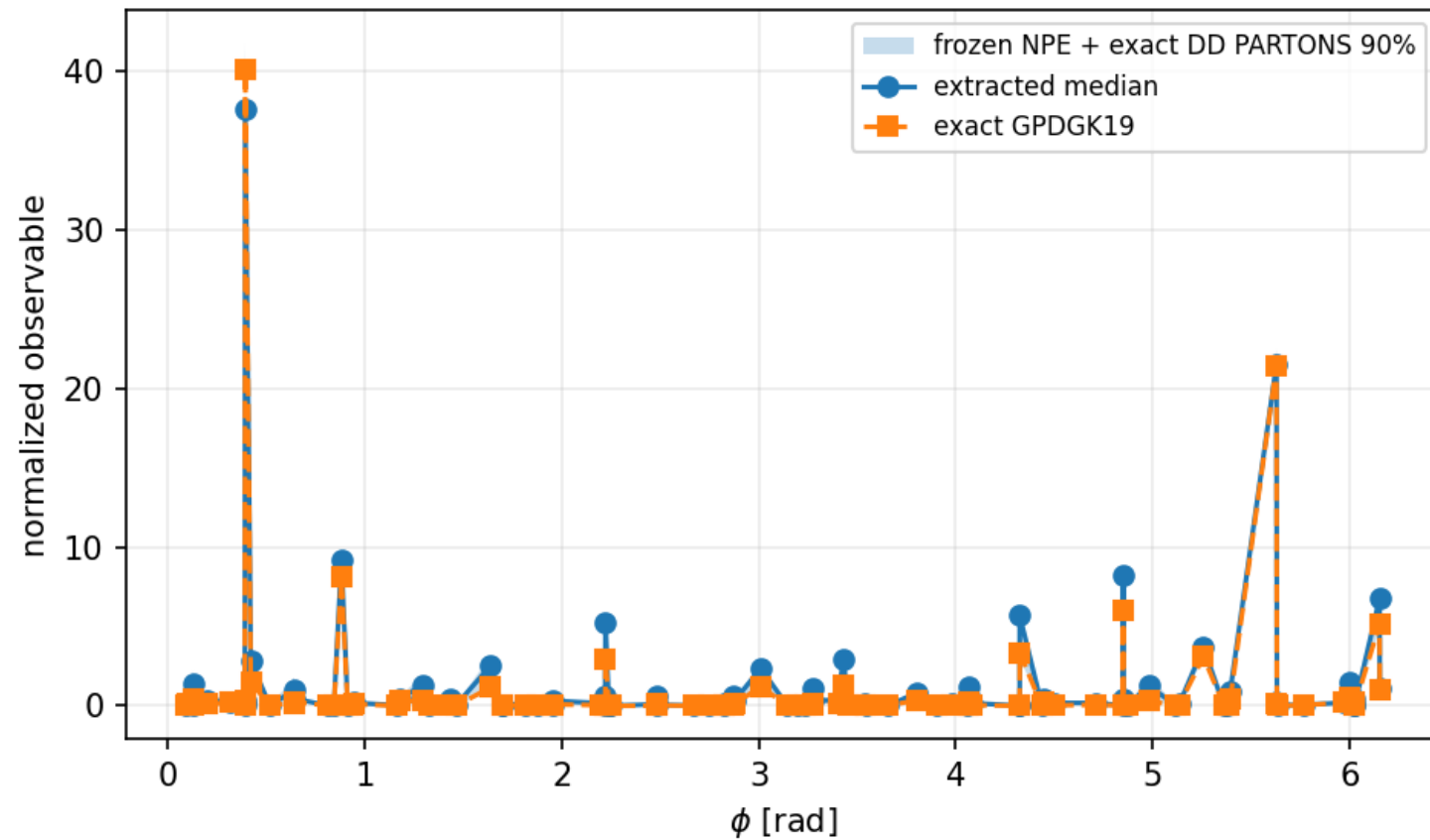
Beam-charge asymmetry
