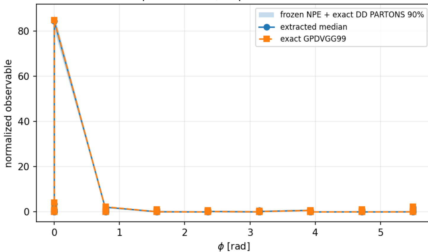
Beam-charge asymmetry
