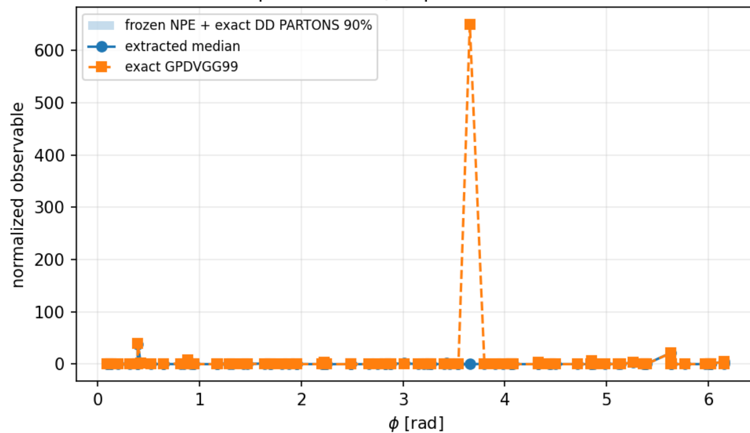
Beam-charge asymmetry
