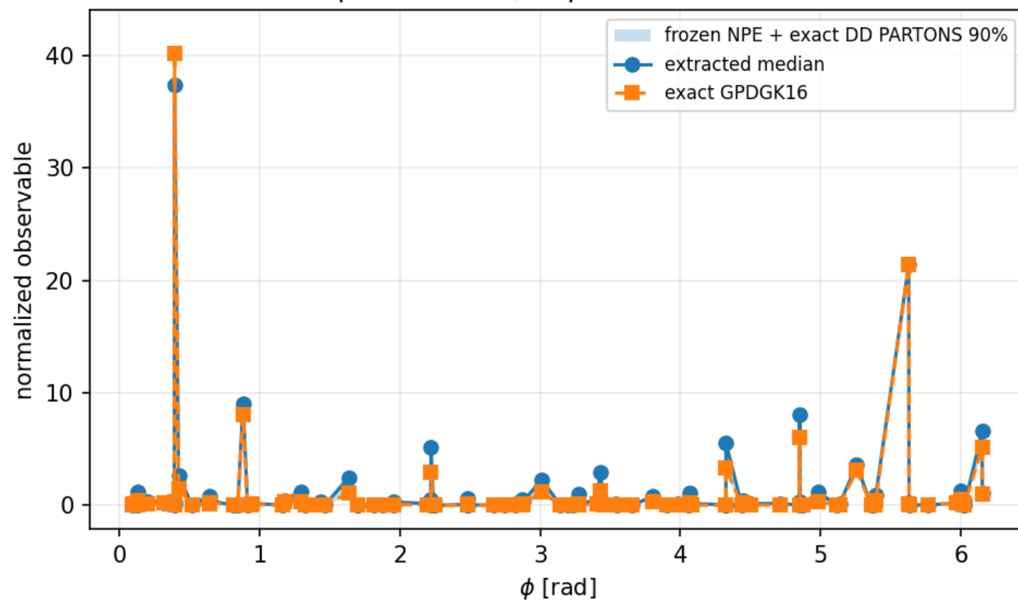
Beam-charge asymmetry
