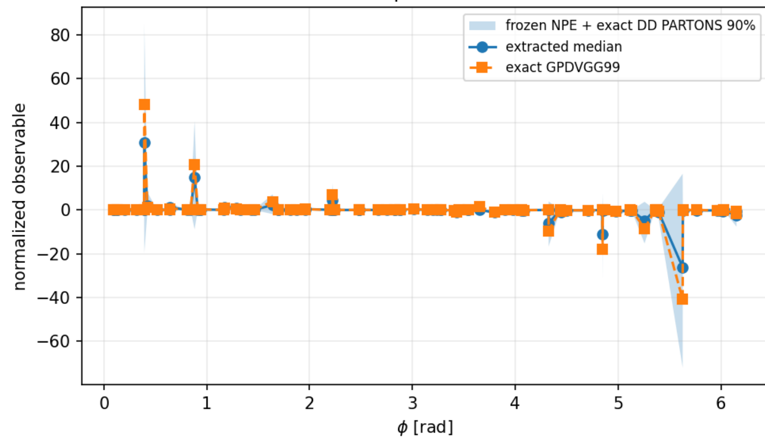
Beam-spin asymmetry
