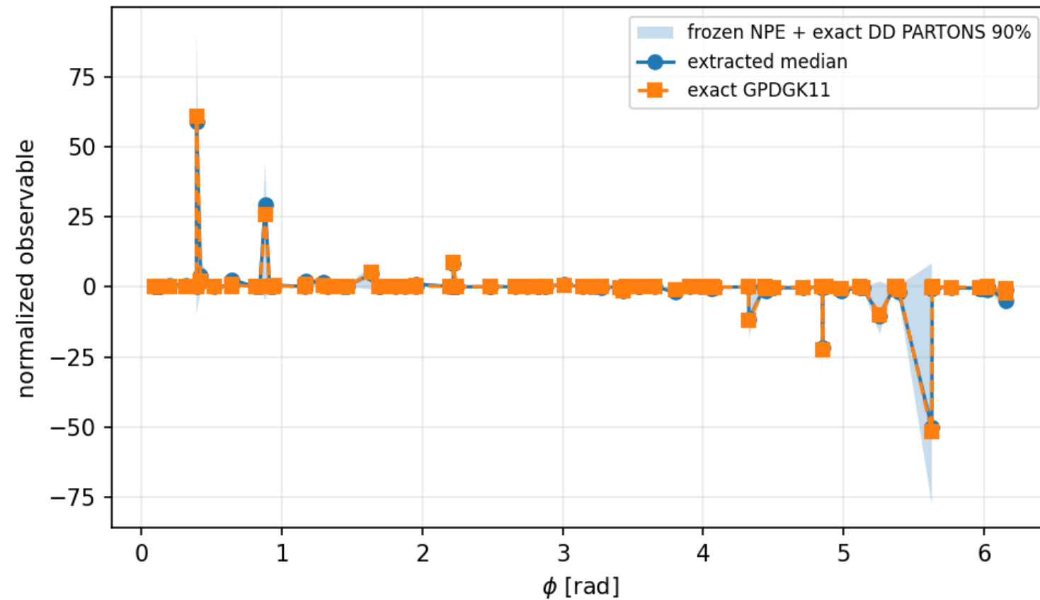
Beam-spin asymmetry
