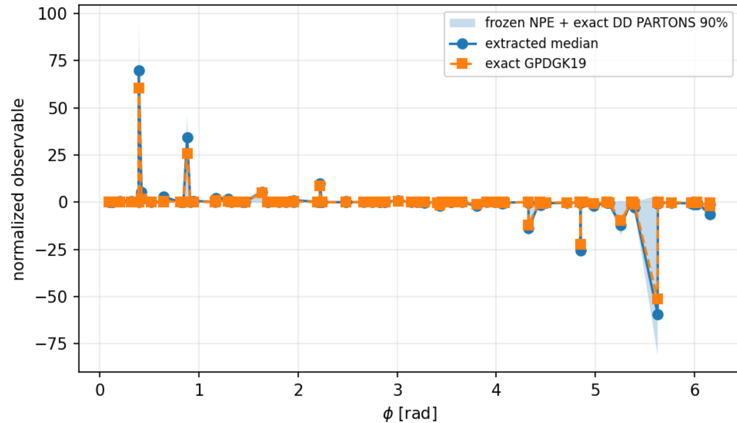
Beam-spin asymmetry
