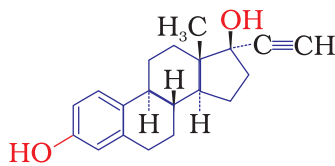
Ethynylestradiol (novestrol)
