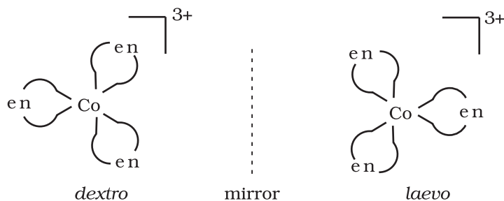
Fig.5.6: Optical isomers ( d and l ) of [Co(en)_3]^{3+}
