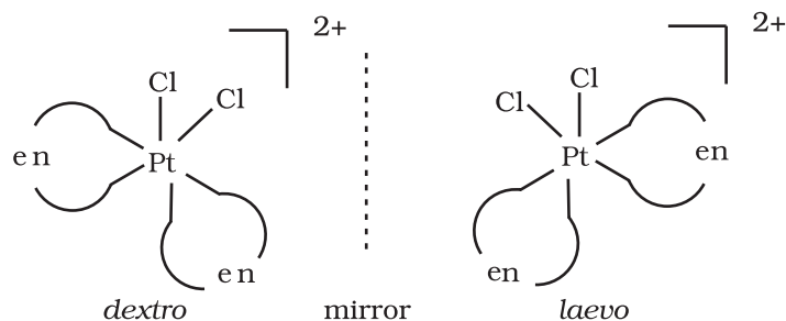
Fig.5.7 Optical isomers ( d and l ) of cis - [PtCl_2(en)_2]^{2+}
