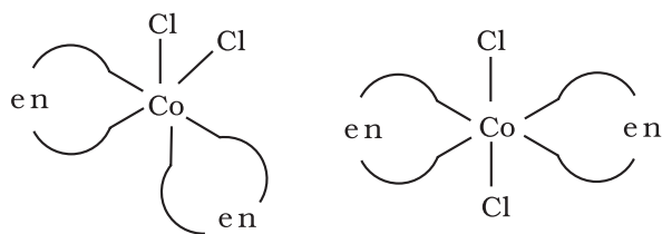
Fig. 5.4: Geometrical isomers ( cis and trans ) of [CoCl_2(en)_2]
