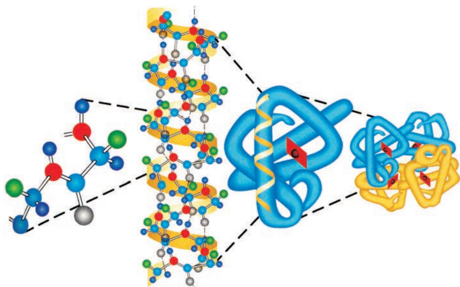
Fig. 10.3: Diagrammatic representation of protein structure (two sub-units of two types in quaternary structure)
