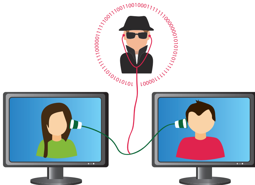
Figure 12.6: Eavesdropping
