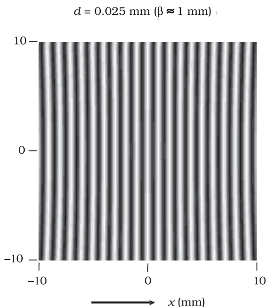
FIGURE 10.13 Computer generated fringe pattern produced by two point source S_1 and S_2 on the screen GG' (Fig. 10.12); correspond to d = 0.025 \text{ mm} , D = 5 \text{ cm} and \lambda = 5 \times 10^{-5} \text{ cm} . (Adopted from OPTICS by A. Ghatak, Tata McGraw Hill Publishing Co. Ltd., New Delhi, 2000.)
