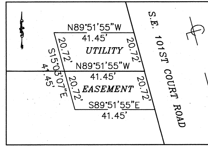
DETAIL C 1"=30'
