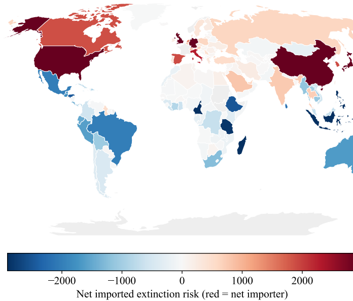
Figure 2: The geography of outsourced extinction risk, 2013.
