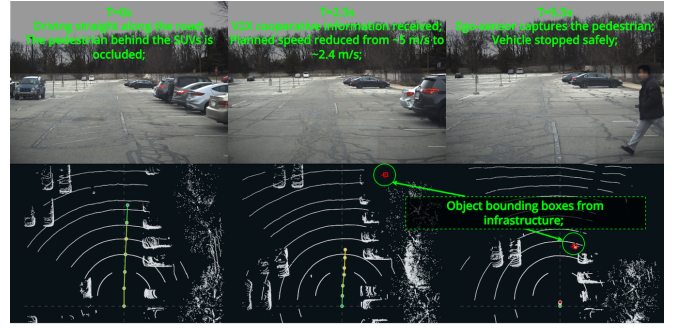
Fig. 5: Real-world demonstration of V2X cooperative driving. The LiDAR point cloud is only used for visualization.
