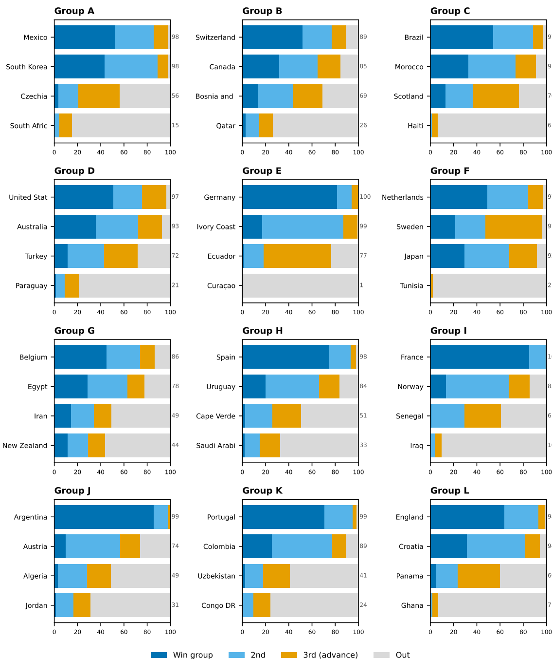
Figure 21: Qualification probability by team — Track B (result-conditioning + live Elo + bookmaker odds; live edition M017)
