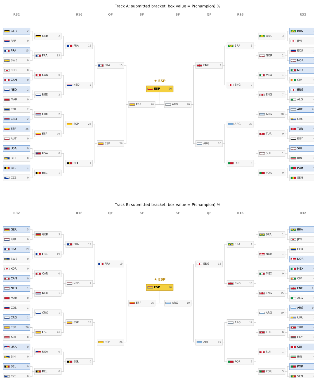
Figure 19: The submitted bracket re-valued by champion probability under Track A (top) and Track B (bottom) at live edition M035; the gold box is each track's most likely champion and greyed boxes are teams eliminated by confirmed results. The locked submitted bracket is Figure 18.
