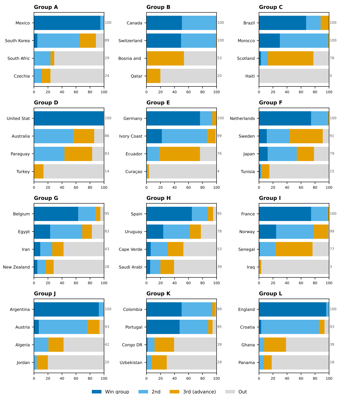
Figure 16: Qualification probability by team — Track A (conditioned on 33 results, June 10 ratings frozen; live edition M035)
