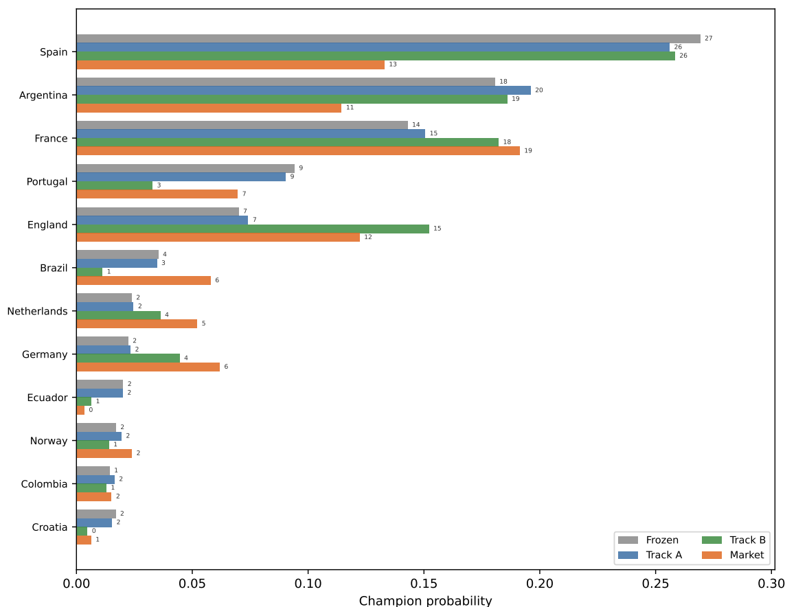
Figure 4: Champion probability, four ways: Frozen / Track A / Track B / Market, top twelve teams (live edition M035)
