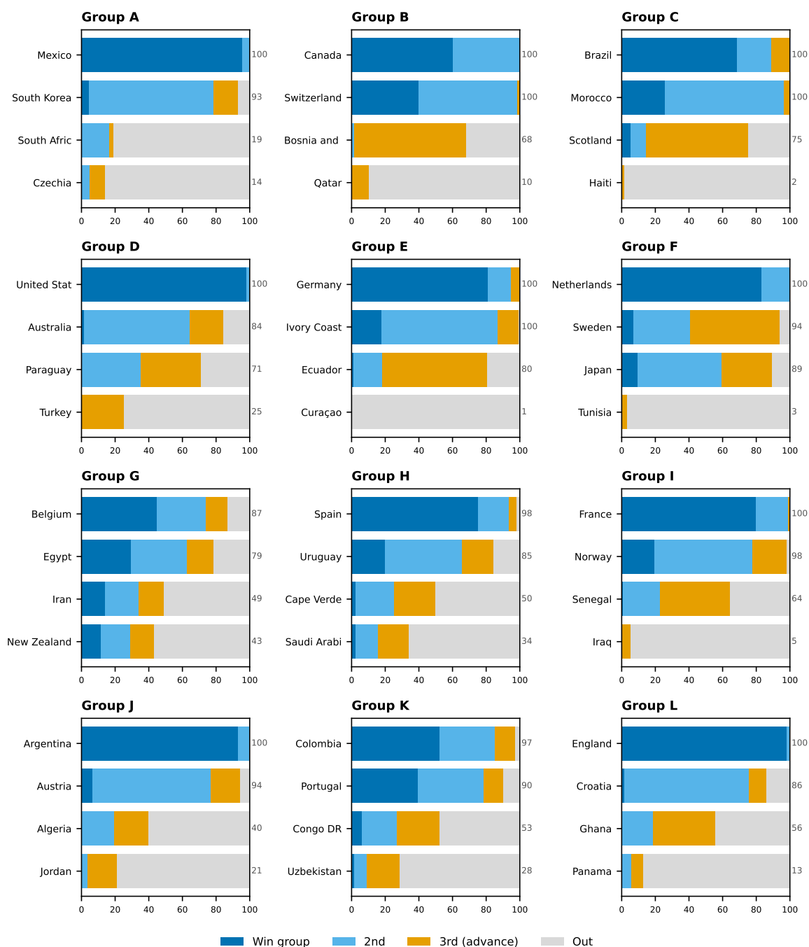
Figure 17: Qualification probability by team — Track B (result-conditioning + live Elo + bookmaker odds; live edition M035)
