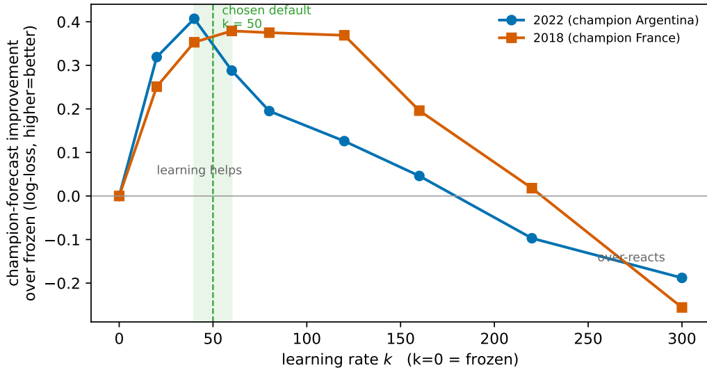
Figure 18: Learning-rate sweep on two World Cups
