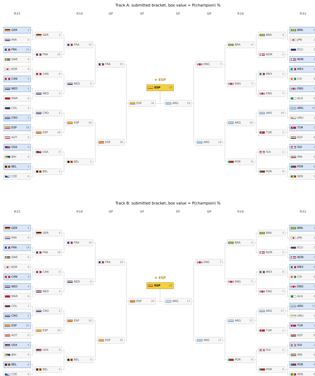
Figure 23: The submitted bracket re-valued by champion probability under Track A (top) and Track B (bottom) at live edition M019; the gold box is each track's most likely champion and greyed boxes are teams eliminated by confirmed results. The locked submitted bracket is Figure 22.
