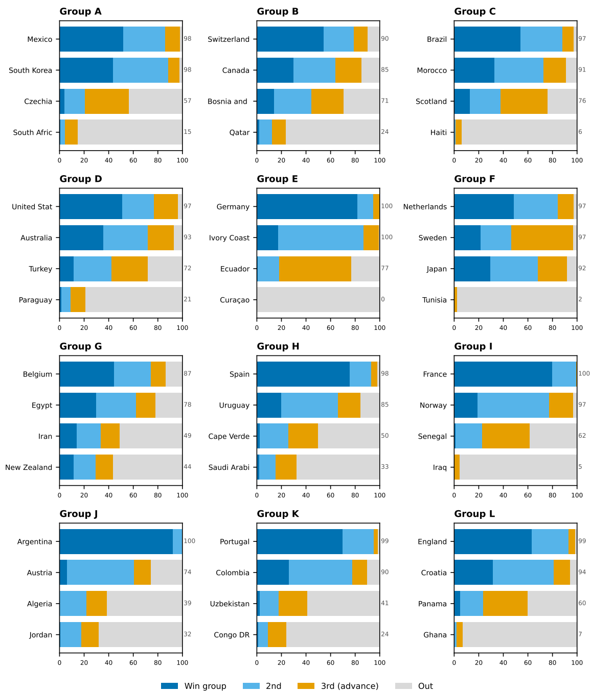
Figure 21: Qualification probability by team — Track B (result-conditioning + live Elo + bookmaker odds; live edition M019)
