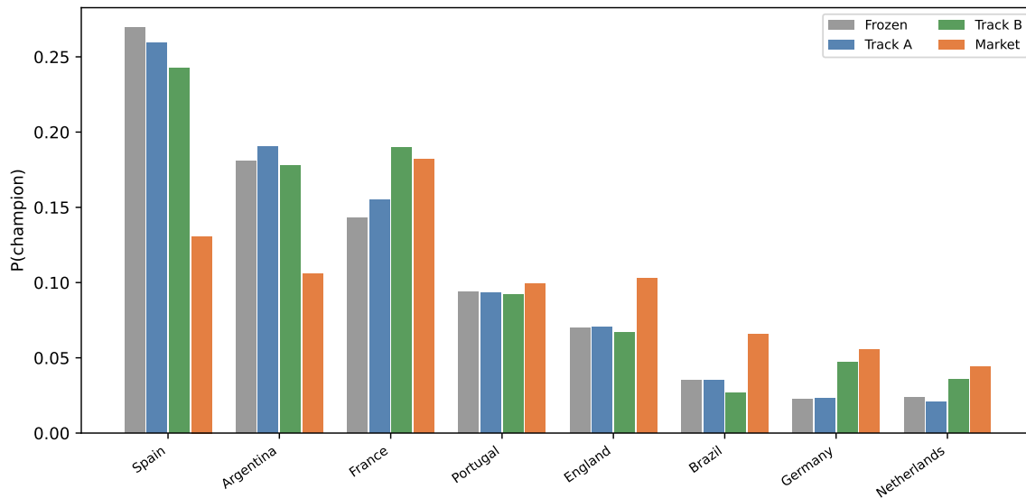
Figure 7: Four-bar champion probability: Frozen / Track A / Track B / Market, top contenders (live edition M019)
