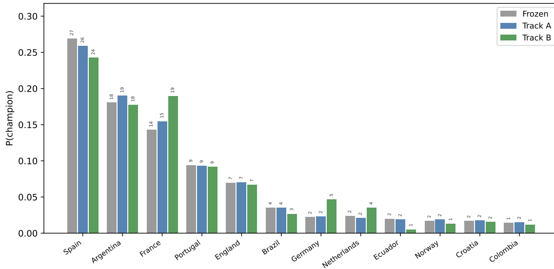
Figure 2: Champion probability distribution, conditioned on 19 results (live edition M019)
