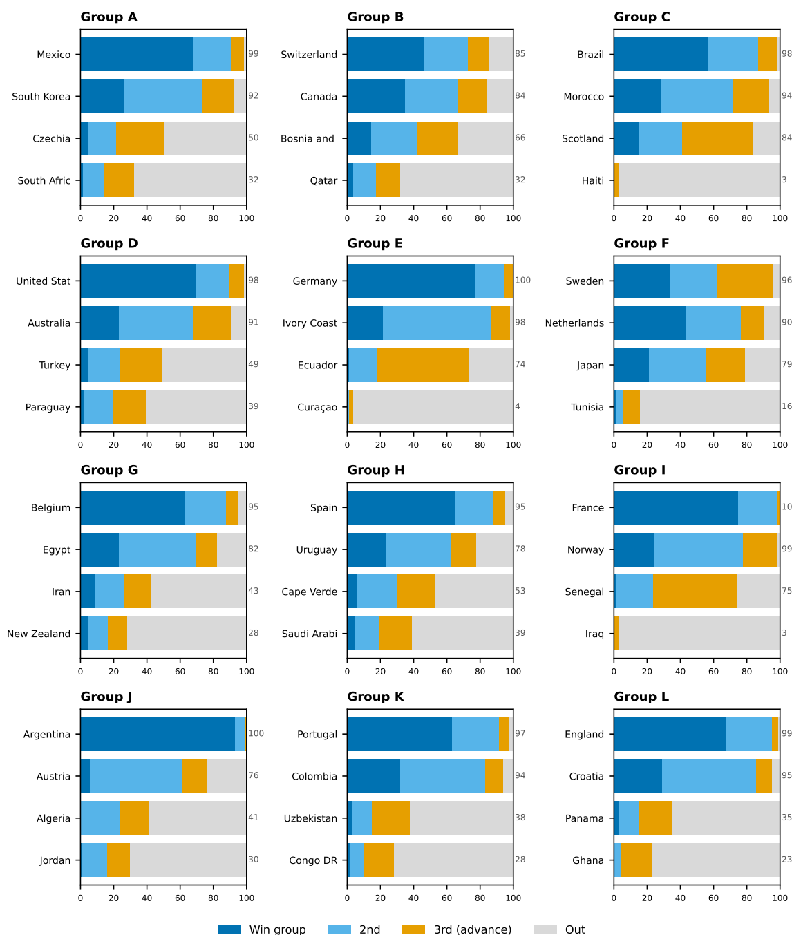
Figure 20: Qualification probability by team — Track A (conditioned on 19 results, June 10 ratings frozen; live edition M019)
