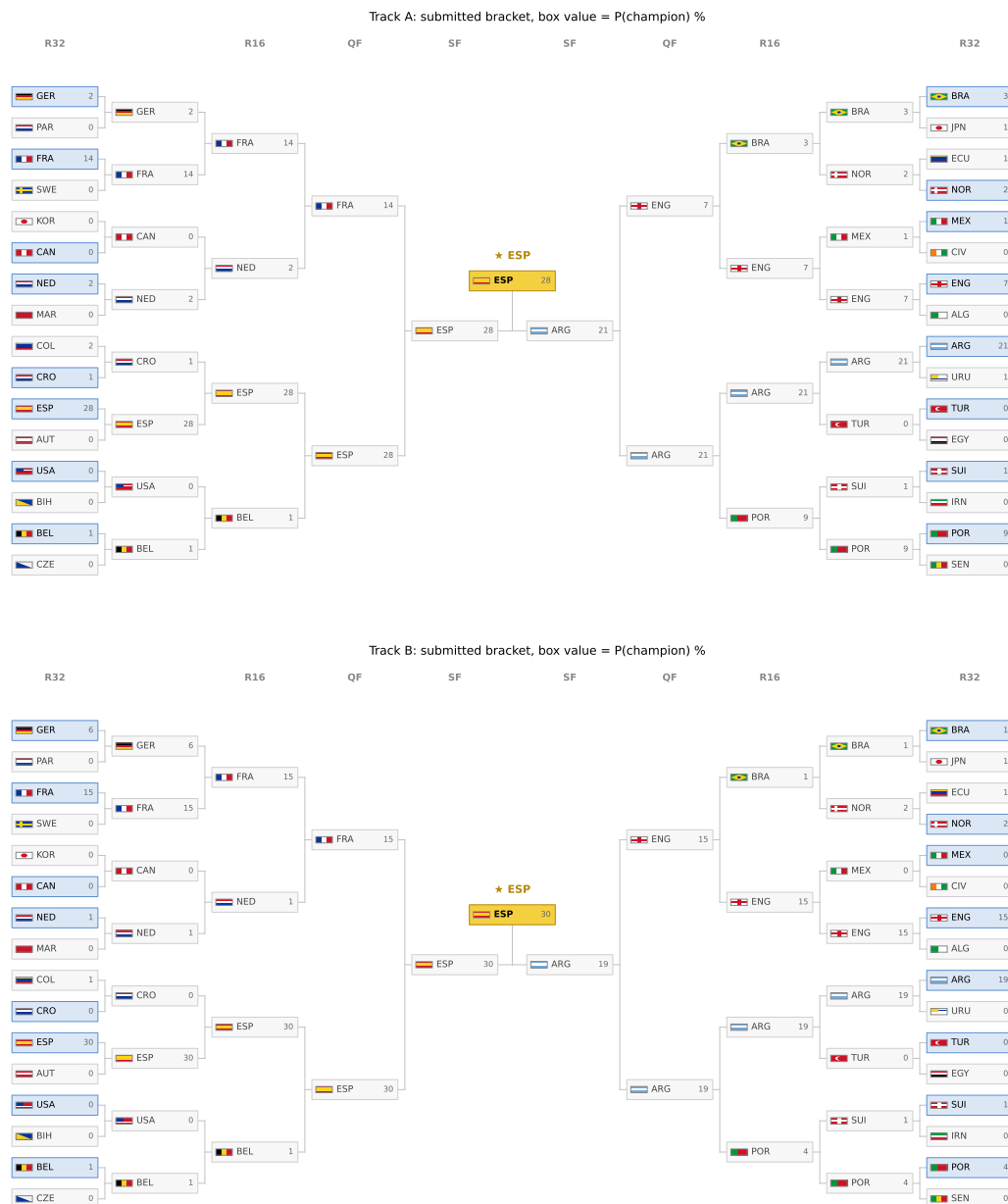
Figure 19: The submitted bracket re-valued by champion probability under Track A (top) and Track B (bottom) at live edition M041; the gold box is each track's most likely champion and greyed boxes are teams eliminated by confirmed results. The locked submitted bracket is Figure 18.
