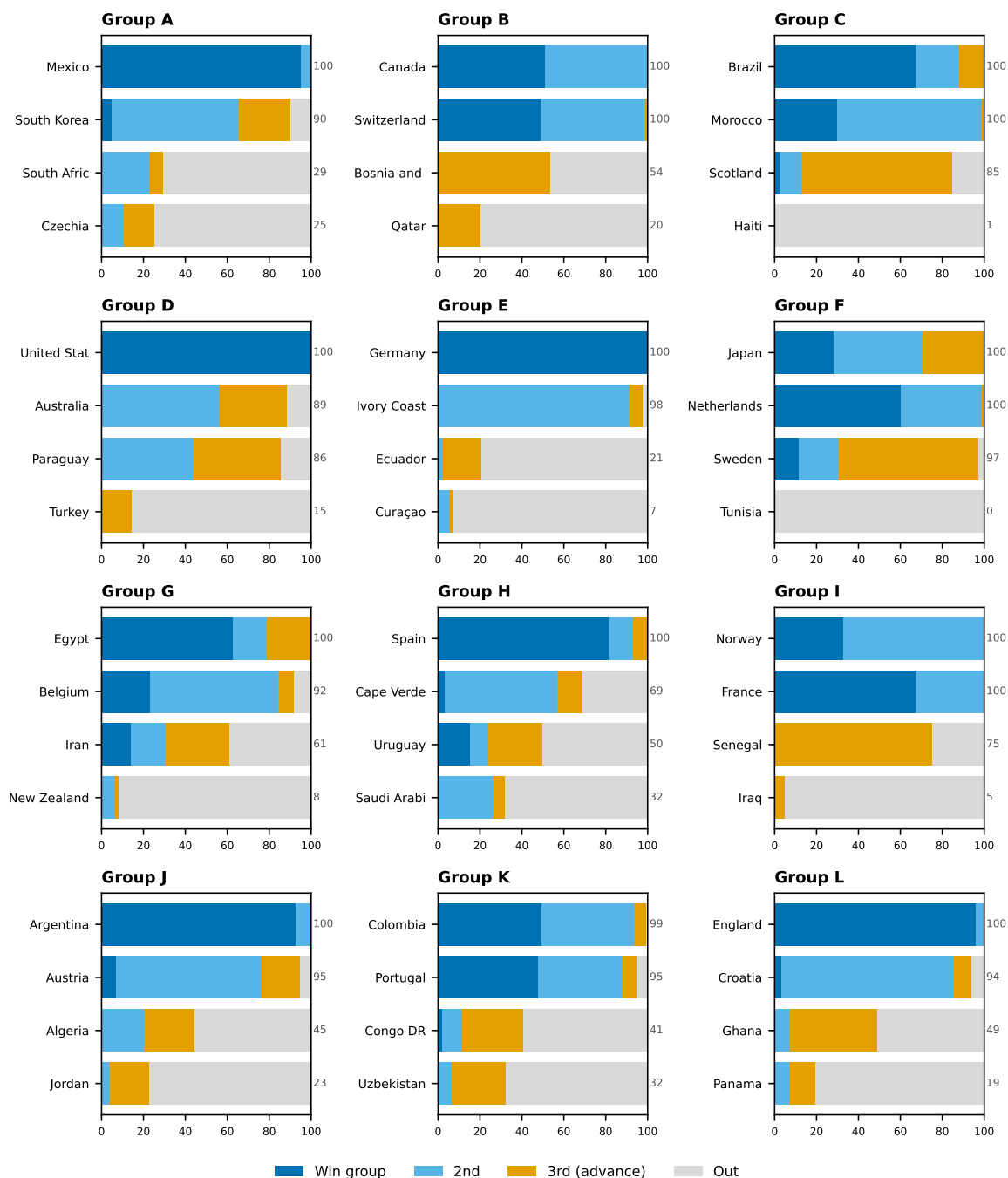
Figure 16: Qualification probability by team — Track A (conditioned on 41 results, June 10 ratings frozen; live edition M041)
