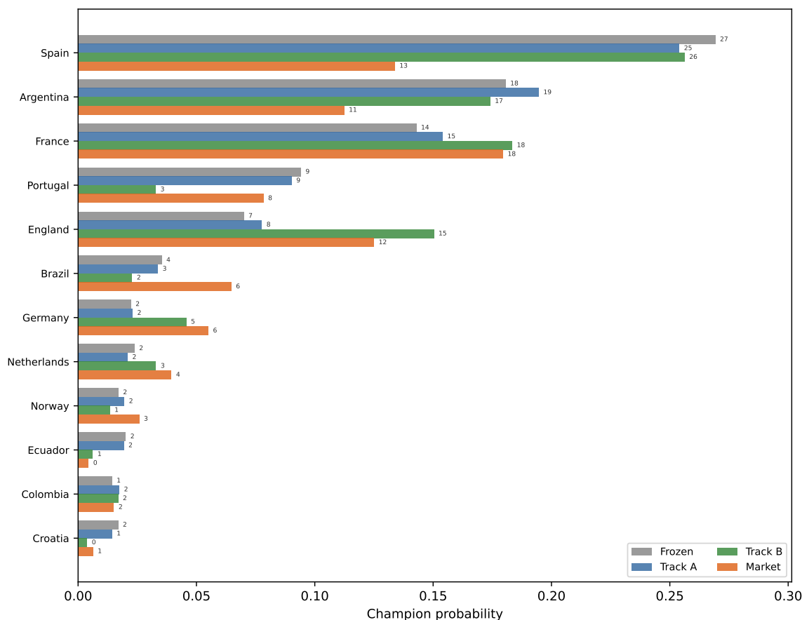
Figure 4: Champion probability, four ways: Frozen / Track A / Track B / Market, top twelve teams (live edition M024)
