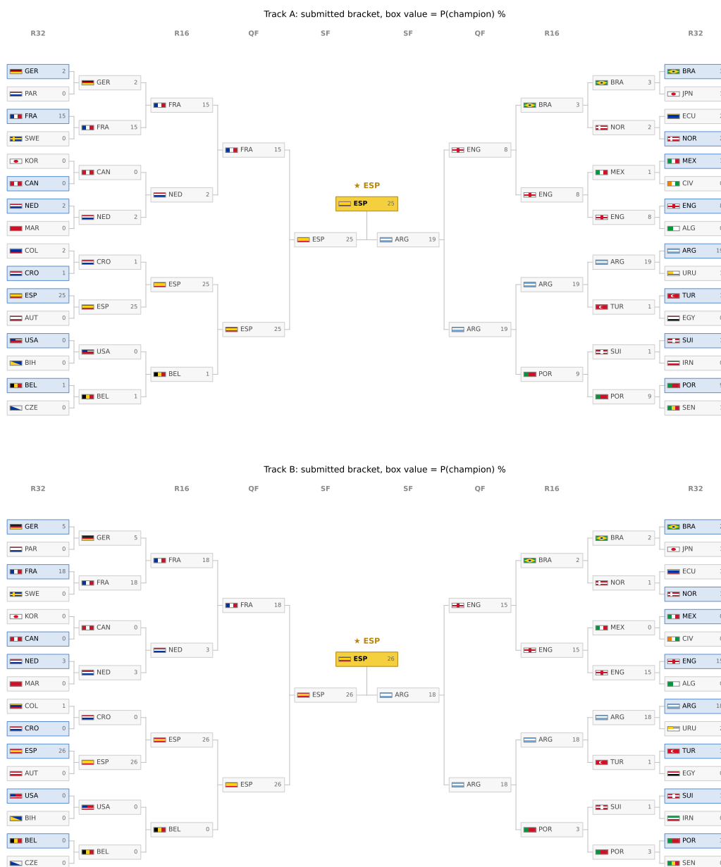
Figure 19: The submitted bracket re-valued by champion probability under Track A (top) and Track B (bottom) at live edition M024; the gold box is each track's most likely champion and greyed boxes are teams eliminated by confirmed results. The locked submitted bracket is Figure 18.
