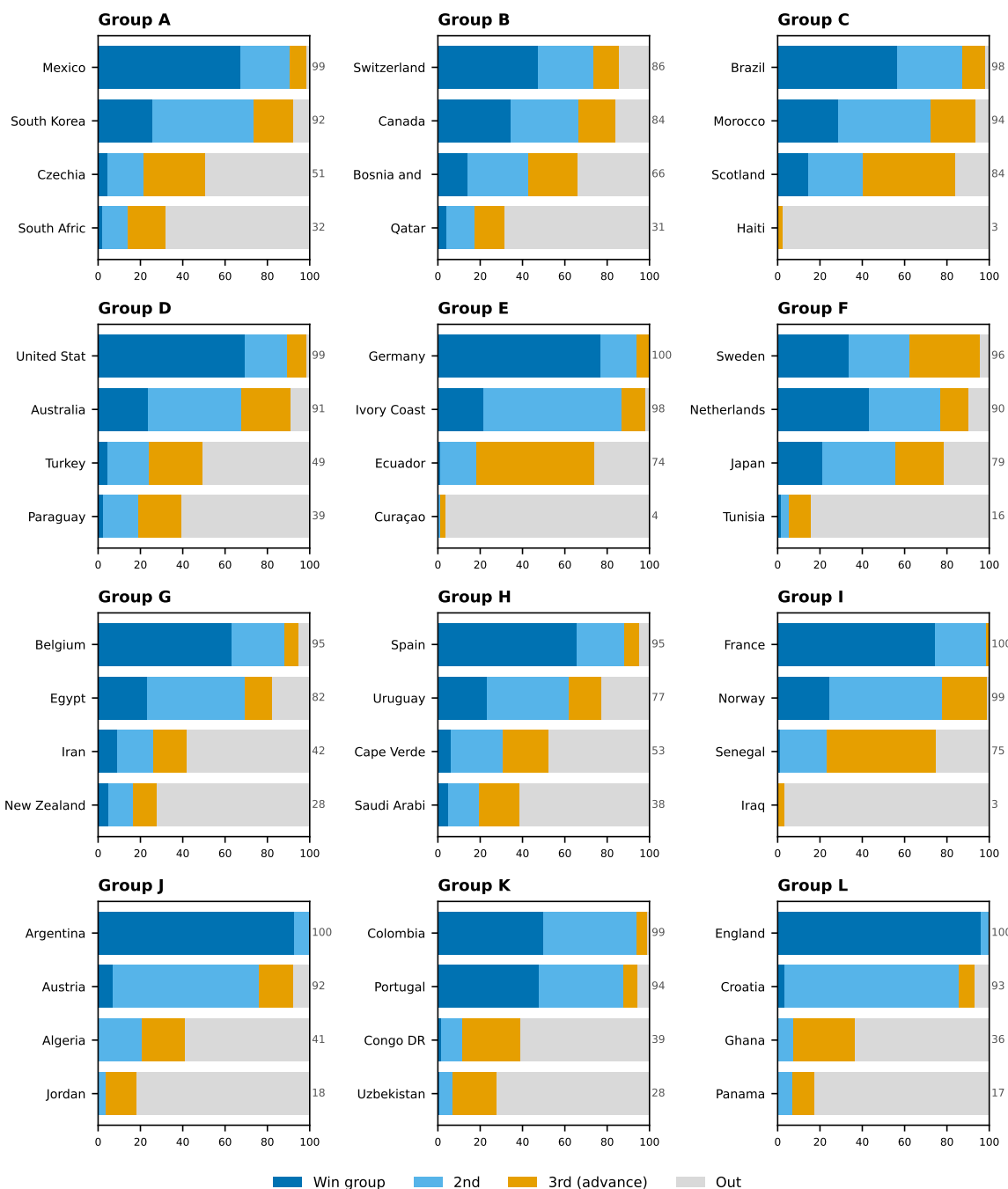
Figure 16: Qualification probability by team — Track A (conditioned on 24 results, June 10 ratings frozen; live edition M024)
