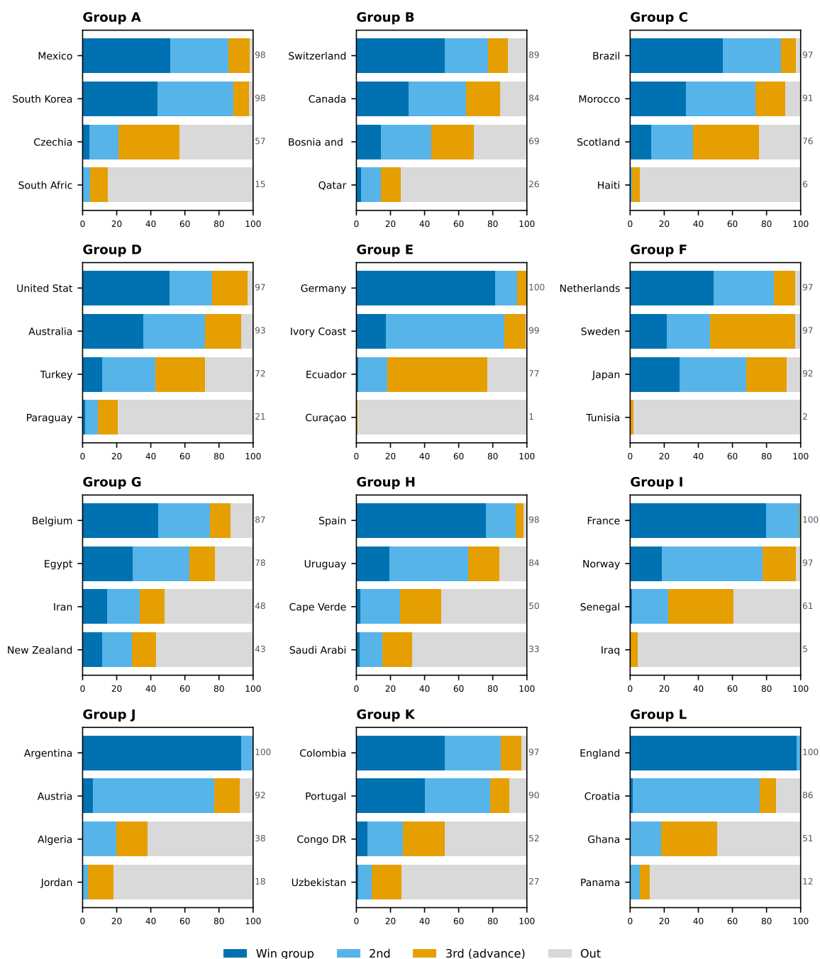
Figure 17: Qualification probability by team — Track B (result-conditioning + live Elo + bookmaker odds; live edition M024)
