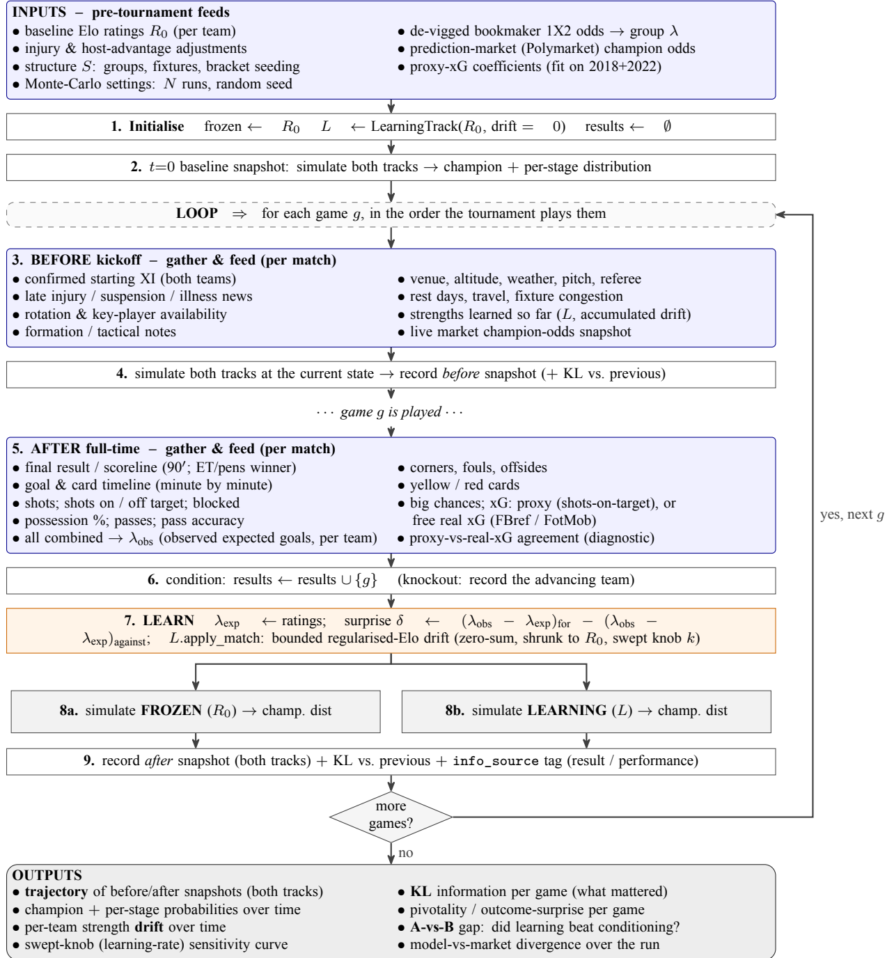
Figure 12: The two-track living-forecast procedure
