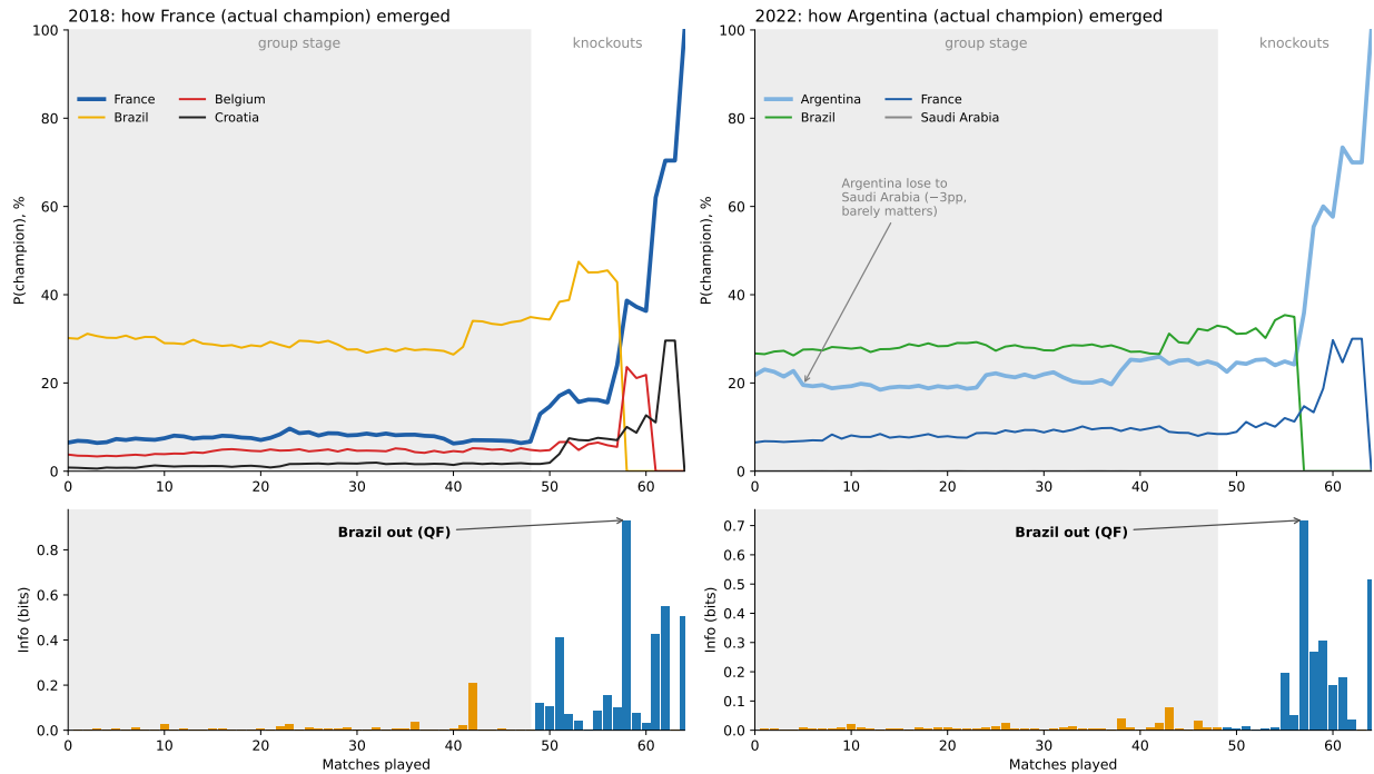
Figure 7: Forecast evolution on 2018 and 2022
