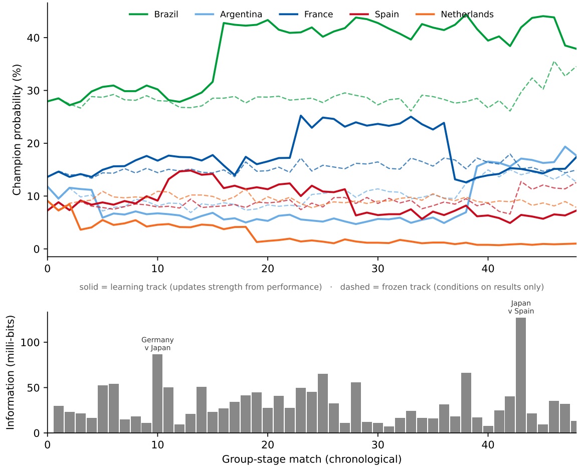
Figure 13: The 2022 group stage as a living forecast
