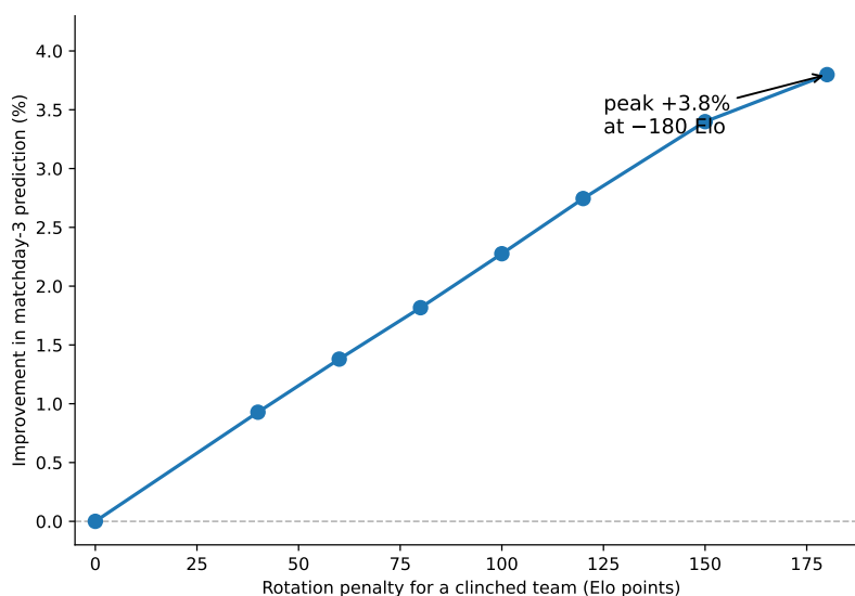
Figure 9: Rotation-aware adjustment on final matchdays
