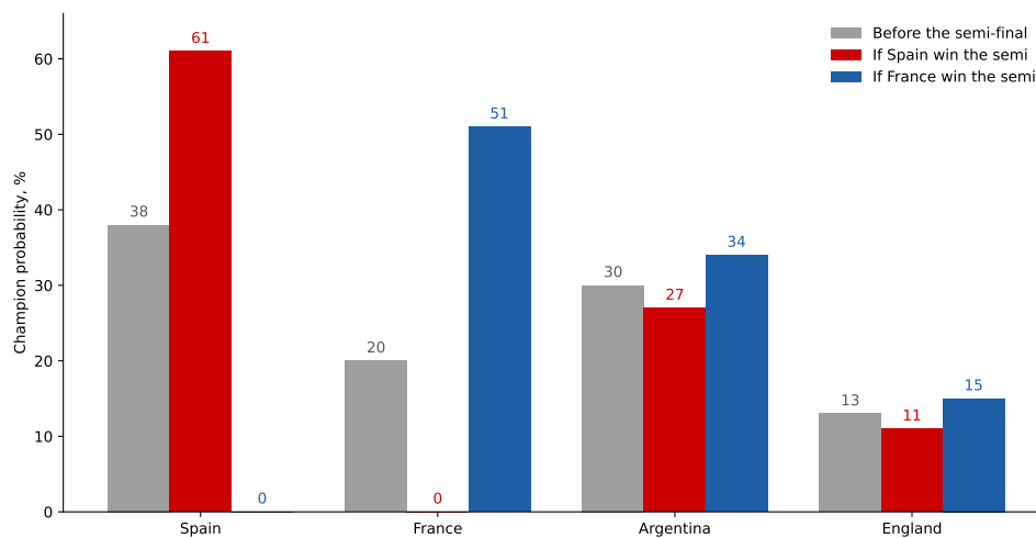
Figure 11: One match, two futures
