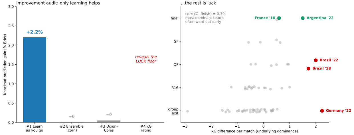
Figure 17: Candidate improvements tested on 2018 and 2022
