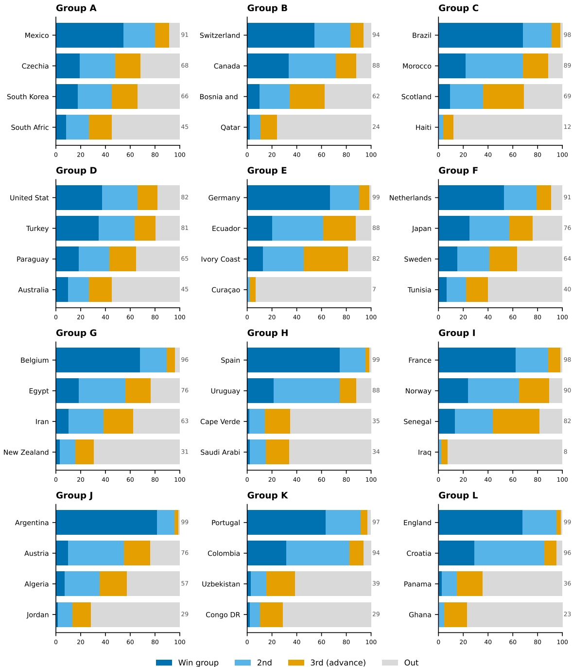
Figure 18: Qualification probability by team
