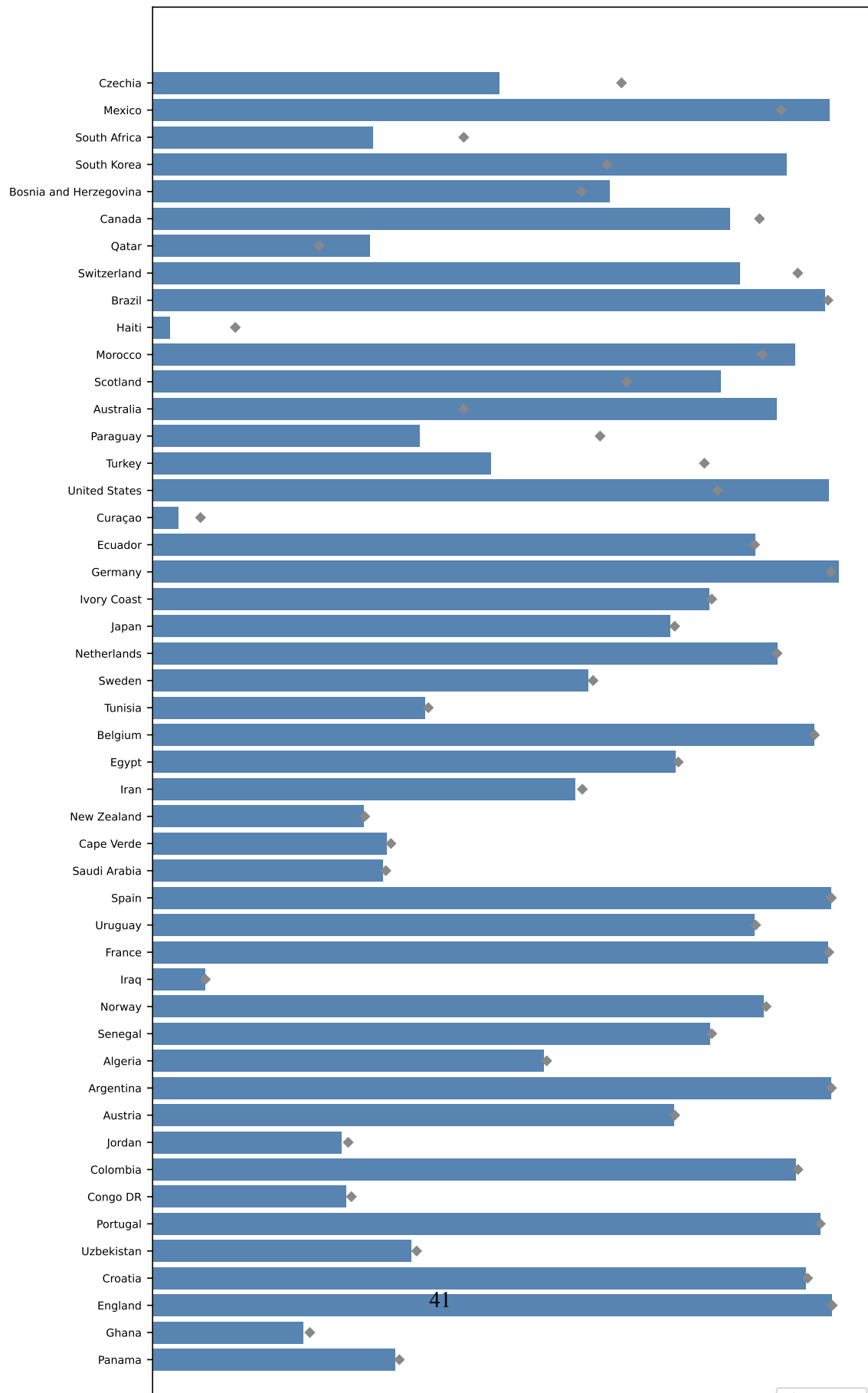
Figure 19: Qualification probability by team — Track A (conditioned on 9 results, June 10 ratings frozen; live edition MM010)
