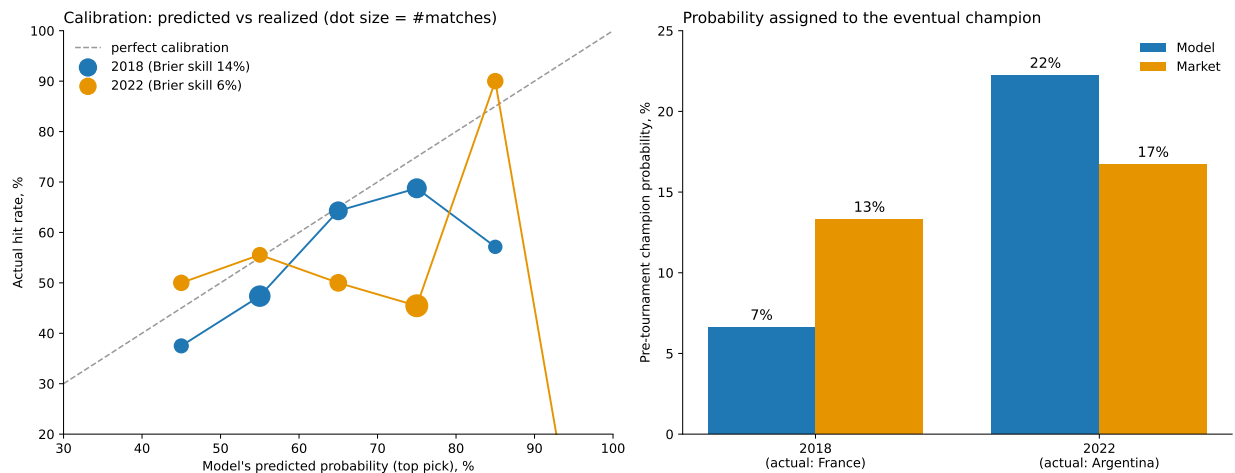
Figure 8: Out-of-sample sanity check on 2018 and 2022
