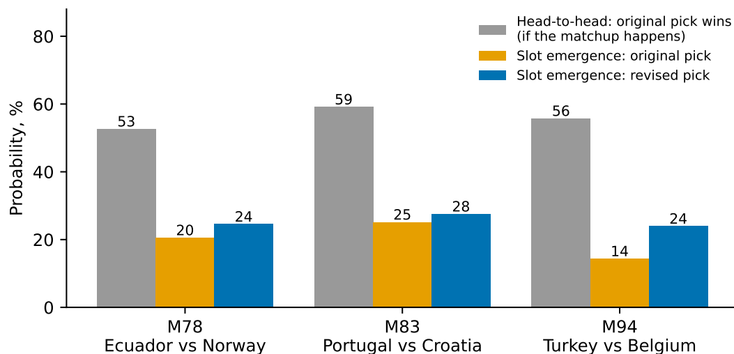
Figure 16: Head-to-head strength versus slot emergence
