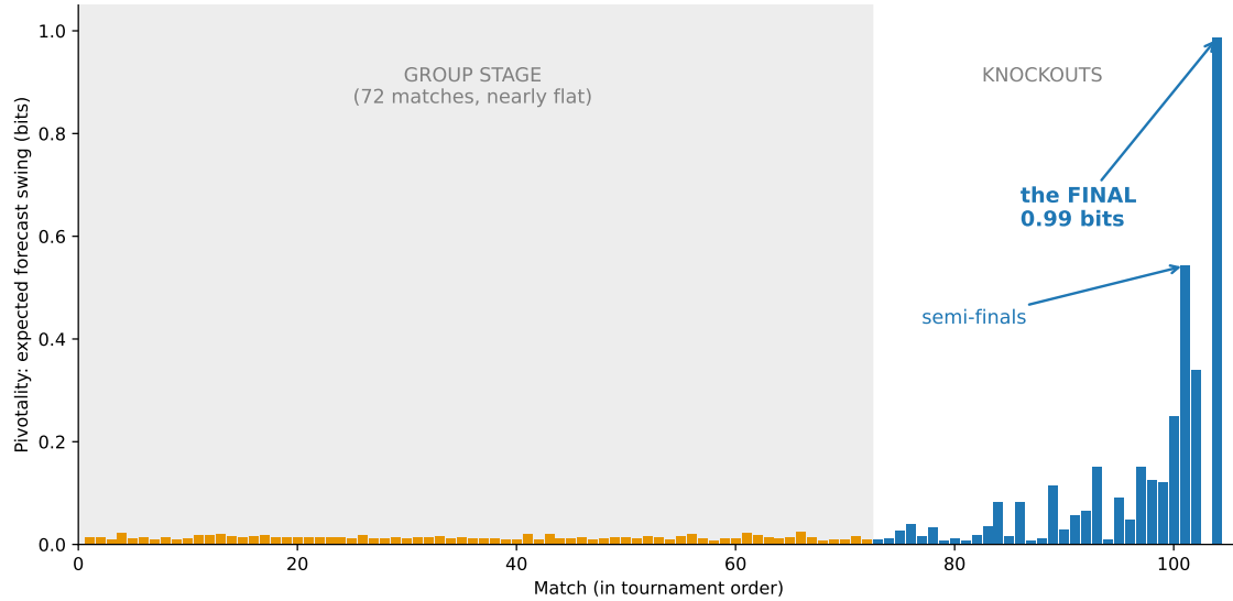
Figure 10: Pivotality along the predicted path
