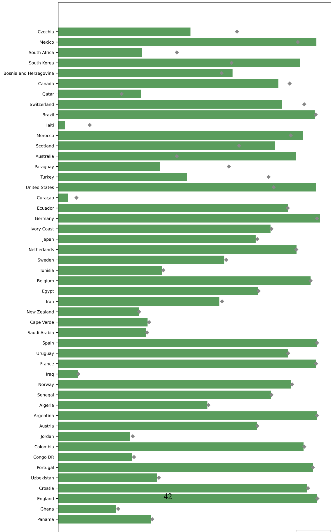
Figure 20: Qualification probability by team — Track B (result-conditioning + live Elo + bookmaker odds; live edition MM010)
