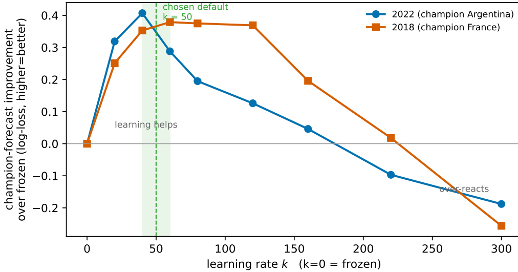
Figure 22: Learning-rate sweep on two World Cups
