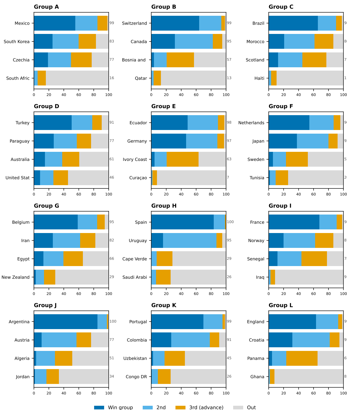
Figure 18: Qualification probability by team — Track B (result-conditioning + live Elo + bookmaker odds; live edition M001)
