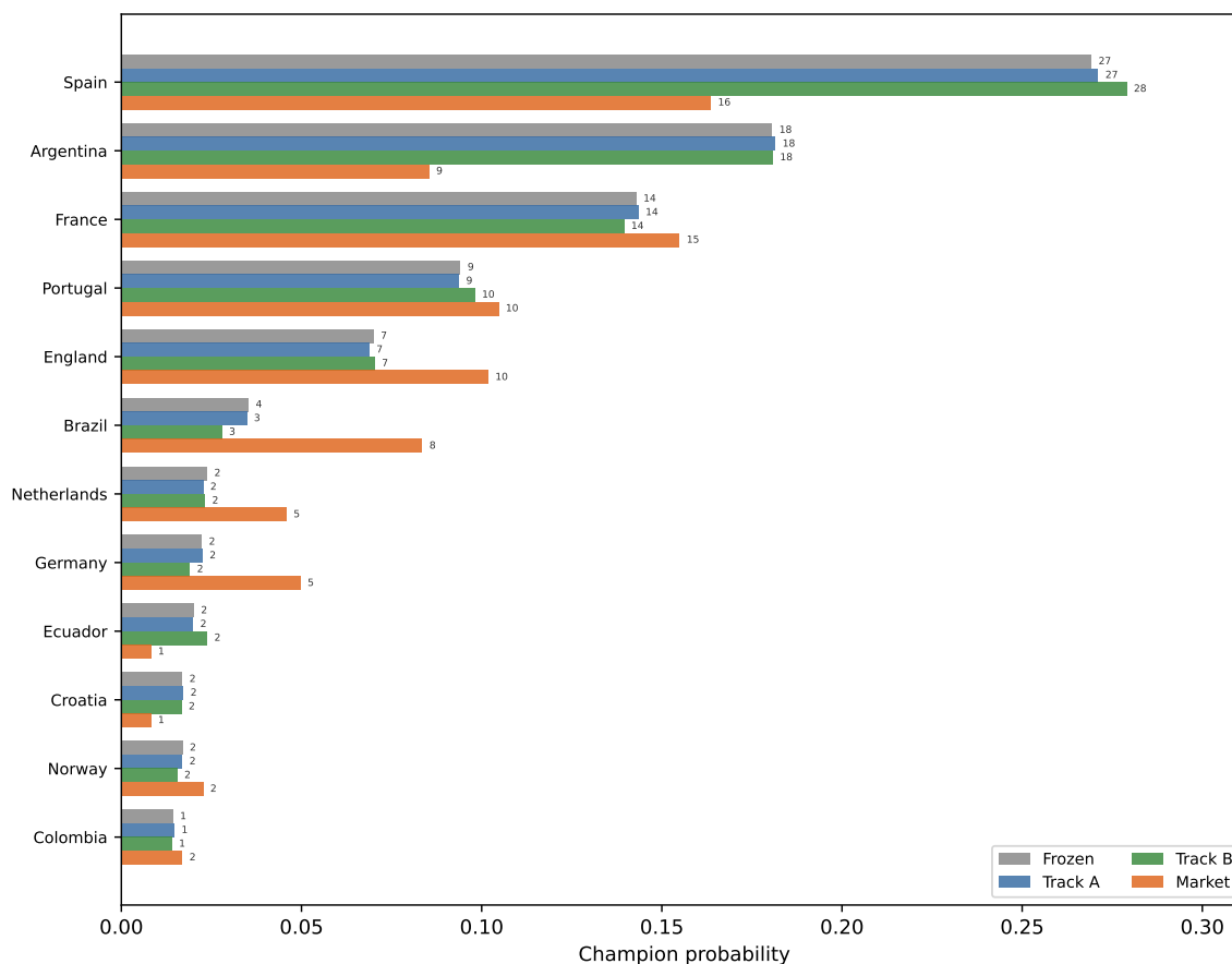
Figure 4: Champion probability, four ways: Frozen / Track A / Track B / Market, top twelve teams (live edition M001)
