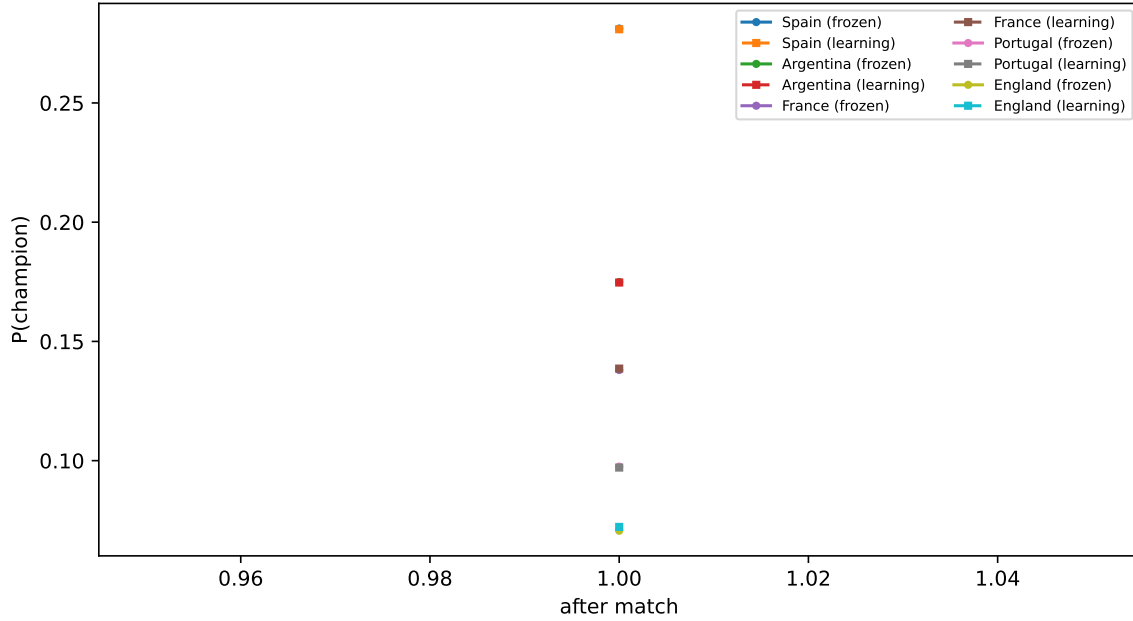
Figure 12: Two tracks live: Frozen vs Track A vs Track B champion paths
