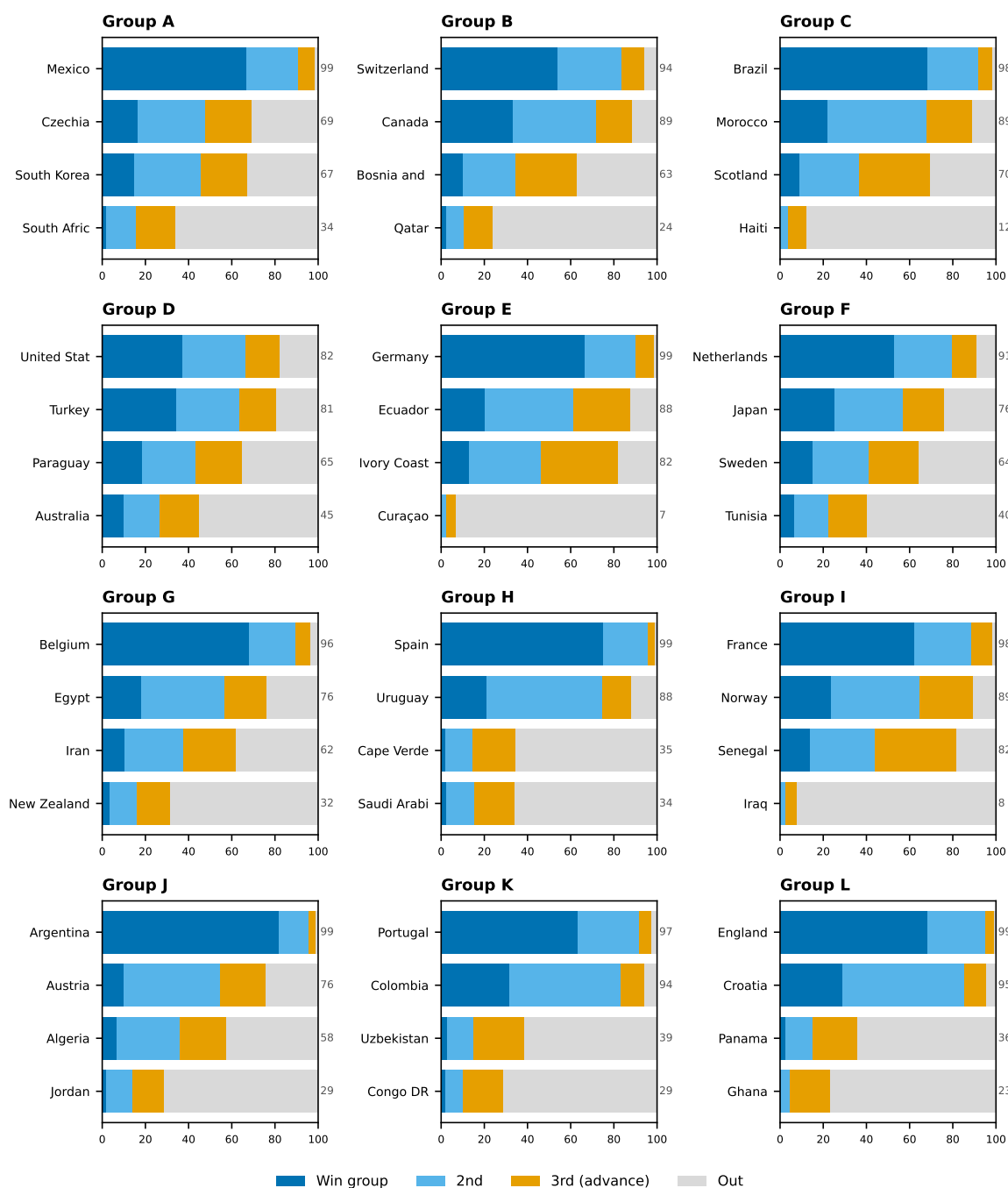
Figure 17: Qualification probability by team — Track A (conditioned on 1 results, June 10 ratings frozen; live edition M001)
