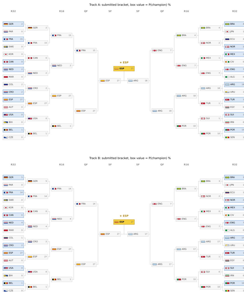
Figure 20: The submitted bracket re-valued by champion probability under Track A (top) and Track B (bottom) at live edition M009; the gold box is each track's most likely champion and greyed boxes are teams eliminated by confirmed results. The locked submitted bracket is Figure 19.
