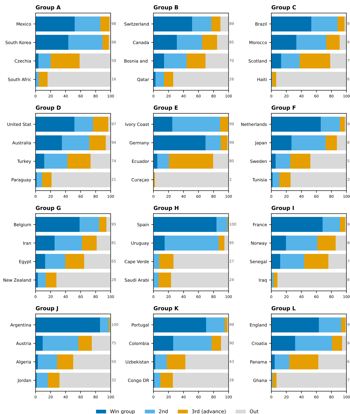
Figure 18: Qualification probability by team — Track B (result-conditioning + live Elo + bookmaker odds; live edition M009)
