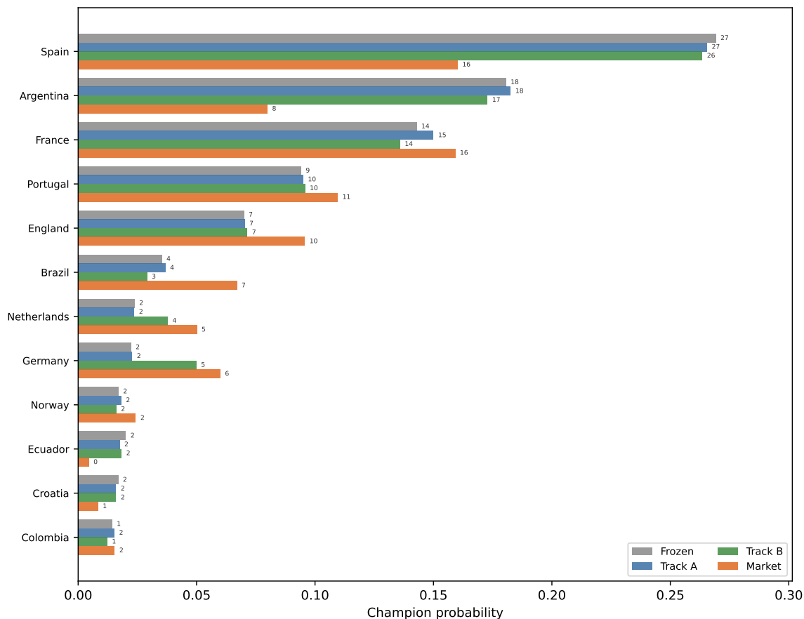
Figure 4: Champion probability, four ways: Frozen / Track A / Track B / Market, top twelve teams (live edition M009)
