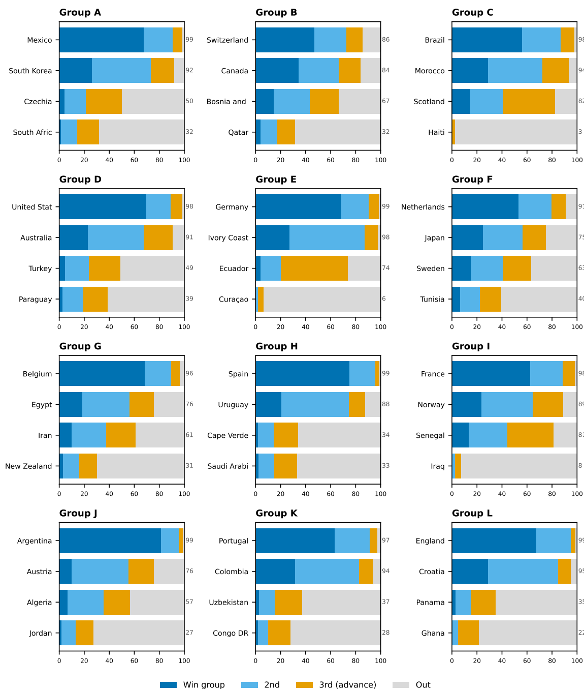
Figure 17: Qualification probability by team — Track A (conditioned on 9 results, June 10 ratings frozen; live edition M009)
