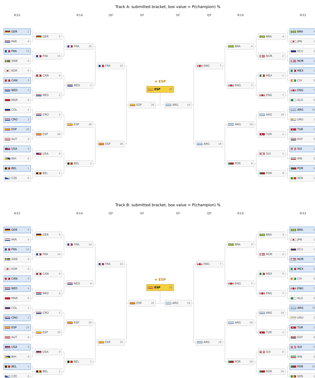
Figure 20: The submitted bracket re-valued by champion probability under Track A (top) and Track B (bottom) at live edition M015; the gold box is each track's most likely champion and greyed boxes are teams eliminated by confirmed results. The locked submitted bracket is Figure 19.
