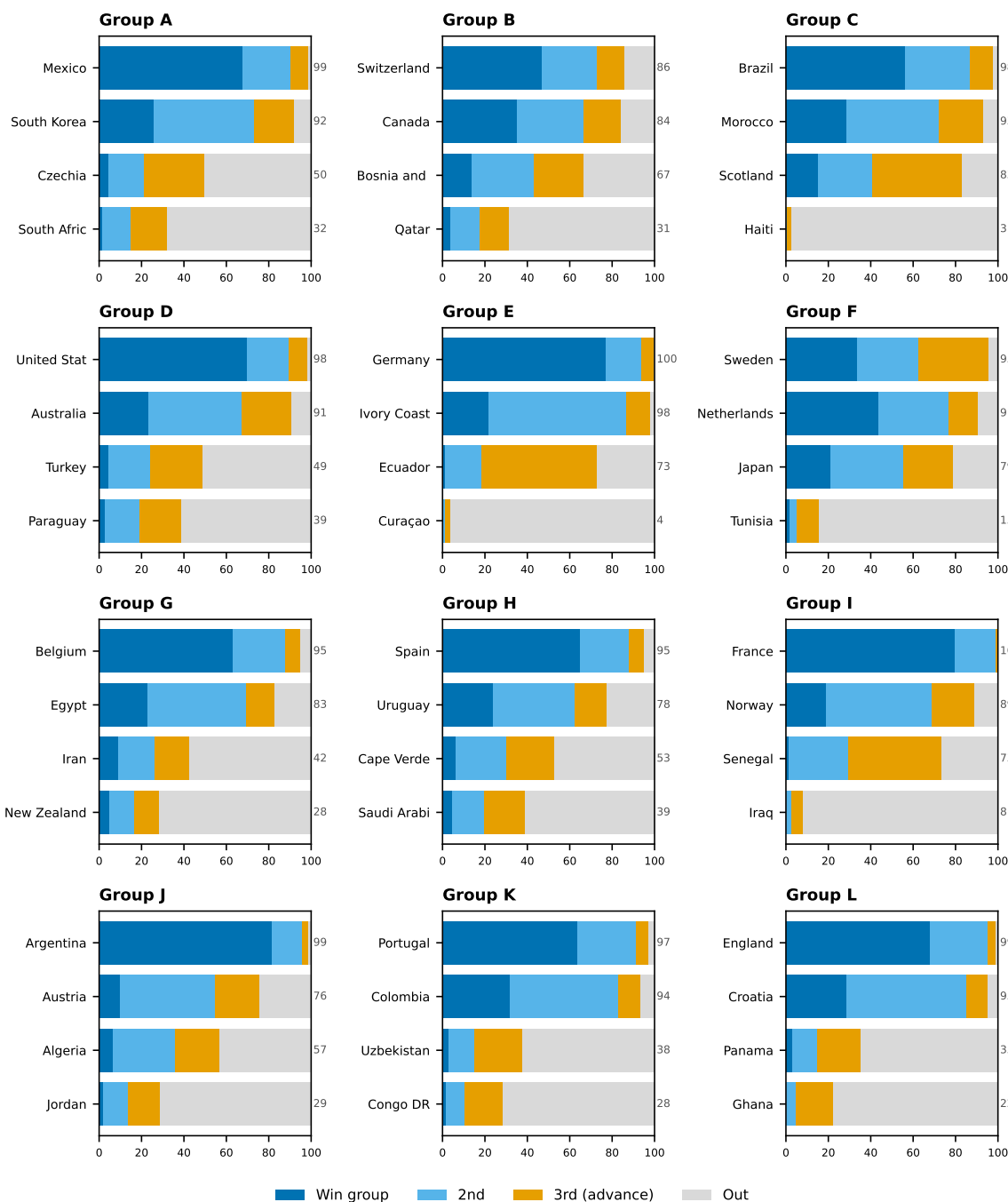
Figure 17: Qualification probability by team — Track A (conditioned on 17 results, June 10 ratings frozen; live edition M017)
