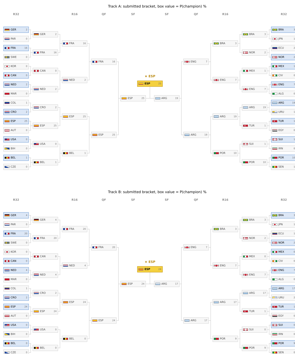
Figure 20: The submitted bracket re-valued by champion probability under Track A (top) and Track B (bottom) at live edition M017; the gold box is each track's most likely champion and greyed boxes are teams eliminated by confirmed results. The locked submitted bracket is Figure 19.
