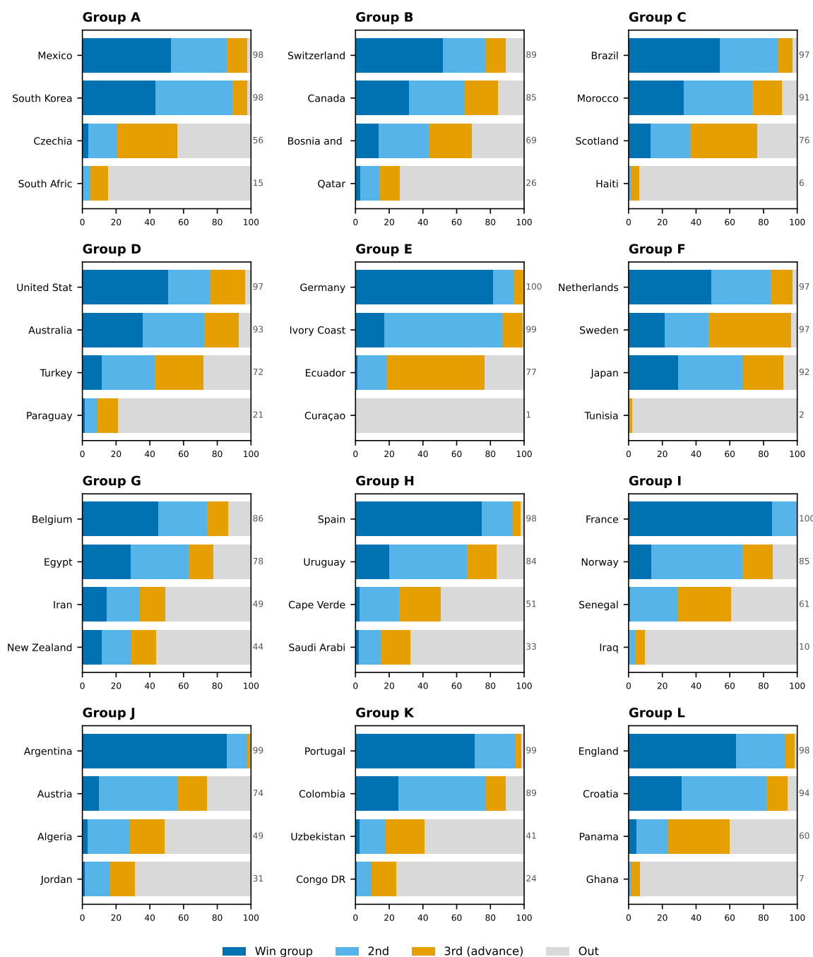
Figure 18: Qualification probability by team — Track B (result-conditioning + live Elo + bookmaker odds; live edition M017)
