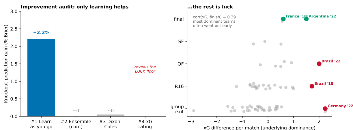
Figure 14: Candidate improvements tested on 2018 and 2022. Left: in-tournament updating improves knockout prediction; forecast combination did not help on this sample; the Dixon–Coles correction, judged on realized points rather than likelihood, gives a small in-sample gain (a fifth test, penalty-shootout temperament, showed no predictive signal and is discussed in the text). Right: expected-goal difference against the stage each team reached, with the correlation only 0.39. The most dominant teams (Brazil, Germany, in red) often went out early, so much of the model’s residual error is the irreducible randomness of football rather than missing information.
