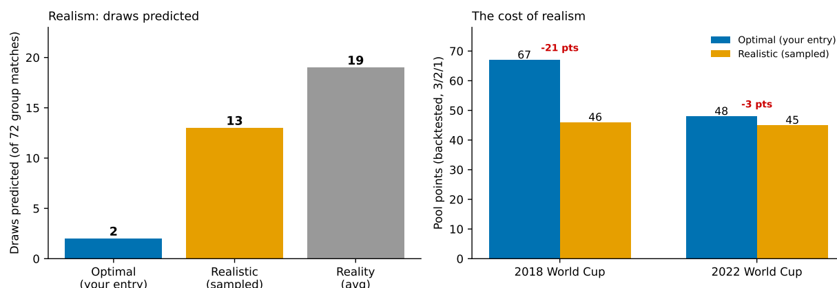
Figure 12: The optimal entry against a realistic, draw-producing alternative that samples each scoreline from its distribution. Left: draws predicted on the 2026 group stage, against the real-tournament average. Right: pool points on the 2018 and 2022 backtests, where the optimal entry scores more in both years, by 31 percent in the orderly 2018 tournament and 6 percent in the upset-heavy 2022 tournament.
