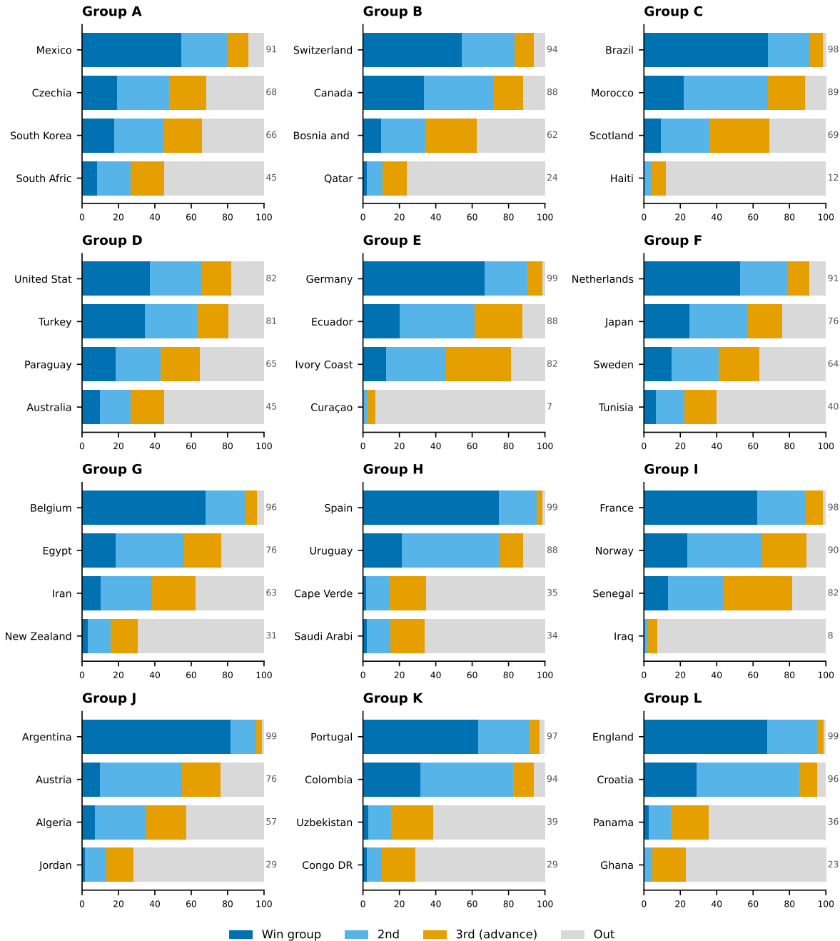
Figure 15: Qualification probability by team across 100,000 simulations. Dark blue is the probability of winning the group, light blue of finishing second, orange of advancing as one of the eight best third-placed teams, and grey of elimination. The number at each bar is the total qualification probability.
