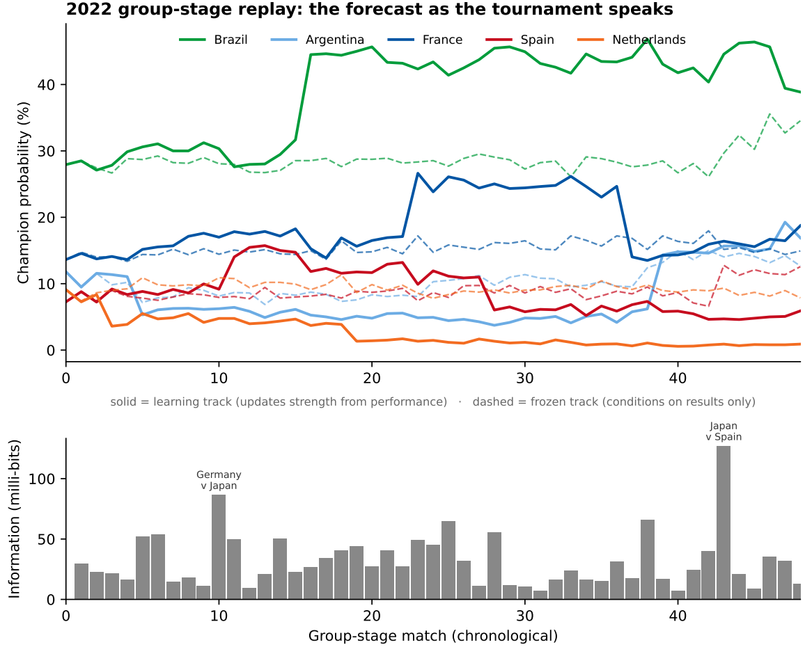
Figure 11: The 2022 World Cup group stage replayed as a living forecast. Top: champion probability for five contenders after each group match, under the learning track (solid, strength updated from performance) and the frozen track (dashed, results only); the learning track raises the eventual finalists Argentina and France and lowers the unconvincing group winners Netherlands and Spain. Bottom: the information each match carries (KL divergence against the previous forecast, in milli-bits), concentrated at Japan’s upsets of Germany and Spain.
