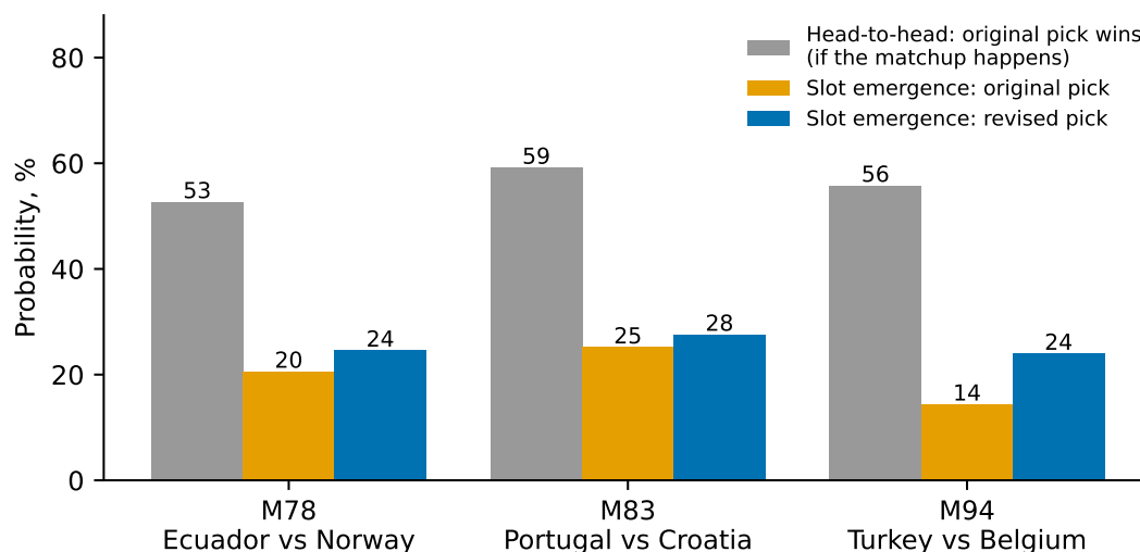
Figure 13: Head-to-head strength versus slot emergence for the three revised knockout picks. Grey: probability the original pick wins if the predicted matchup occurs (Elo). Orange/blue: probability the team actually occupies and wins the bracket slot across 200,000 simulations. All three original picks are head-to-head favorites; all three are slot-emergence underdogs.
