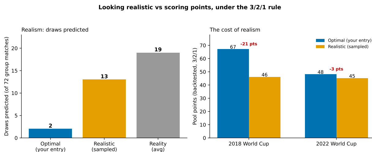
Figure 13: The optimal entry against a realistic, draw-producing alternative that samples each scoreline from its distribution. Left: draws predicted on the 2026 group stage, against the real-tournament average. Right: pool points on the 2018 and 2022 backtests, where the optimal entry scores more in both years, by 31 percent in the orderly 2018 tournament and 6 percent in the upset-heavy 2022 tournament.
