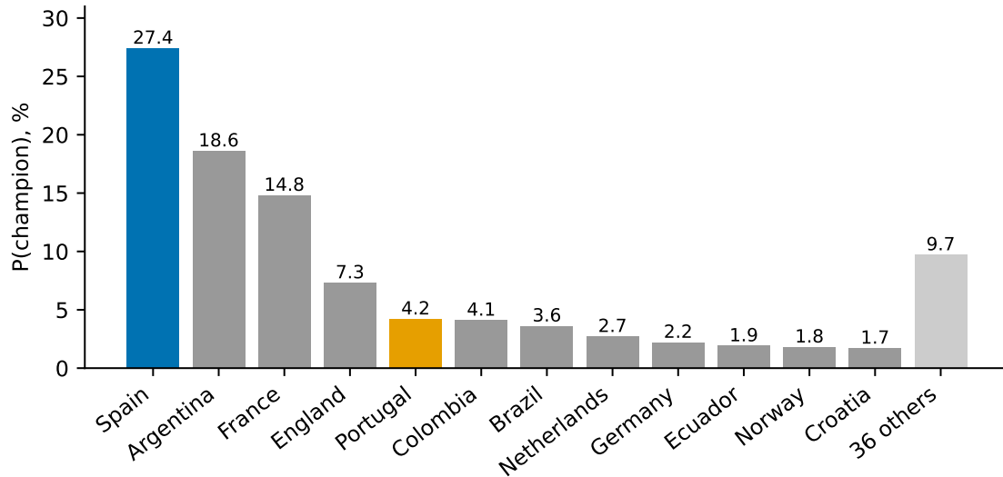
Figure 1: Champion probability distribution across 200,000 simulated tournaments. Spain (blue) is the modal champion yet fails to win in 72.6% of simulations; Portugal (orange) is discussed in Section 5.2. The 36 teams outside the top twelve jointly retain a 9.7% champion share.
