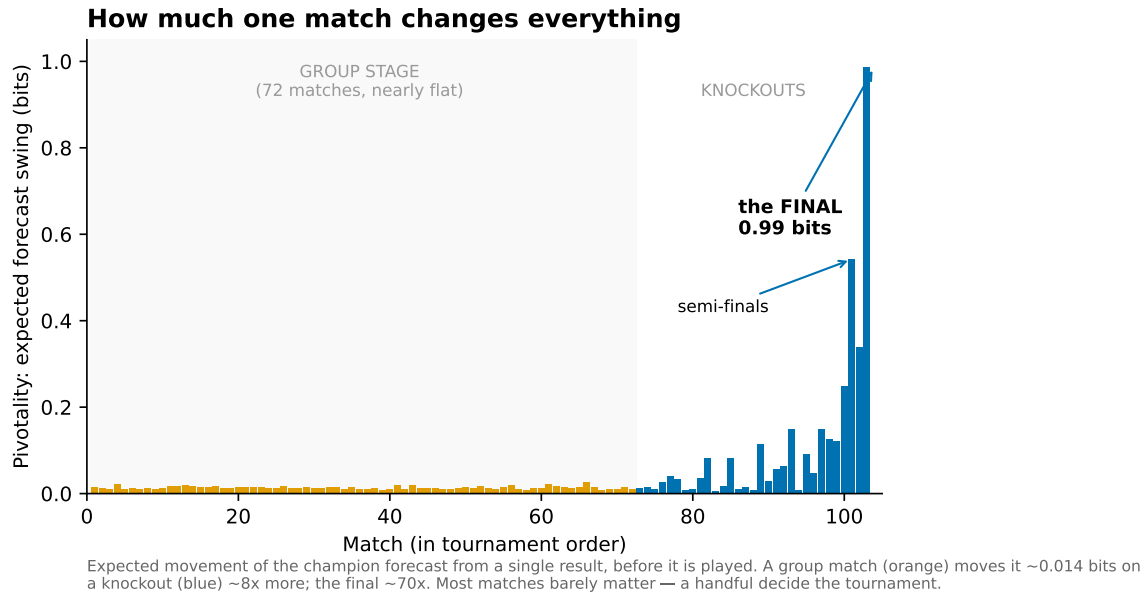
Figure 8: Pivotality of each match along the predicted path: the expected movement of the champion forecast from a single result, before it is played. Group matches (orange) average 0.014 bits; knockout matches (blue) average 0.11 bits; the final reaches 0.99 bits. Most matches barely affect who wins, and a few decide it.
