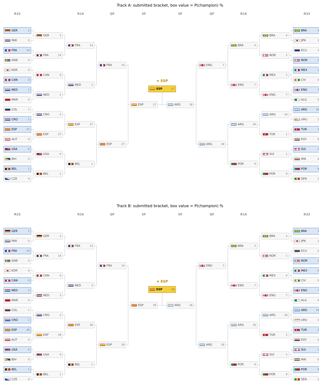
Figure 23: The submitted bracket re-valued by champion probability under Track A (top) and Track B (bottom) at live edition M002; the gold box is each track's most likely champion and greyed boxes are teams eliminated by confirmed results. The locked submitted bracket is Figure 22.
