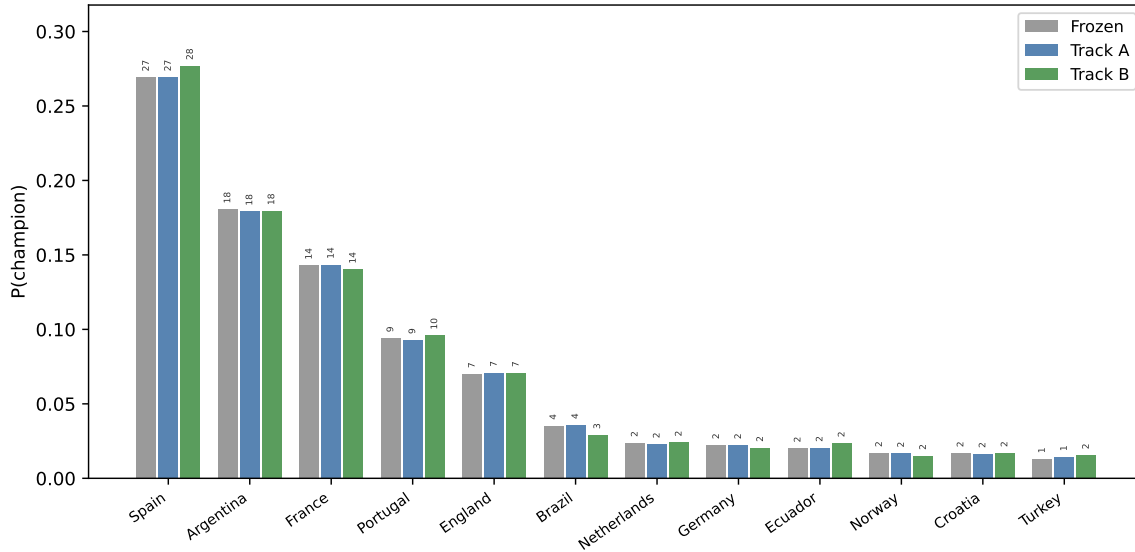
Figure 2: Champion probability distribution, conditioned on 2 results (live edition M002)
