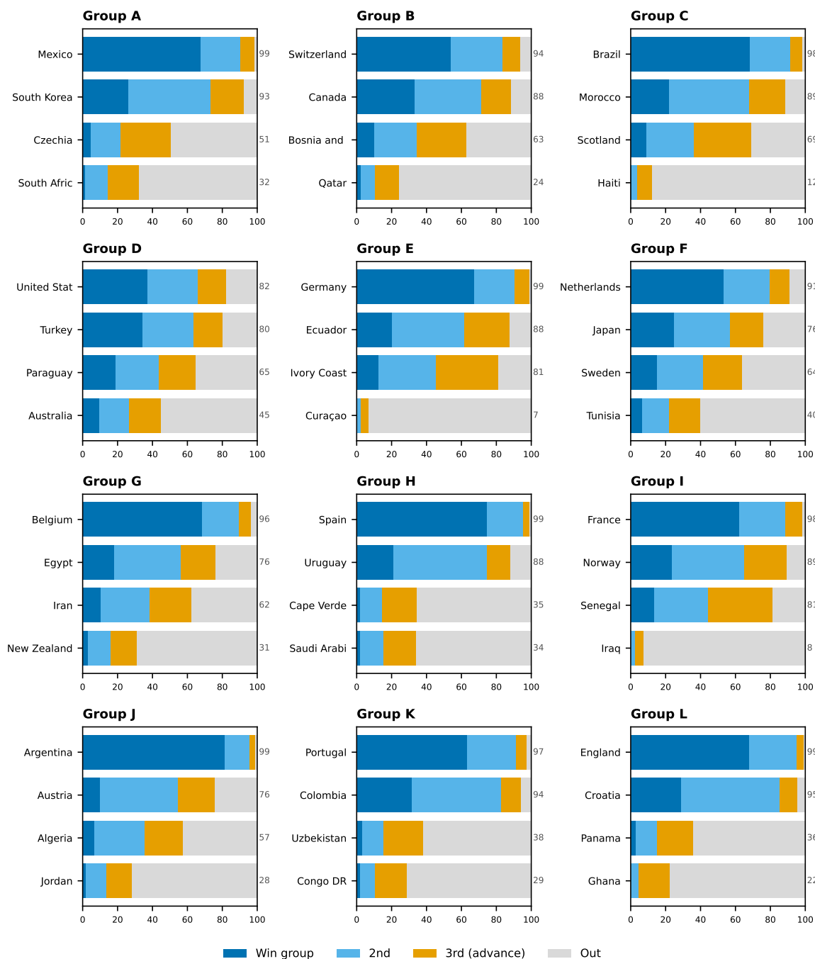
Figure 20: Qualification probability by team — Track A (conditioned on 2 results, June 10 ratings frozen; live edition M002)
