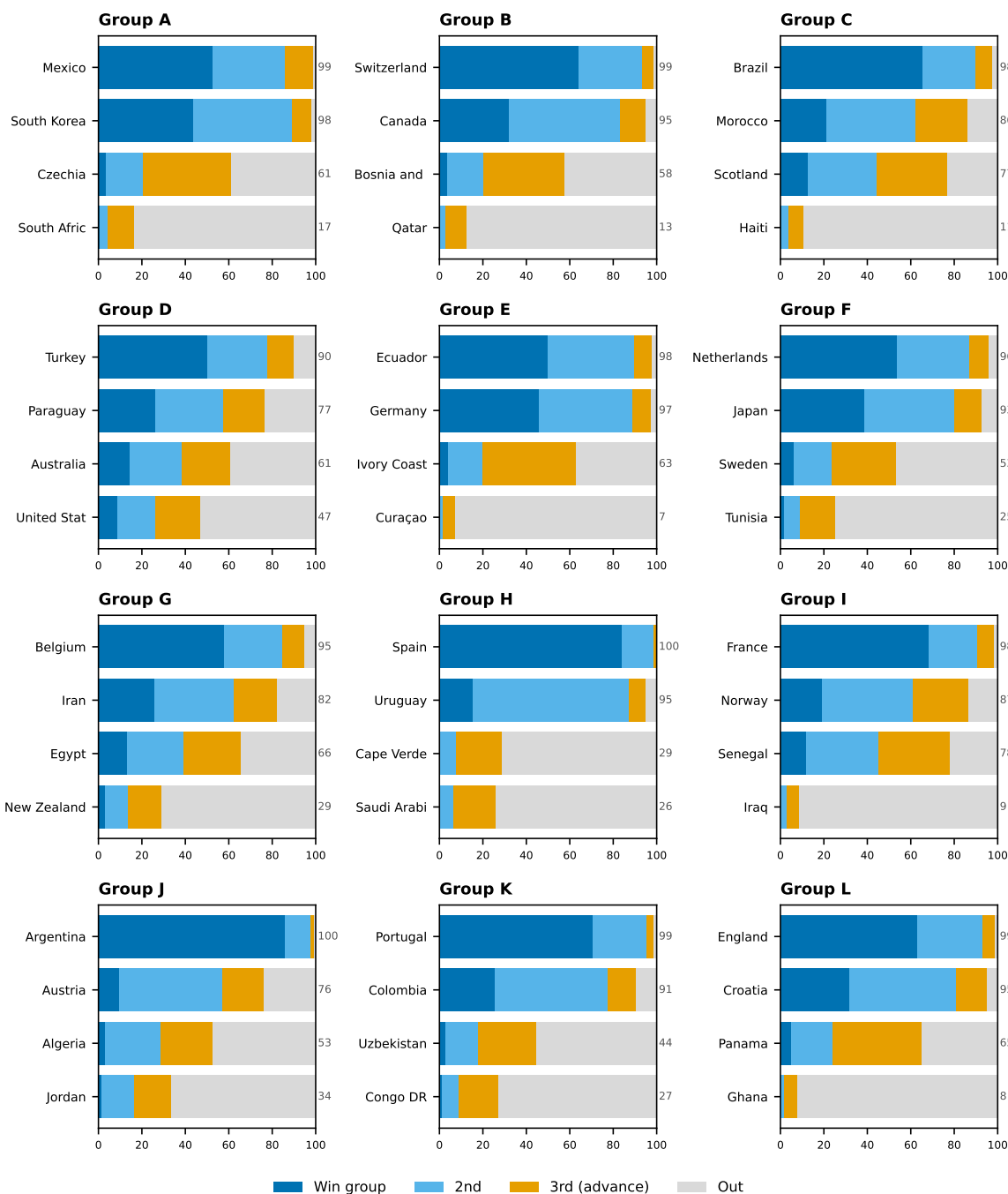
Figure 21: Qualification probability by team — Track B (result-conditioning + live Elo + bookmaker odds; live edition M002)
