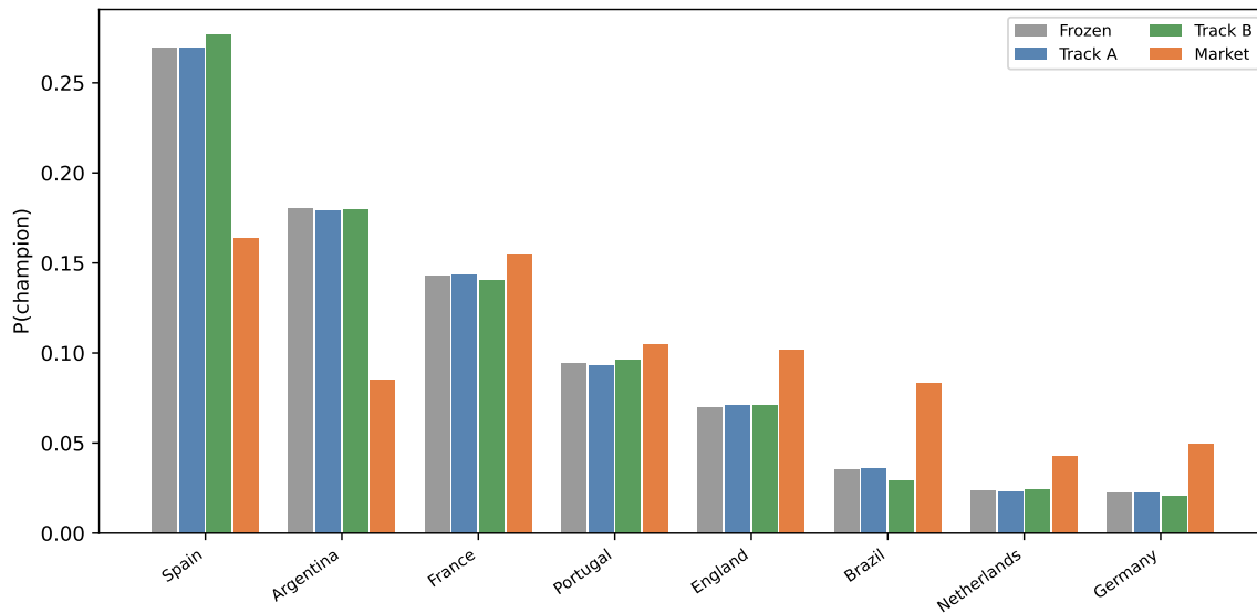
Figure 7: Four-bar champion probability: Frozen / Track A / Track B / Market, top contenders (live edition M002)
