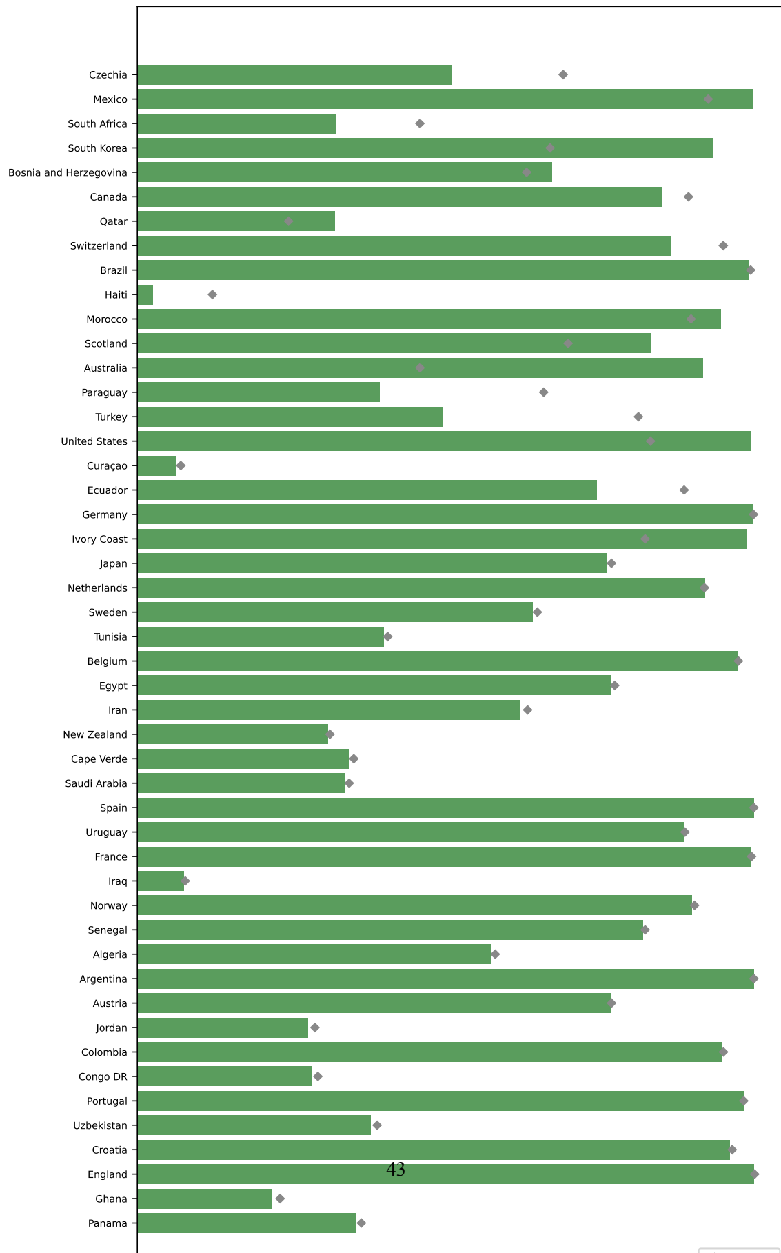
Figure 21: Qualification probability by team — Track B (result-conditioning + live Elo + bookmaker odds; live edition M009)
