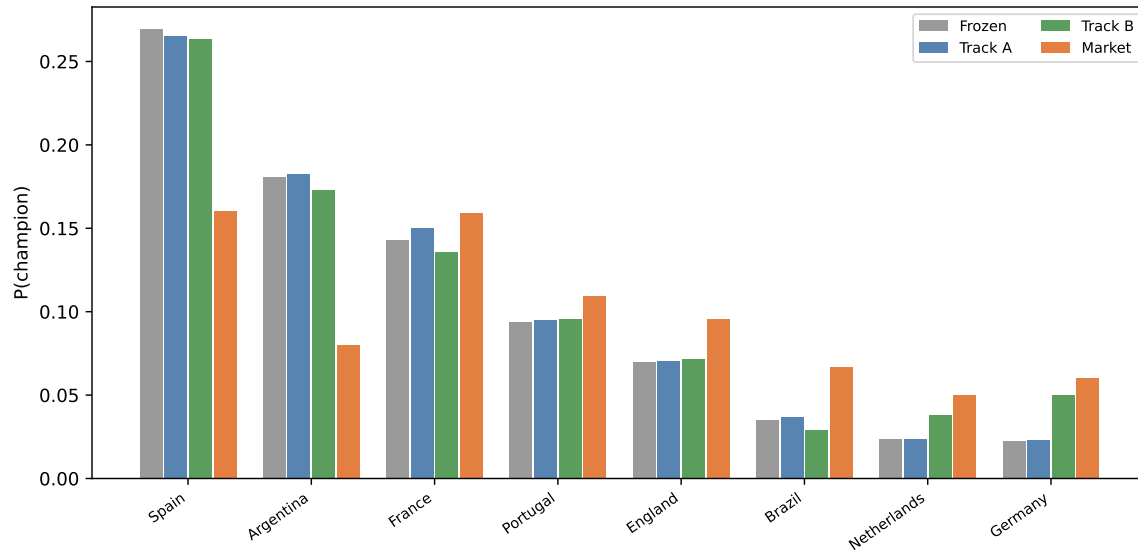
Figure 7: Four-bar champion probability: Frozen / Track A / Track B / Market, top contenders (live edition M009)
