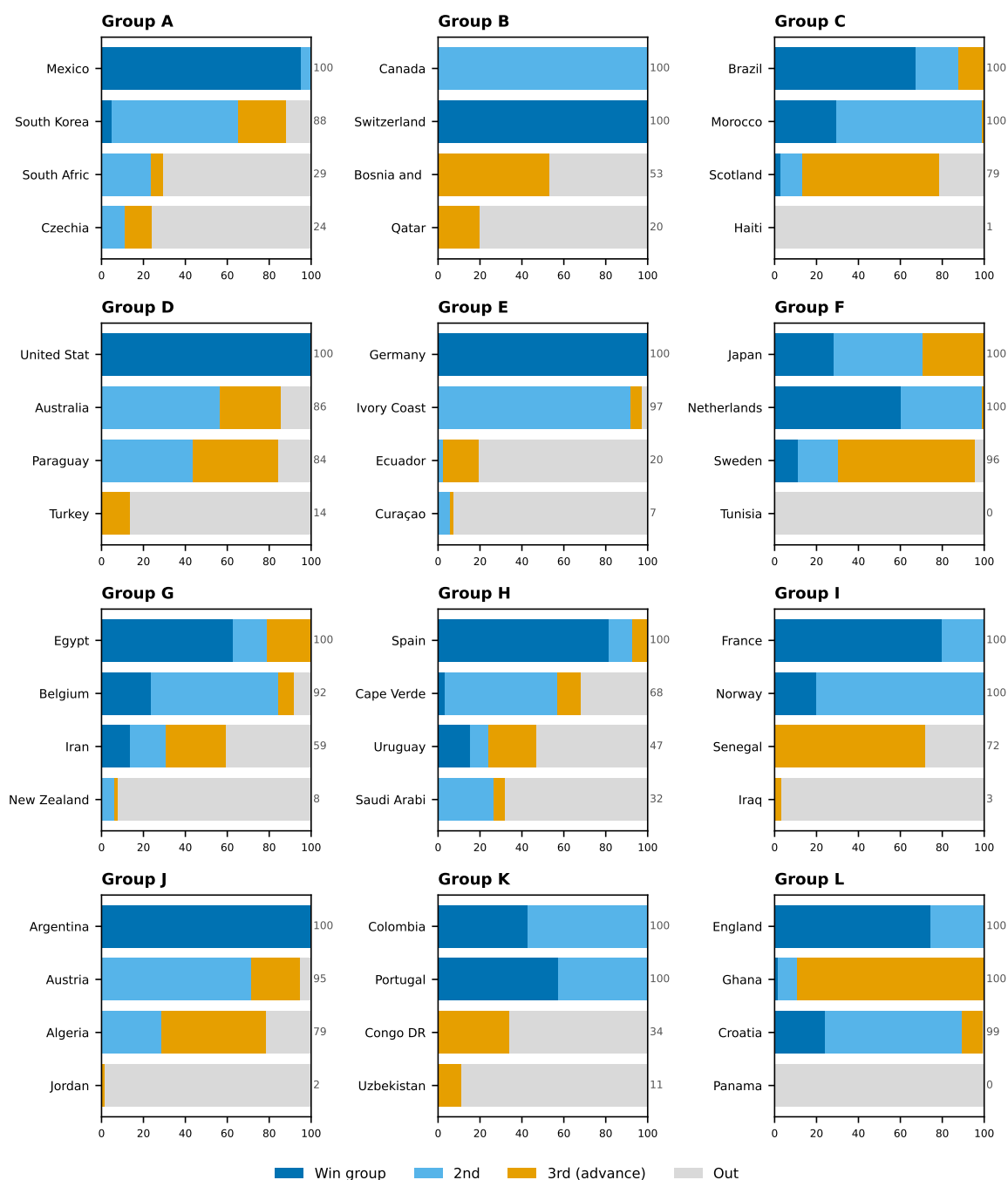
Figure 16: Qualification probability by team — Track A (conditioned on 49 results, June 10 ratings frozen; live edition M051)
