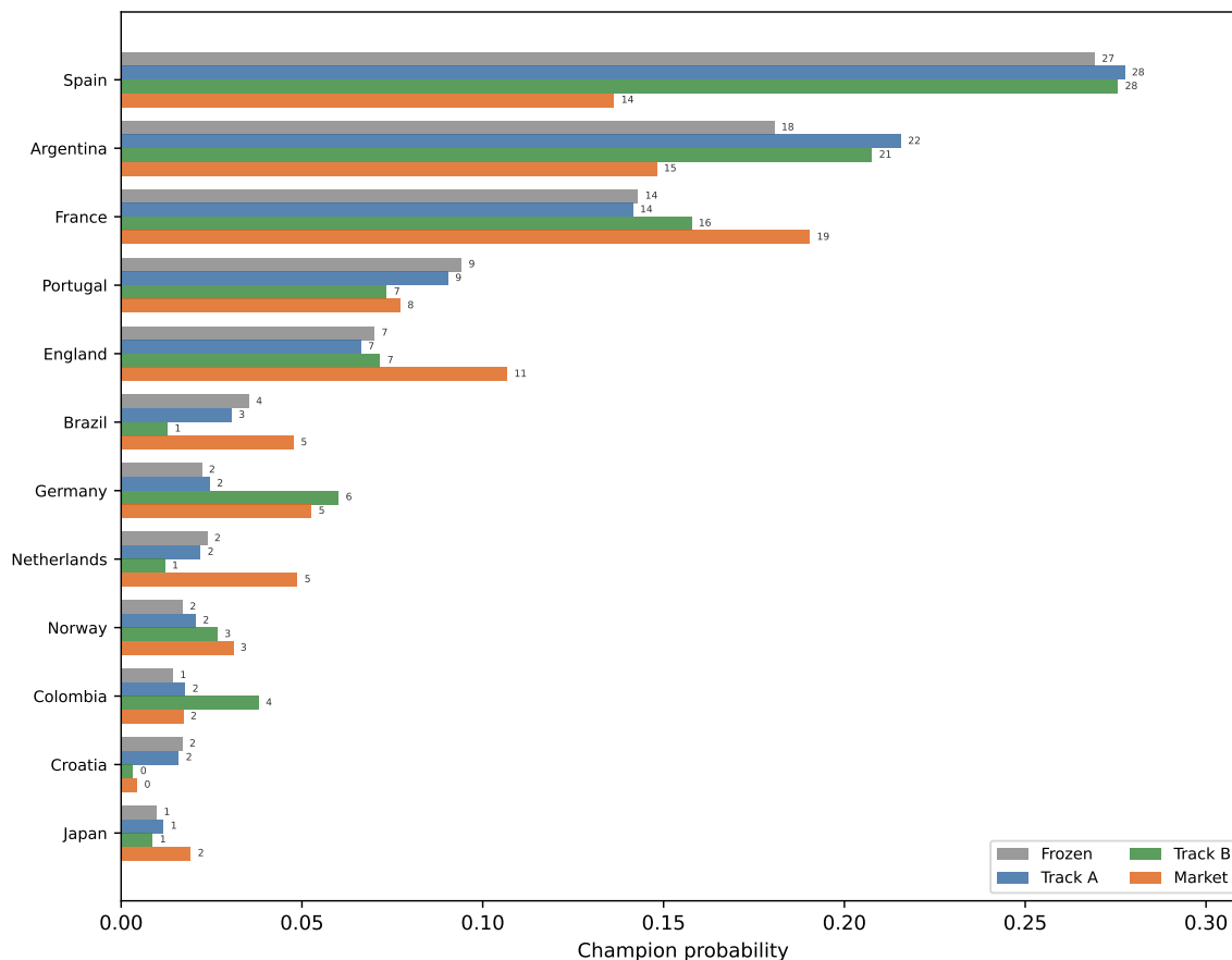
Figure 4: Champion probability, four ways: Frozen / Track A / Track B / Market, top twelve teams (live edition M051)
