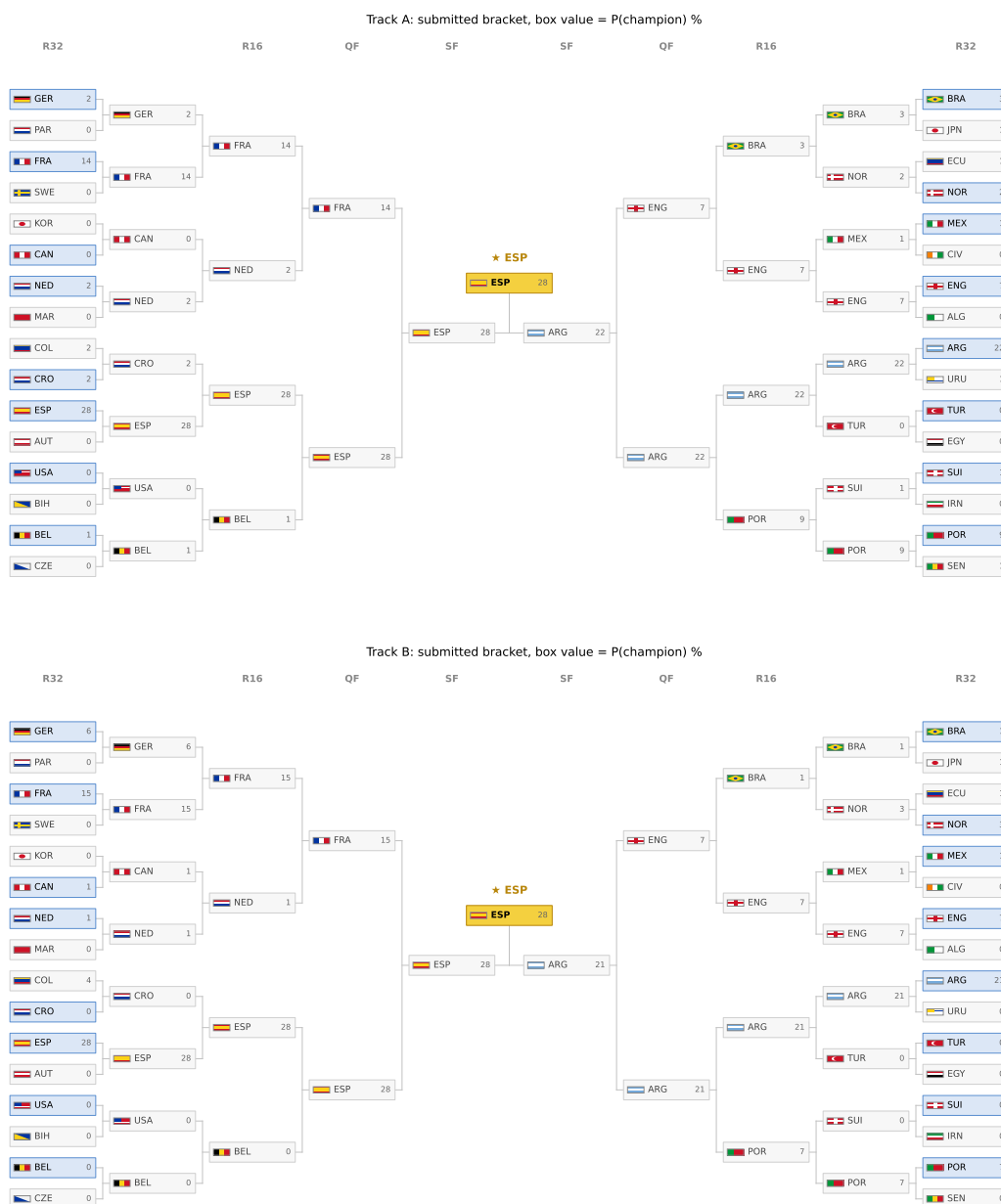
Figure 19: The submitted bracket re-valued by champion probability under Track A (top) and Track B (bottom) at live edition M051; the gold box is each track's most likely champion and greyed boxes are teams eliminated by confirmed results. The locked submitted bracket is Figure 18.
