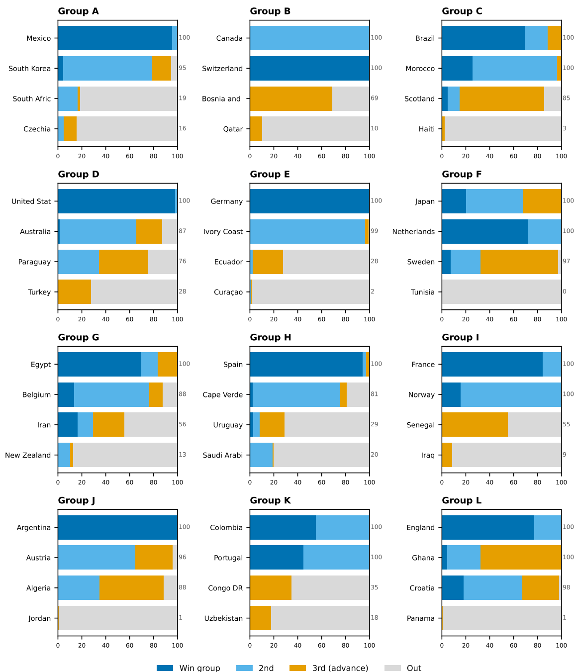
Figure 17: Qualification probability by team — Track B (result-conditioning + live Elo + bookmaker odds; live edition M051)
