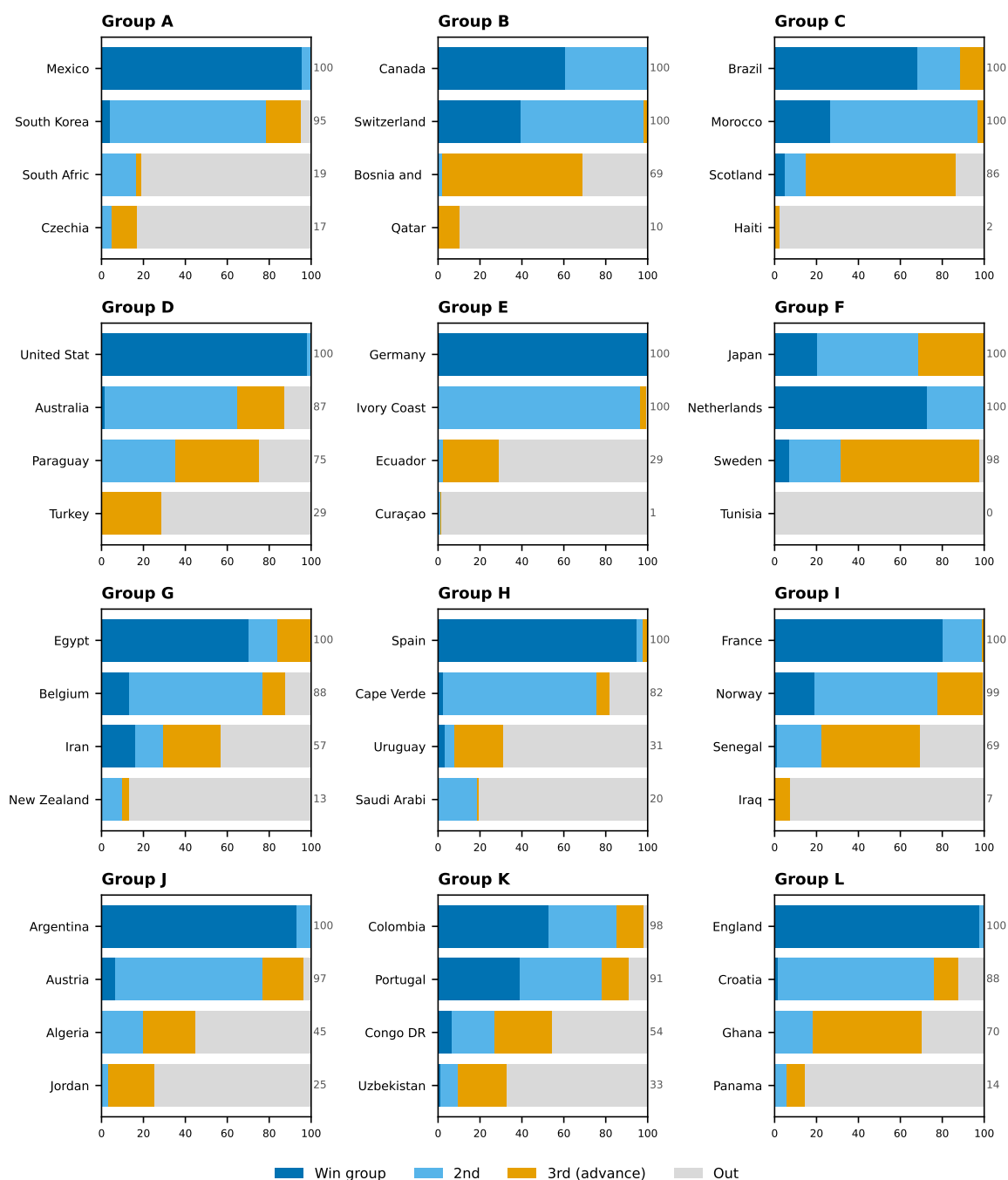
Figure 17: Qualification probability by team — Track B (result-conditioning + live Elo + bookmaker odds; live edition M040)
