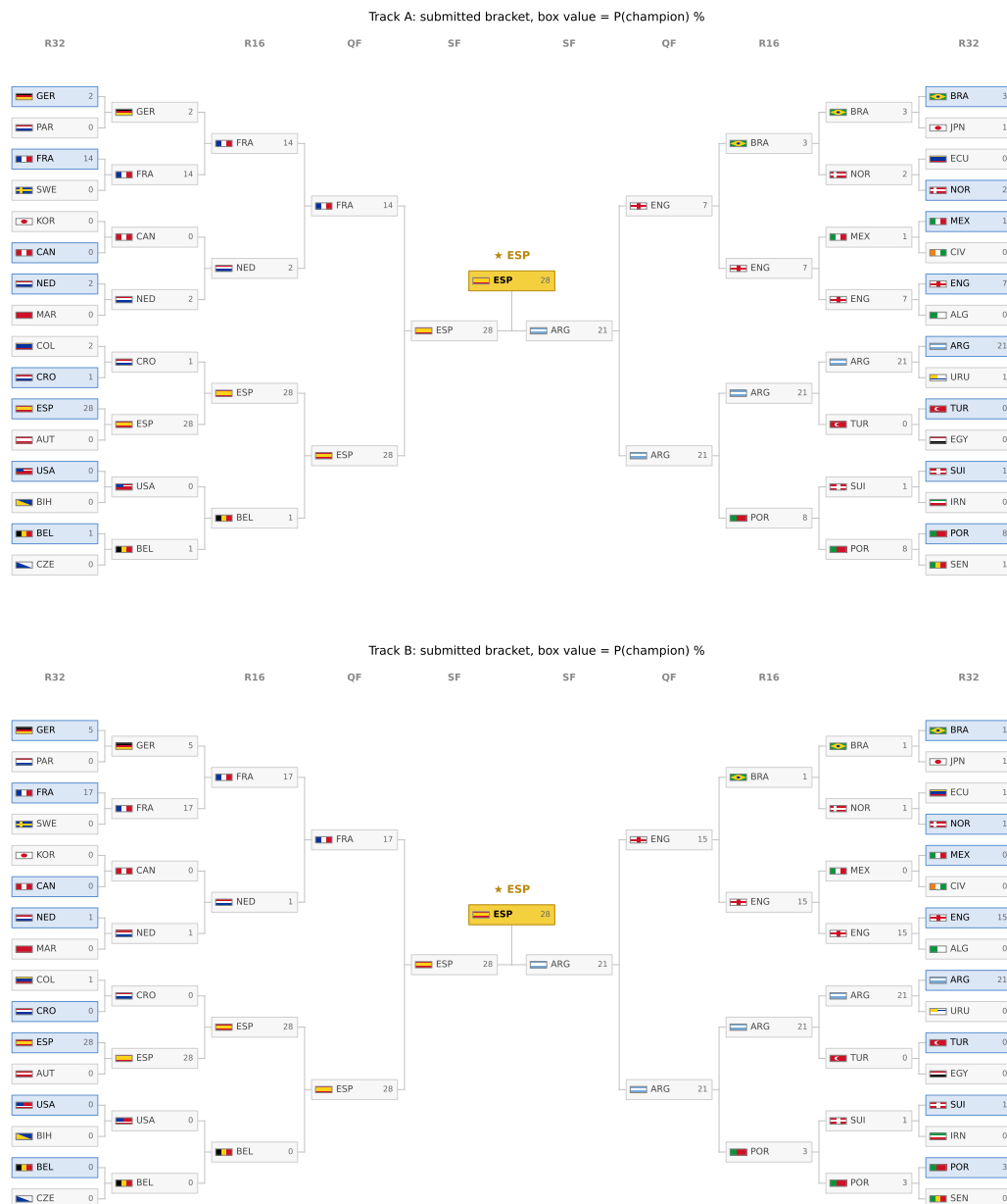
Figure 19: The submitted bracket re-valued by champion probability under Track A (top) and Track B (bottom) at live edition M040; the gold box is each track's most likely champion and greyed boxes are teams eliminated by confirmed results. The locked submitted bracket is Figure 18.
