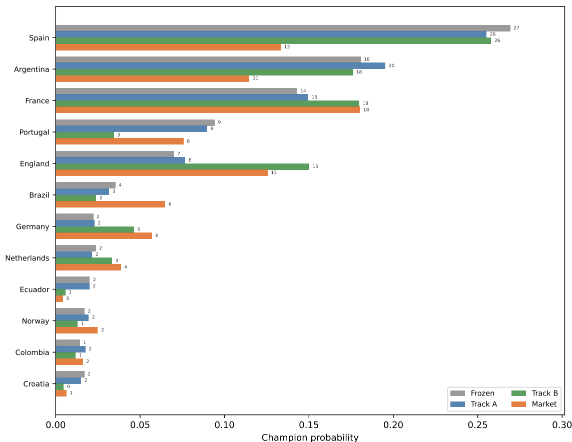
Figure 4: Champion probability, four ways: Frozen / Track A / Track B / Market, top twelve teams (live edition M027)
