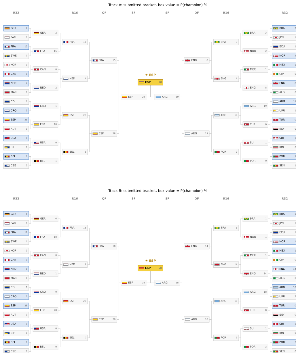
Figure 19: The submitted bracket re-valued by champion probability under Track A (top) and Track B (bottom) at live edition M038; the gold box is each track's most likely champion and greyed boxes are teams eliminated by confirmed results. The locked submitted bracket is Figure 18.
