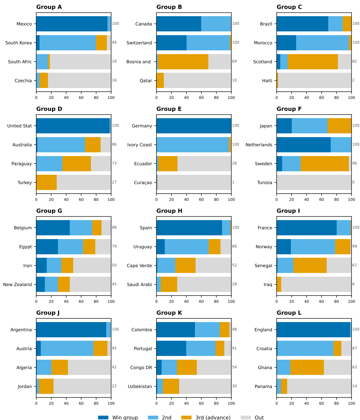
Figure 17: Qualification probability by team — Track B (result-conditioning + live Elo + bookmaker odds; live edition M038)
