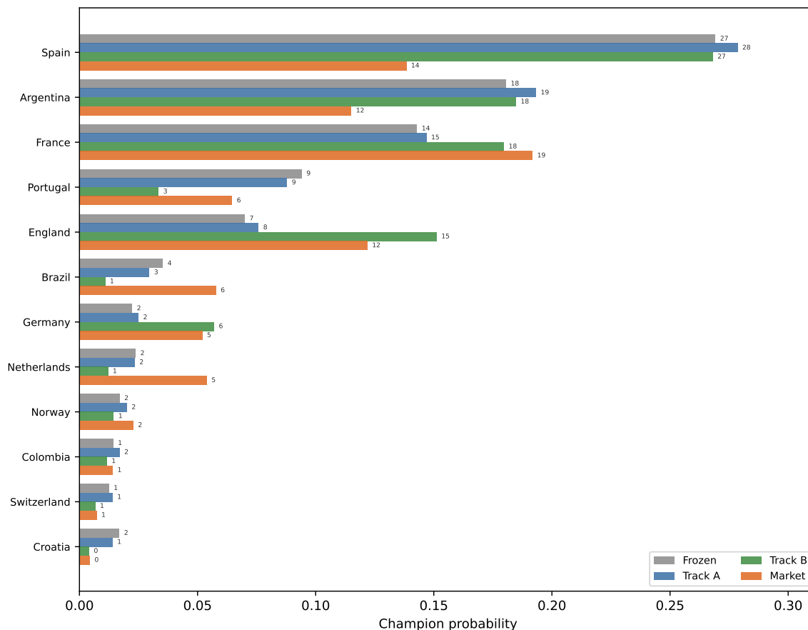
Figure 4: Champion probability, four ways: Frozen / Track A / Track B / Market, top twelve teams (live edition M038)
