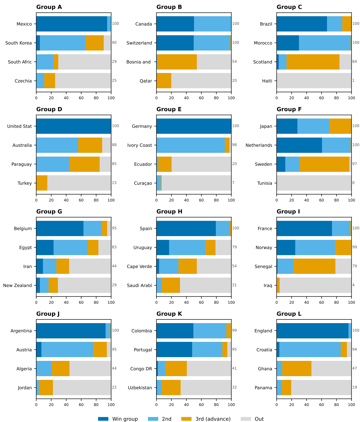
Figure 16: Qualification probability by team — Track A (conditioned on 37 results, June 10 ratings frozen; live edition M038)
