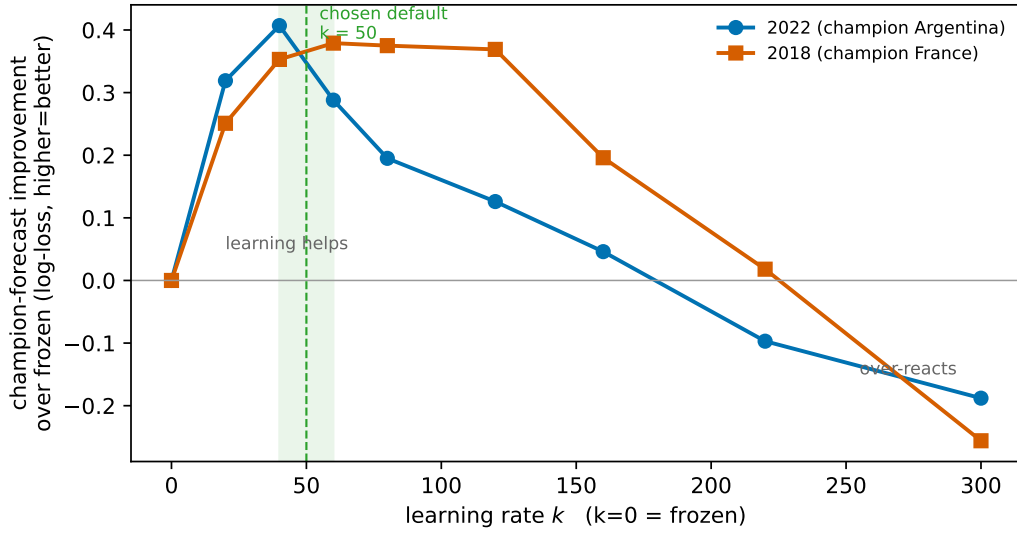
Figure 17: Learning-rate sweep on two World Cups
