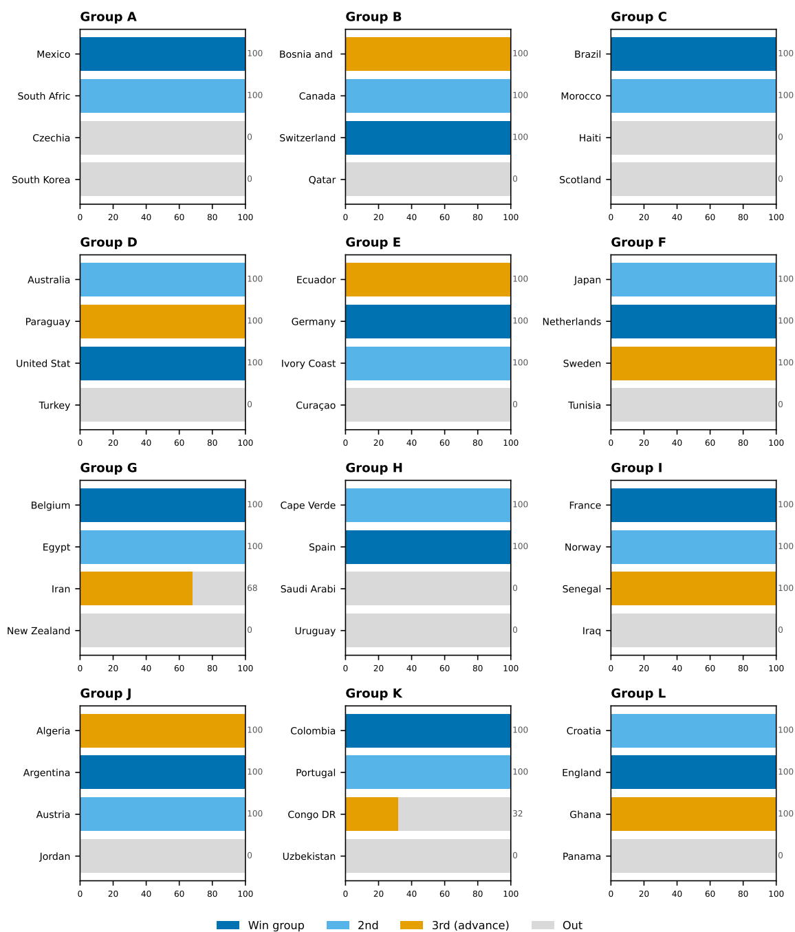
Figure 16: Qualification probability by team — Track A (conditioned on 71 results, June 10 ratings frozen; live edition M071)
