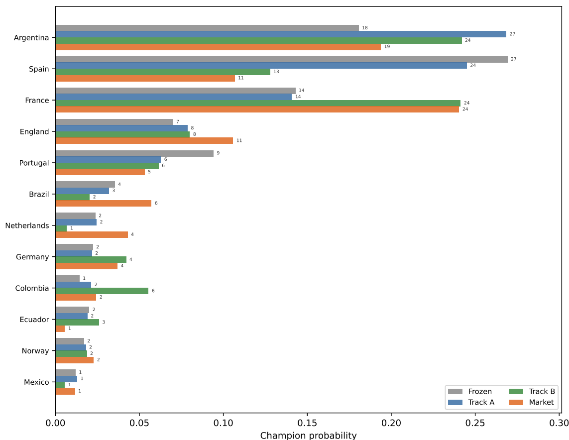
Figure 4: Champion probability, four ways: Frozen / Track A / Track B / Market, top twelve teams (live edition M071)
