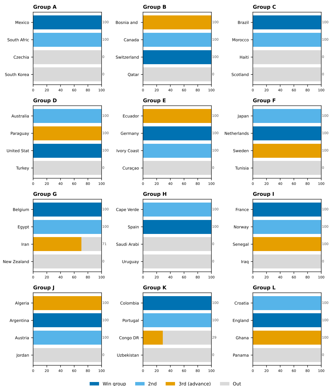
Figure 17: Qualification probability by team — Track B (result-conditioning + live Elo + bookmaker odds; live edition M071)
