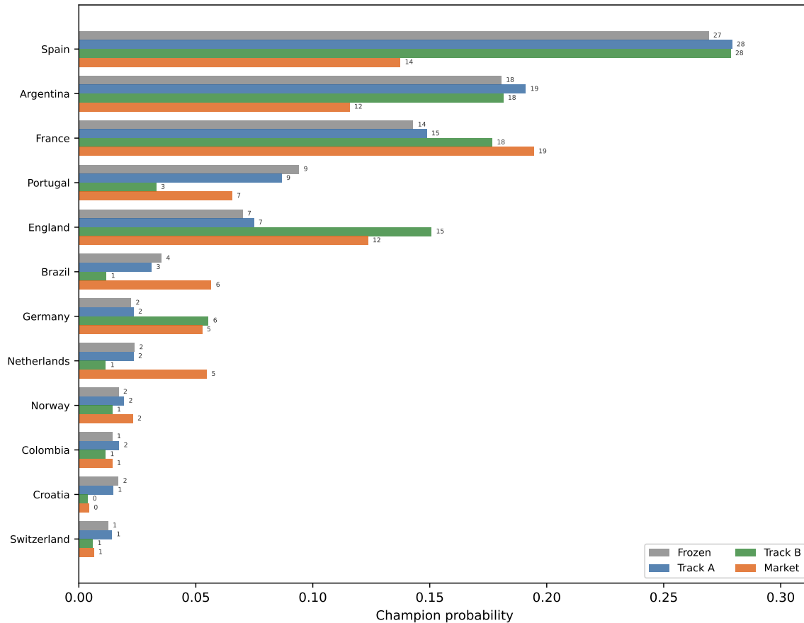
Figure 4: Champion probability, four ways: Frozen / Track A / Track B / Market, top twelve teams (live edition M039)
