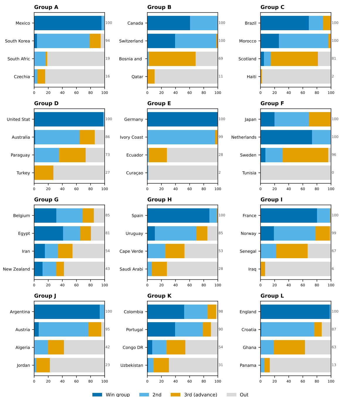
Figure 17: Qualification probability by team — Track B (result-conditioning + live Elo + bookmaker odds; live edition M039)
