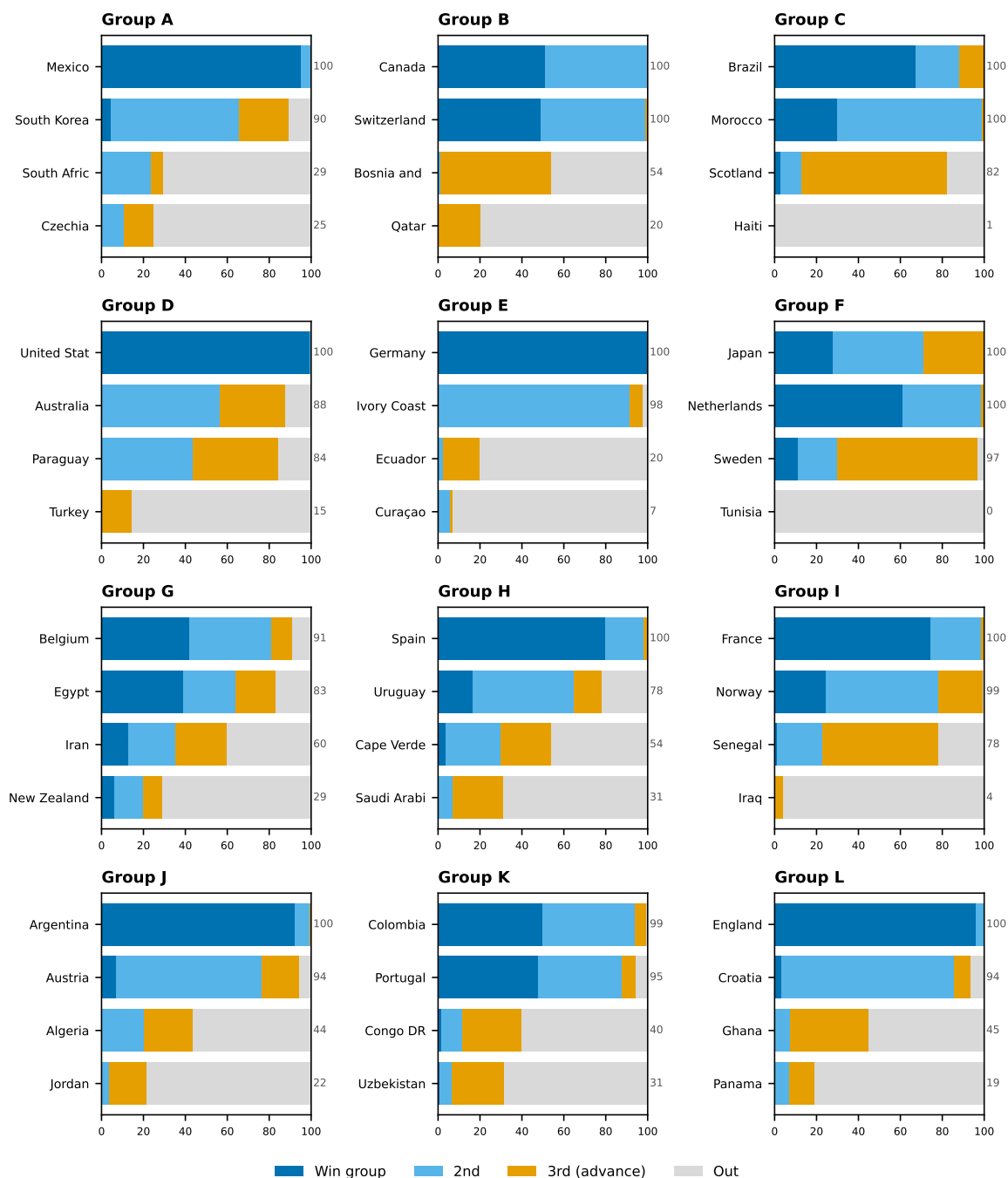
Figure 16: Qualification probability by team — Track A (conditioned on 38 results, June 10 ratings frozen; live edition M039)
