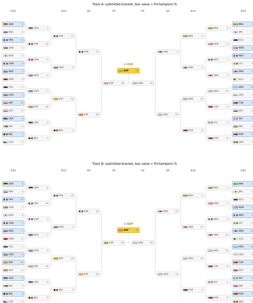
Figure 19: The submitted bracket re-valued by champion probability under Track A (top) and Track B (bottom) at live edition M039; the gold box is each track's most likely champion and greyed boxes are teams eliminated by confirmed results. The locked submitted bracket is Figure 18.
